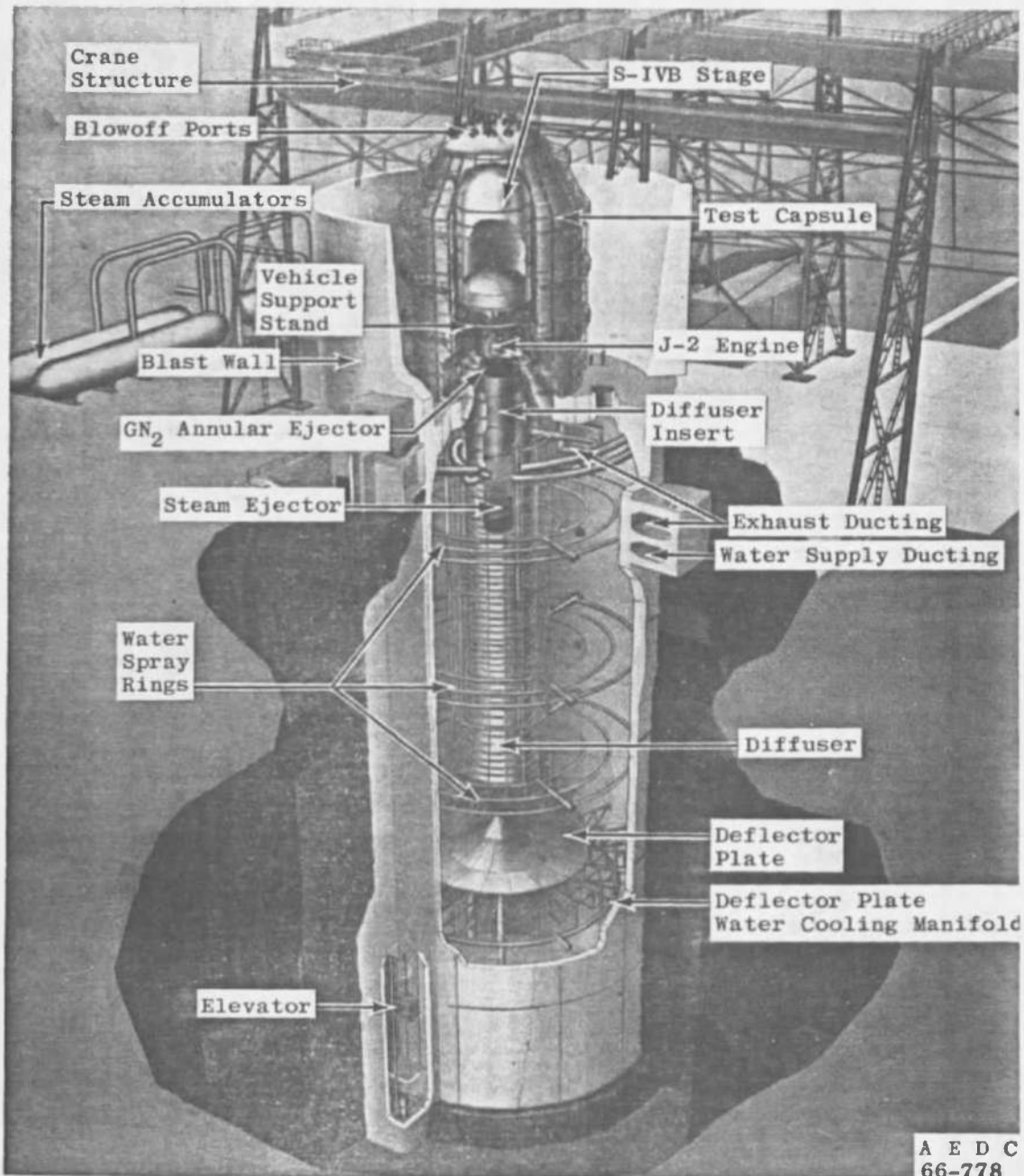
Fig. 12 Propulsion Engine Test Cell (J-4) Details
