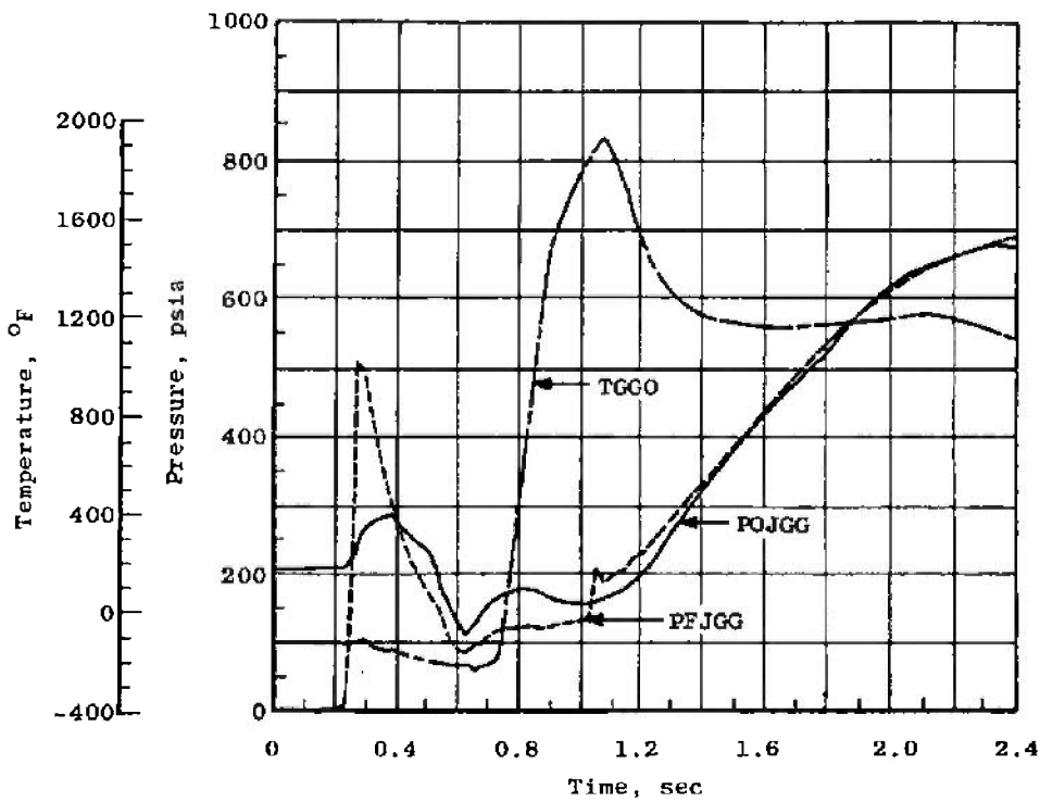
b. Gas Generator Start Transient - Test 24C
