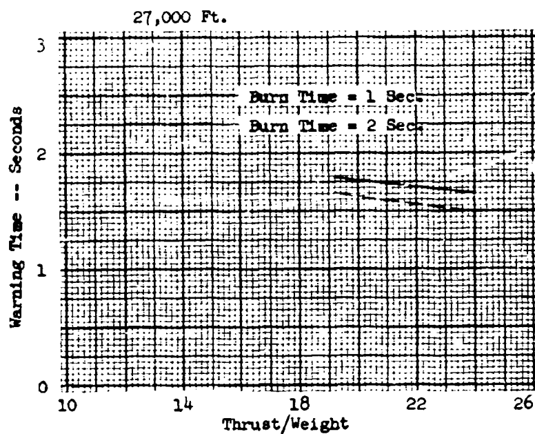
Fig. 75 Minimum Explosion Warning Time Required for a Typical HTOL Vehicle
