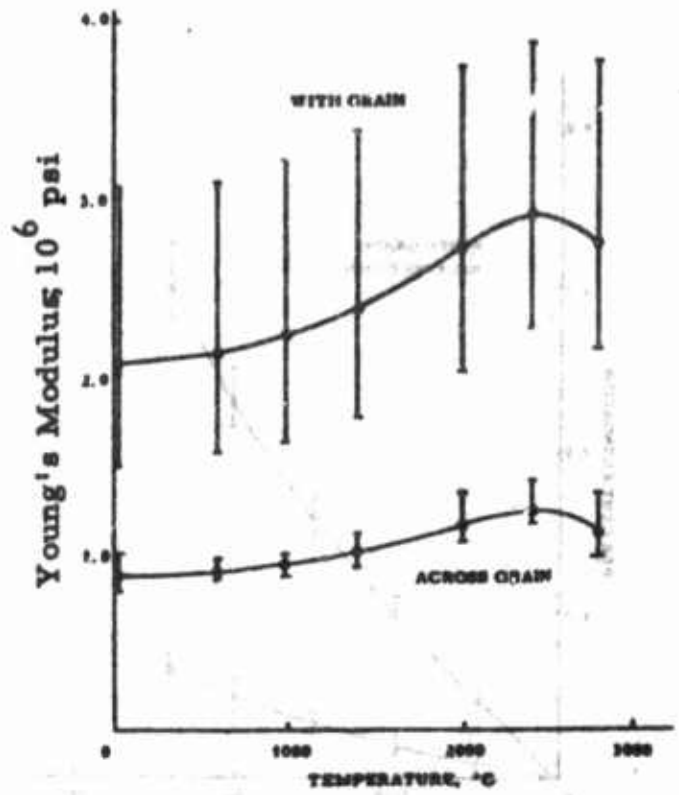
Young's Modulus vs. Temperature, ZTA Graphite, 8-1/2" x 11"
