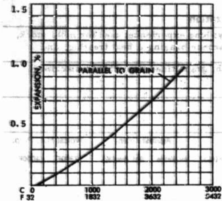
Thermal Expansion vs. Temperature Grade 3499S
