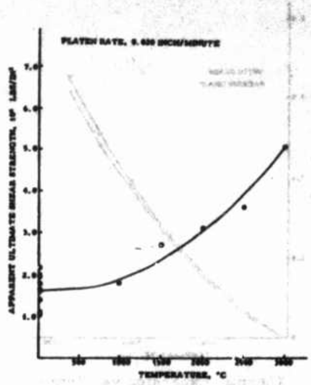
With-Grain Apparent Ultimate Shear Strength vs. Temperature, CFW Graphite, 40" O. D. x 15" L. D. x 20"
