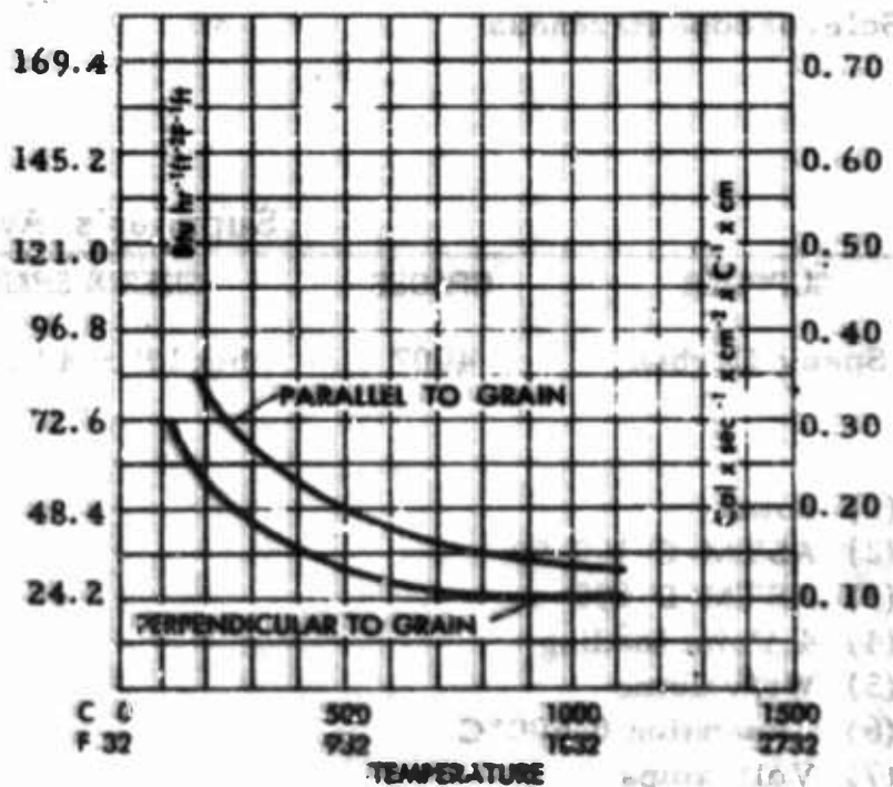
Thermal Conductivity - Grade 3499S
