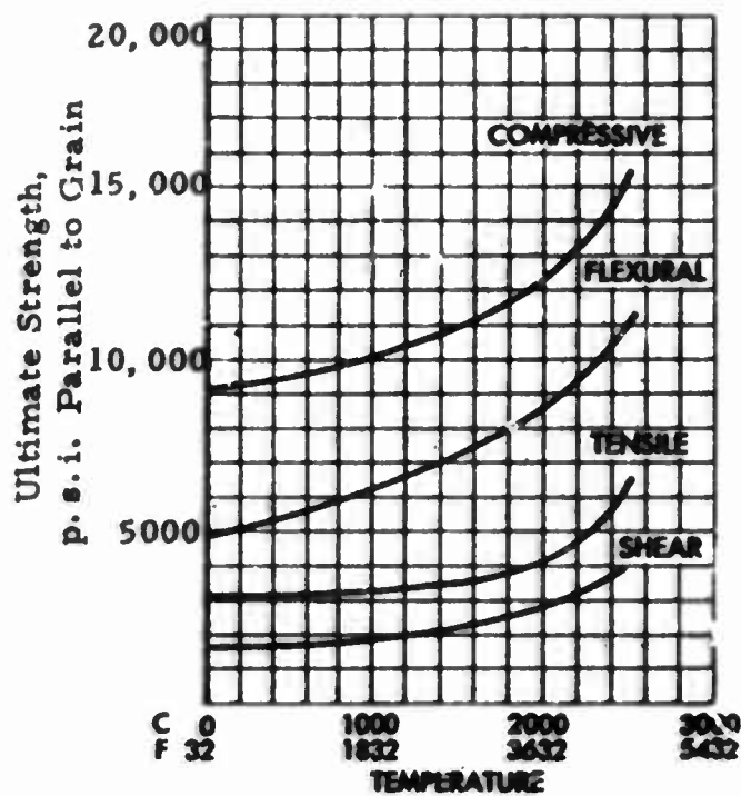
Ultimate Strength-Grade 9134
