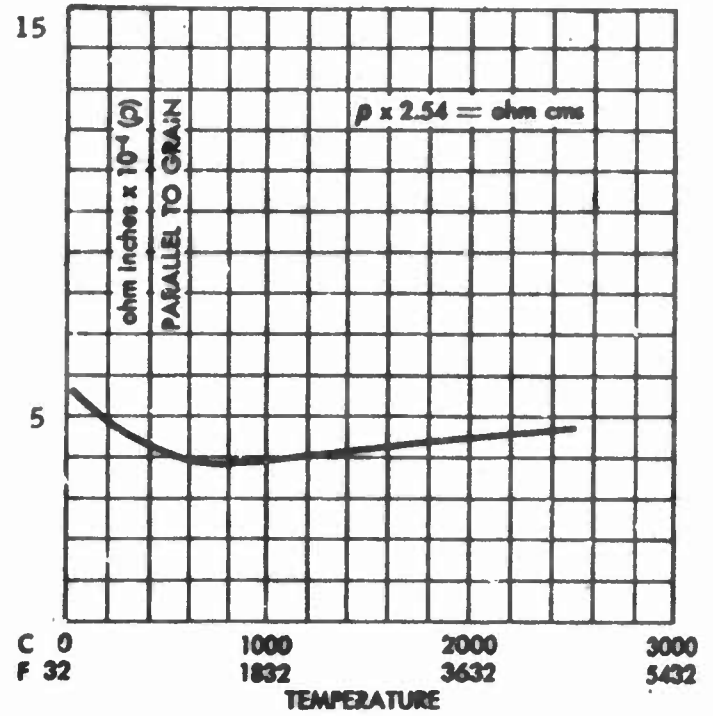
Electrical Resistivity - Grade 580
