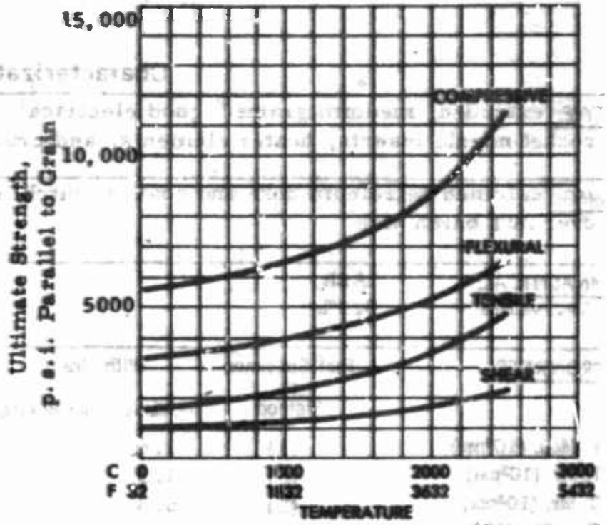
Ultimate Strength vs. Temperature Grade 873S
