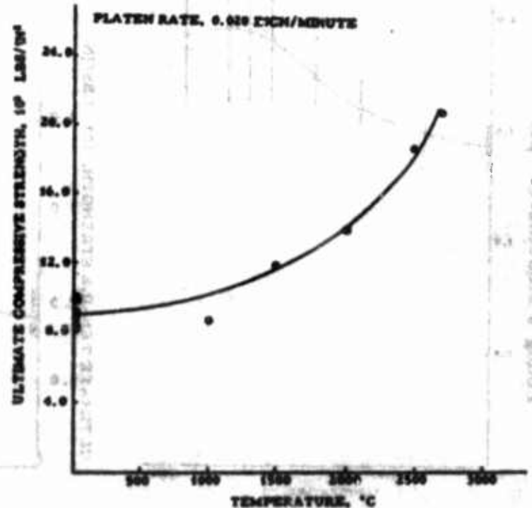
With-Grain Ultimate Compressive Strength vs. Temperature, CFW Graphite, 40" O. D. x 15" L. D. x 20"
