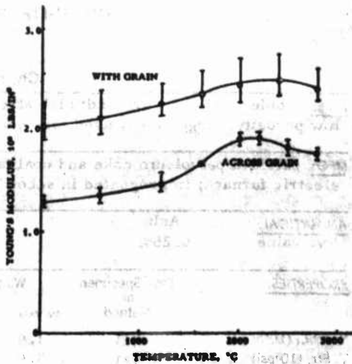
Young's Modulus vs. Temperature, CFZ Graphite, 14" dia. x 13-1/2"
