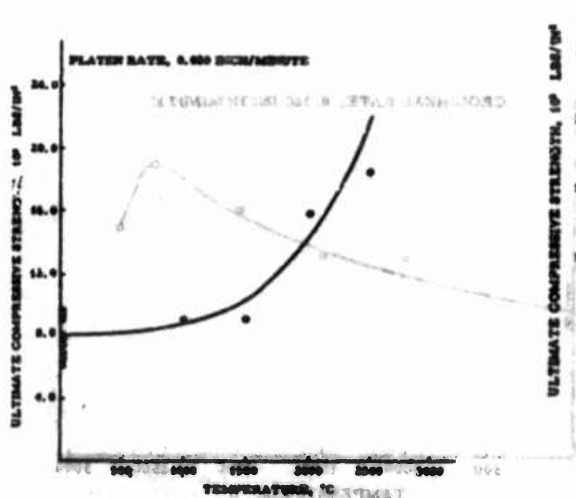
Across-Grain Ultimate Compressive Strength vs. Temperature, CFW Graphite, 40" O. D. x 15" L. D. x 20"
