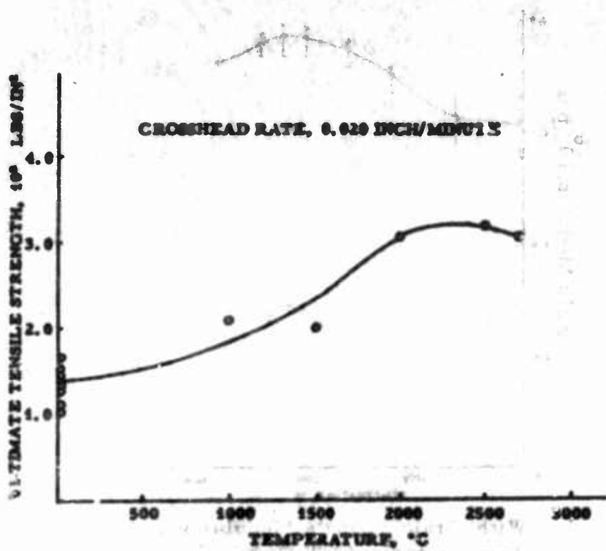
Across-Grain Ultimate Tensile Strength vs. Temperature, CFW Graphite, 40" O. D. x 15" L. D. x 20"
