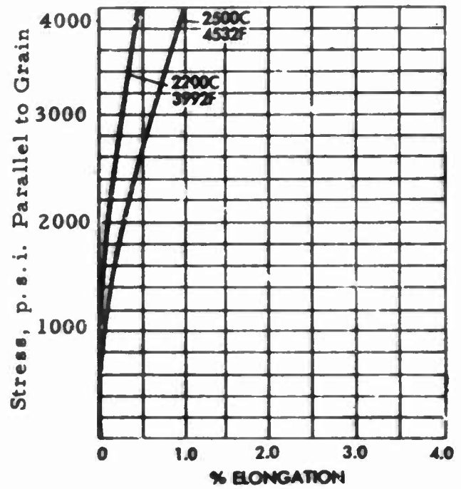
Tensile Stress-Strain Curves at Various Temperatures Grade 9134
