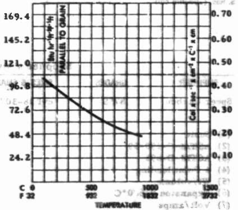
Thermal Conductivity - Grade 873S
