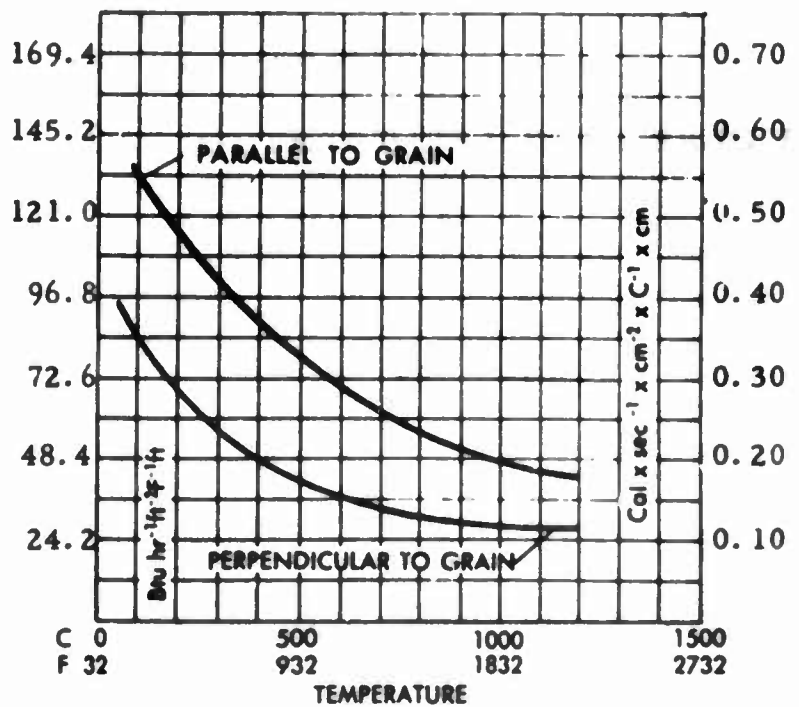
Thermal Conductivity - Grade 8882
