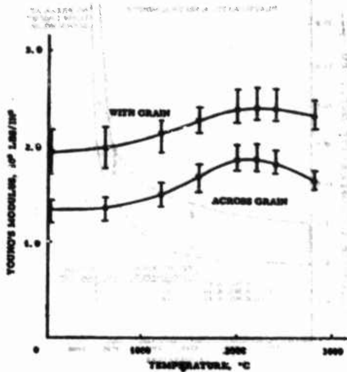
Young's Modulus vs. Temperature, RVA Graphite, 33" dia. x 42"
