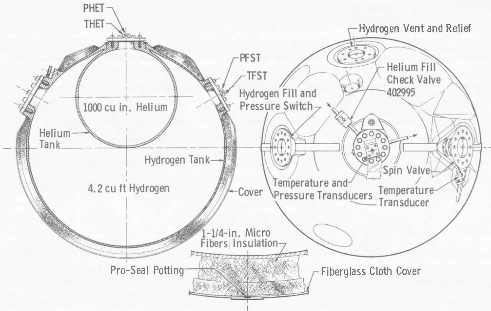
a. Start Tank and Helium Tank Fig. III-1 Instrument Locations
