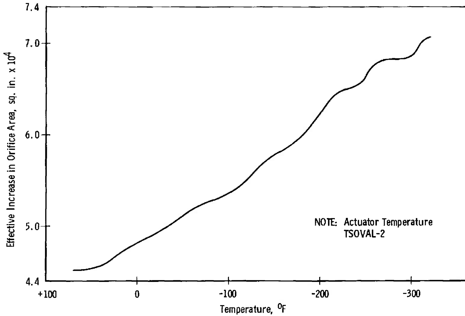
Fig. 12 Thermostatic Orifice Characteristics
