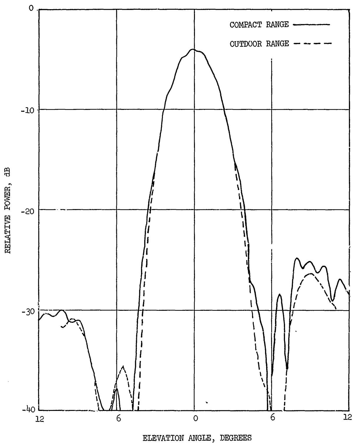
Figure 22. Comparison of the elevation patterns recorded on the outdoor range and on the modified line-source compact range at 10 GHz.
