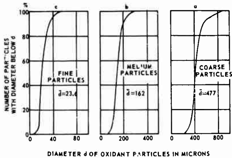
Figure 5. Particulate Distribution of Oxidant
