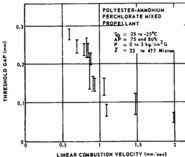
Figure 10. Effects of Linear Combustion Velocity on Flame Propagation into Cracks
