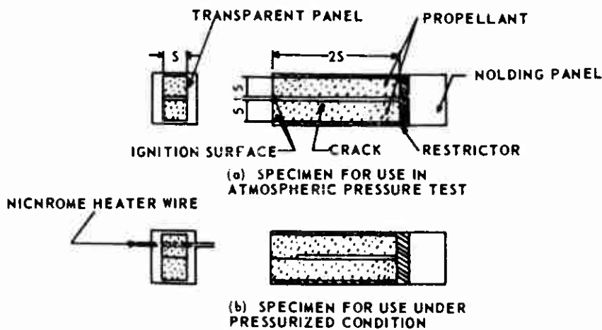
Figure 1. Details of Propellant Test Specimen
