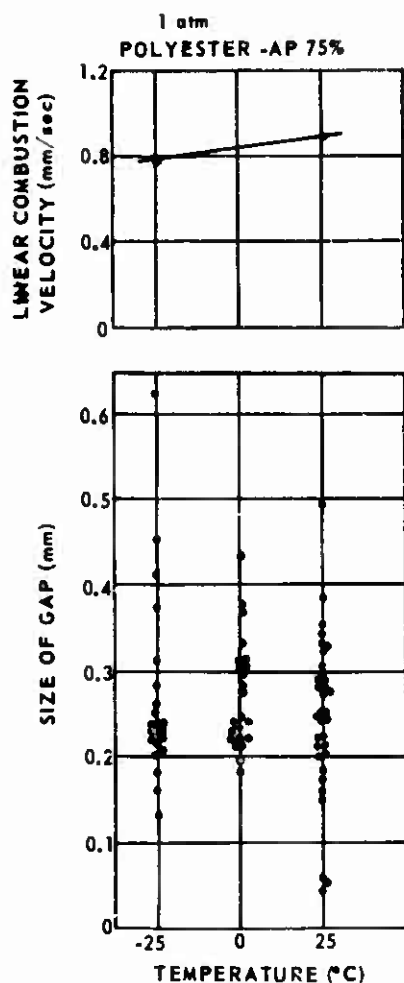
Figure 6. Effects of Propellant Initial Temperature on Flame Propagation into Cracks
