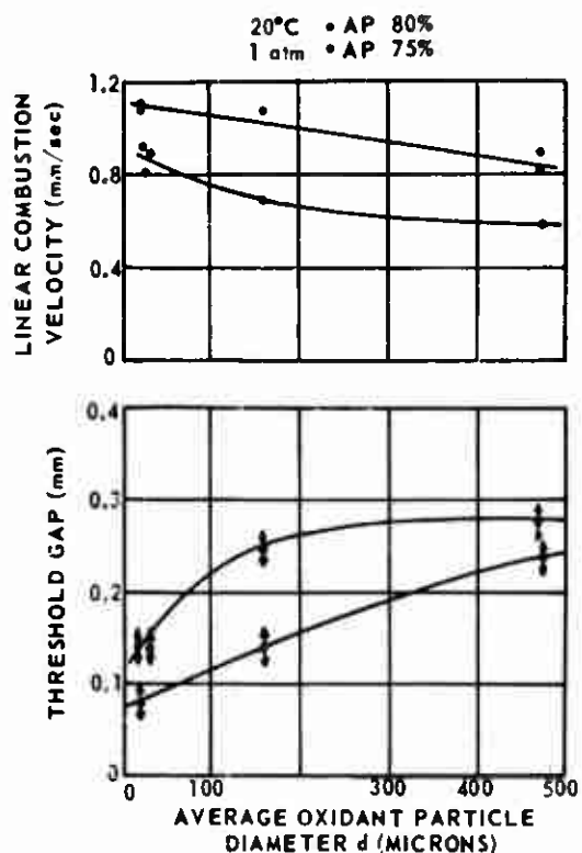
Figure 9. Effects on Flame Propagation into Cracks of Oxidant's Particulate Distribution and Content
