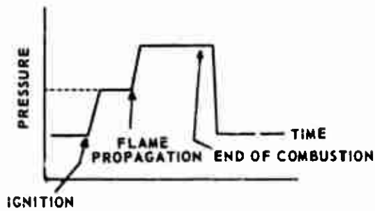
Figure 3. Change in Pressure within the Chamber with Passage of Time when the Flame Propagated into Cracks
