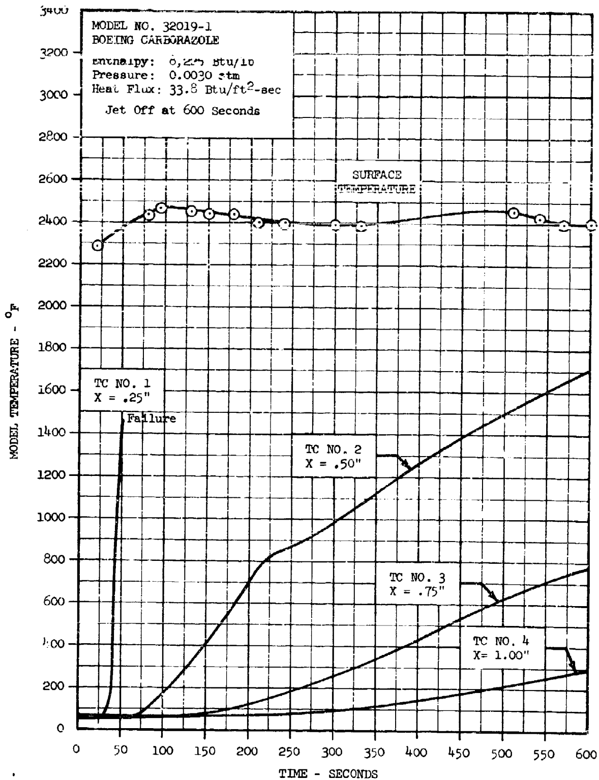
Figure 13 -- Boeing Carborazole Model 32019-1 Temperature History
