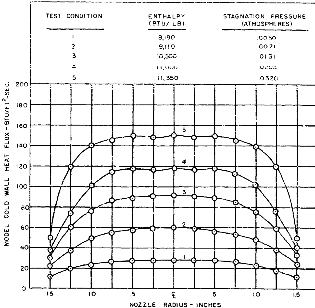
Heat Flux Surveys of 3-inch Stream
