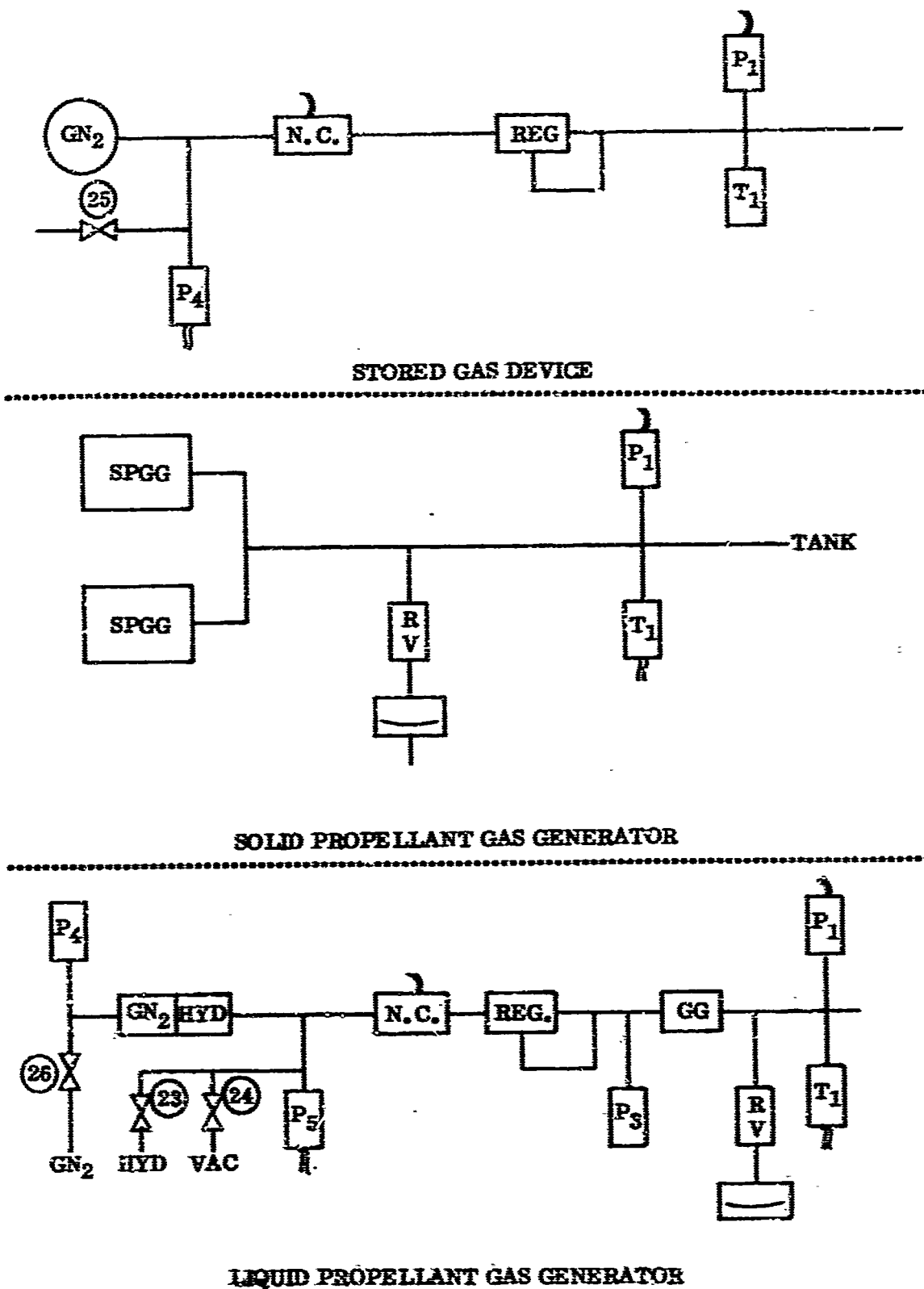
Figure 52. Pressurization Subsystem Test Schematic
