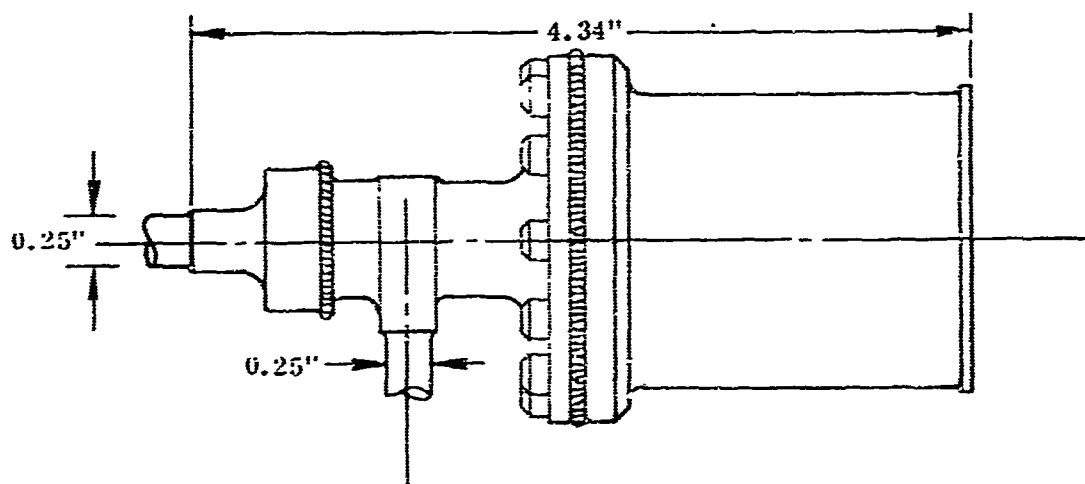
Figure 43. Pressure Regulator
