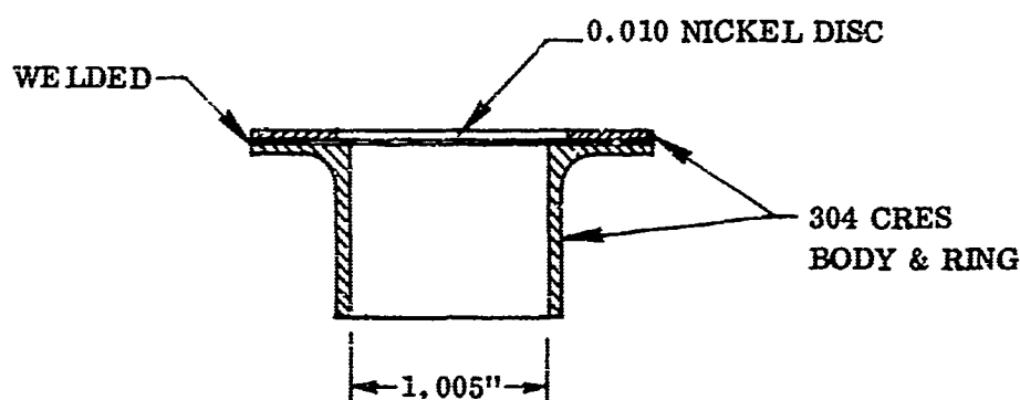
Figure 25. Rupture Disc Relief Valve Outlet
