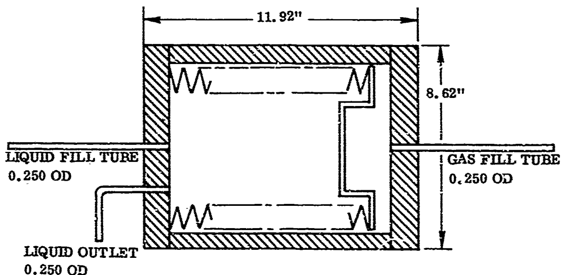
Figure 21. Gas/Hydrazine Tank
