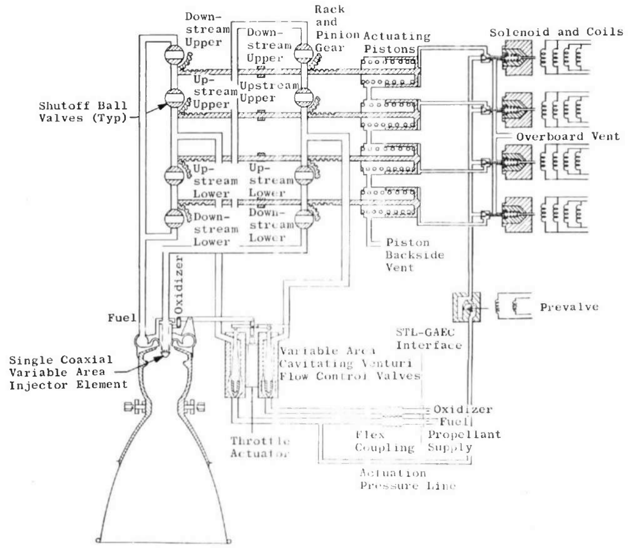
Fig. 6 Schematic of the Thrust Control System
