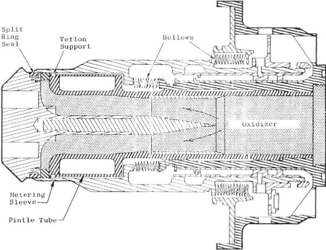
b. Pintle Schematic Fig. 7 Concluded
