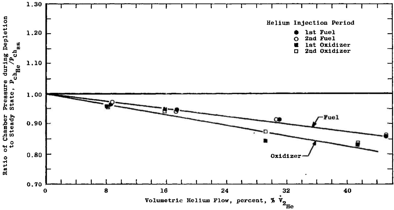
b. Chamber Pressure Fig. 23 Continued
