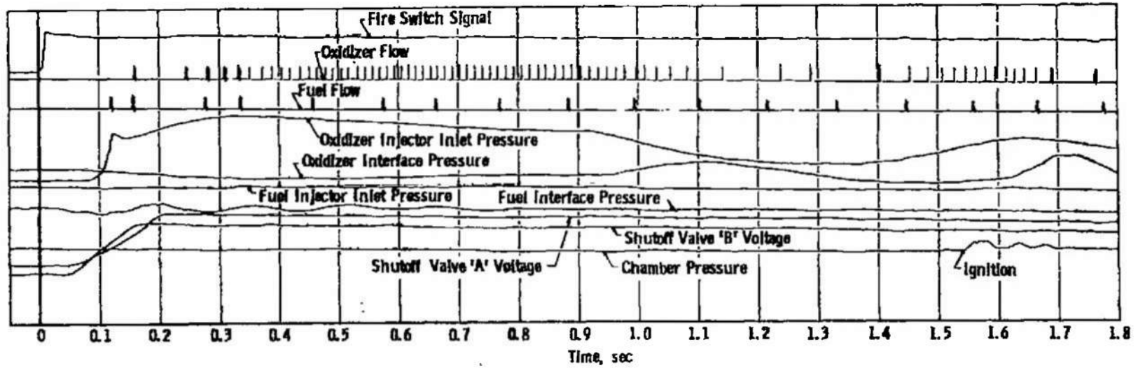
c. Oxidizer System Ingestion (Firing AE-40, Volume = 0.221 ft 3 )
