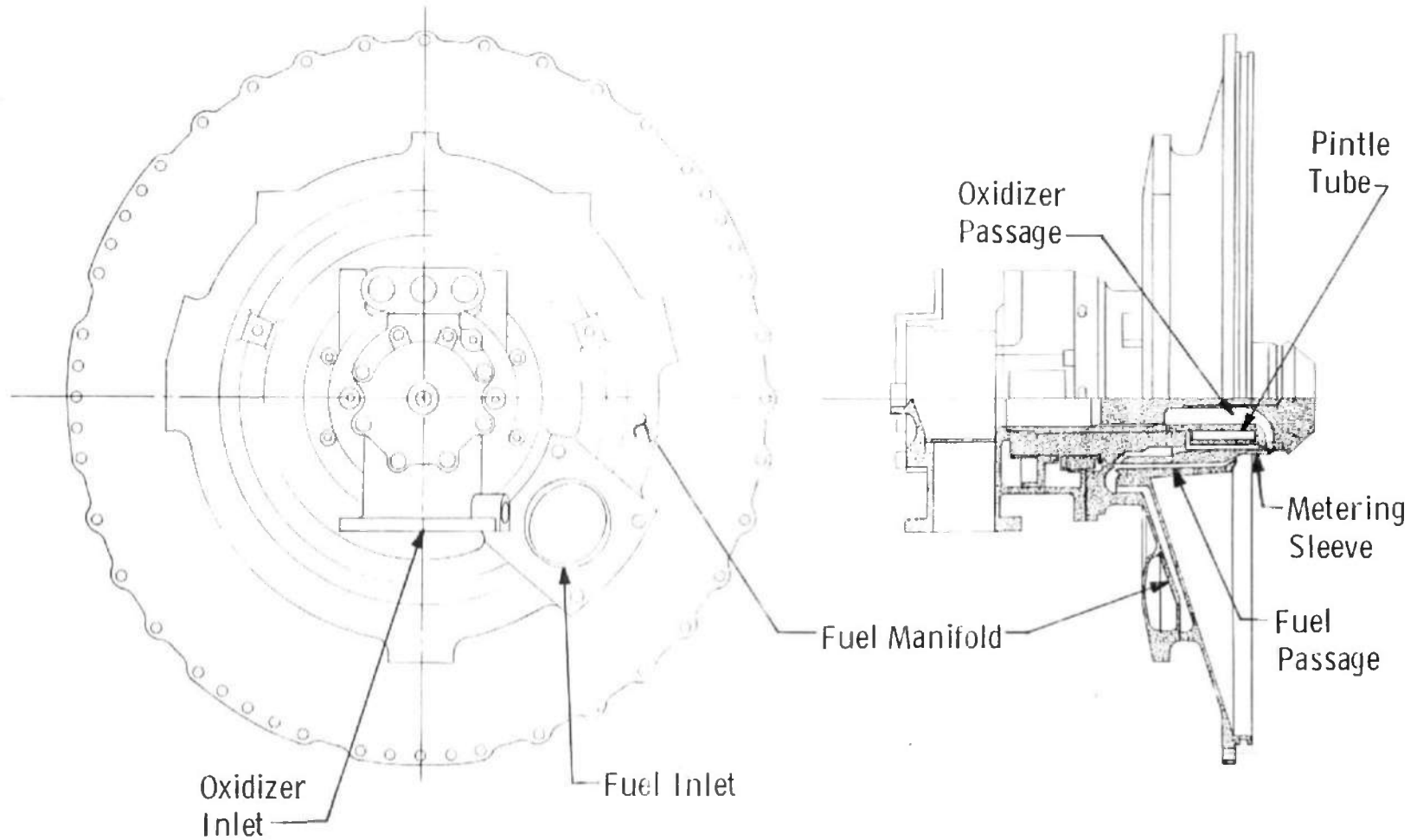
a. Assembly Fig. 7 Propellant Injector
