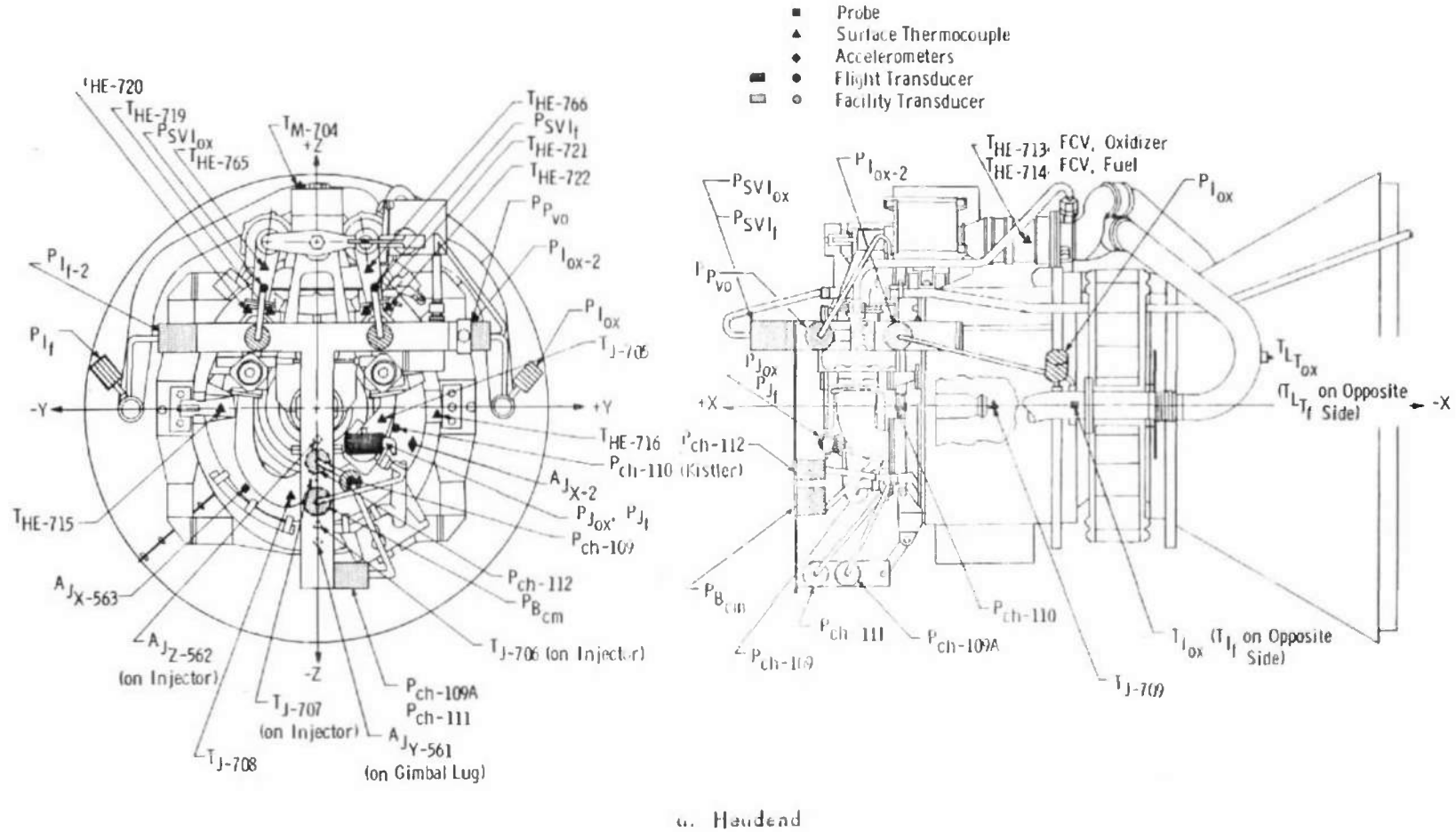
Fig. 12 Engine Instrumentation Locations
