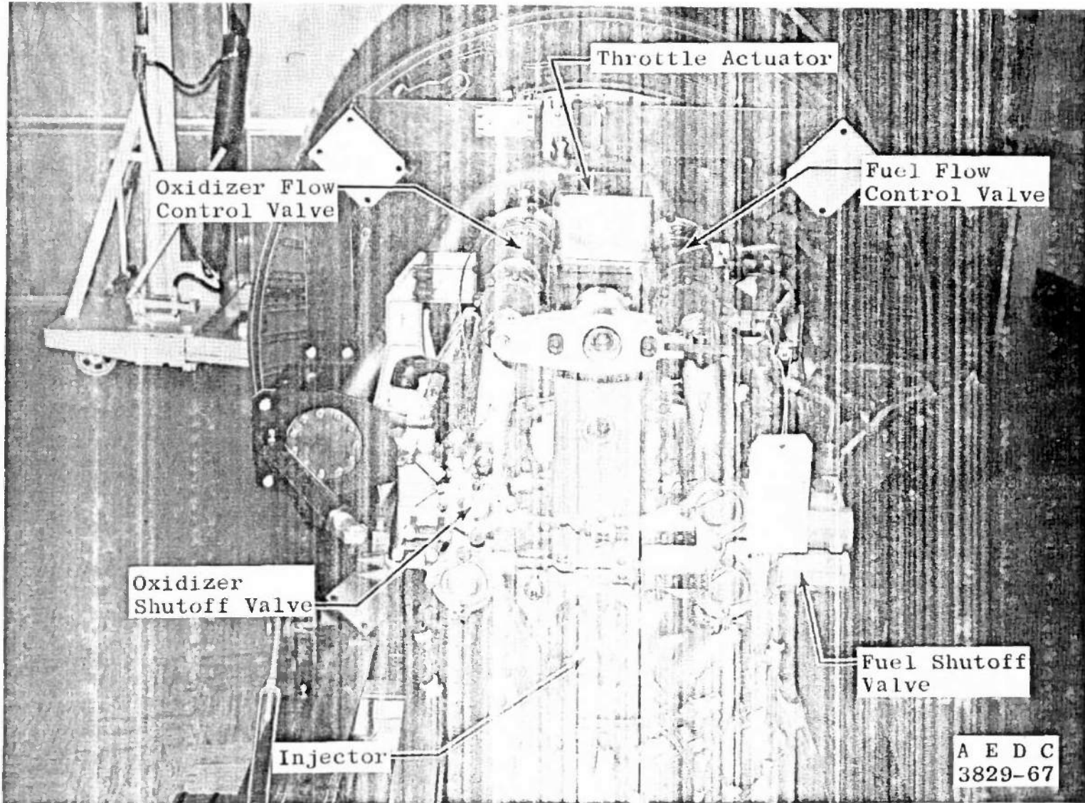
Fig. 5 Thrust Control Assembly
