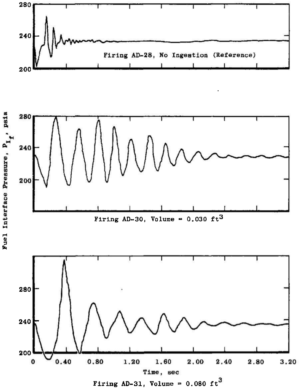
Fig. 15 Fuel Interface Pressure Ignition History
