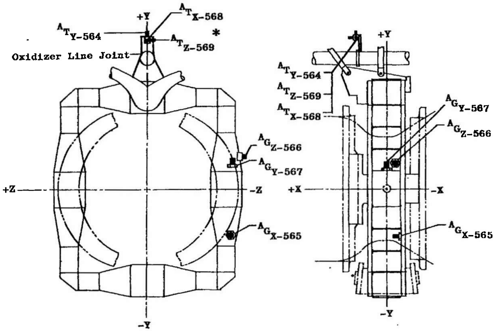
c. Gimbal Assembly Fig. 12 Concluded
