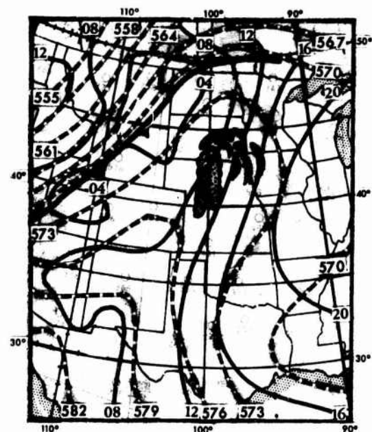
FIGURE 3.—Surface analysis (solid lines) and 1000-500-mb. thickness analysis (dashed lines), 1200 omt June 22, 1966. Stippled area denotes squall-line cloudiness seen in figure 1 and solid shading represents radar echoes observed at 1445 omt.
