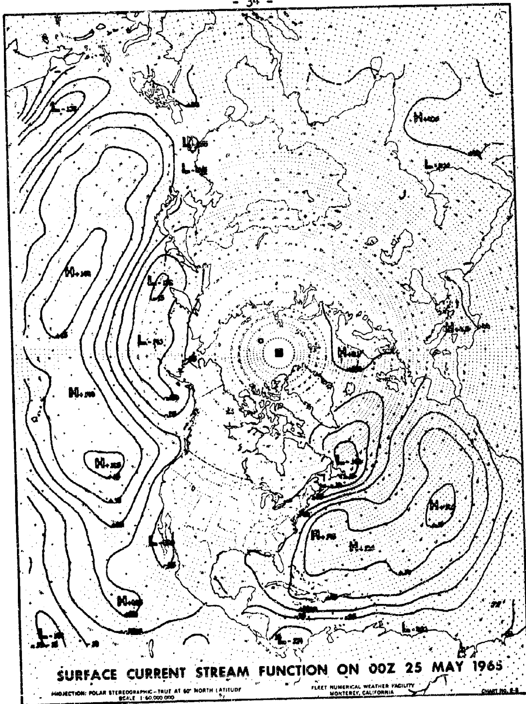
Figure 4.4 Surface Current Stream Function on 00Z 25 May 1965
