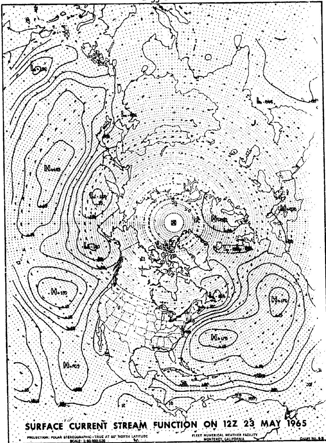
Figure 4.8 Surface Current Stream Function on 12Z 23 May 1965
