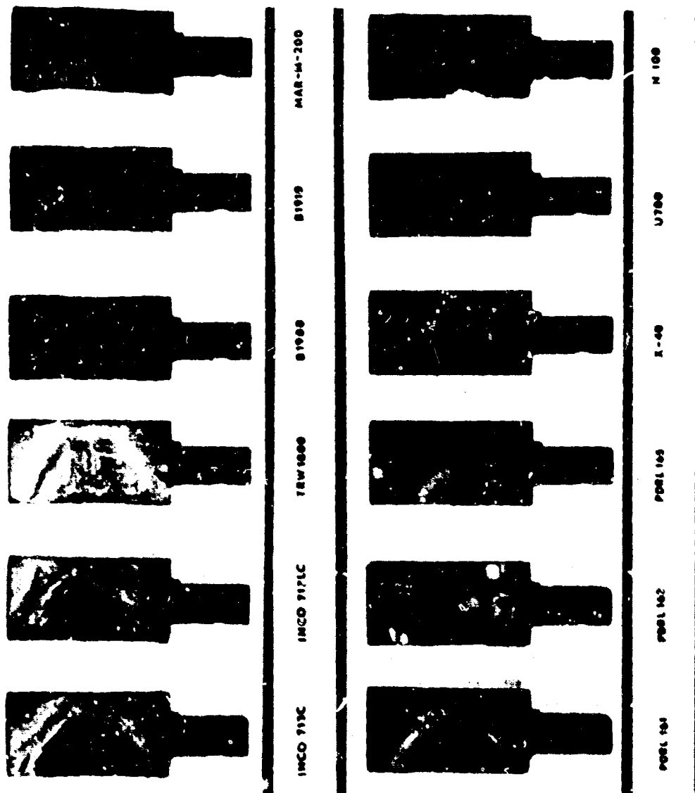
Figure 14. General Appearance of Specimens Tested 120 Hours at 1600°C F Using JP-4R Fuel and an 8 ppm Salt/Air Ratio (Test S-530).
