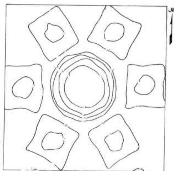
SPECTRAL WINDOW
