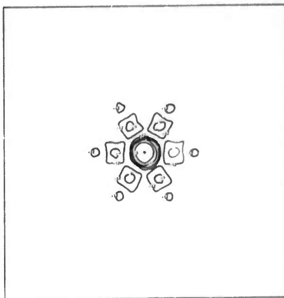
SPECTRAL WINDOW
