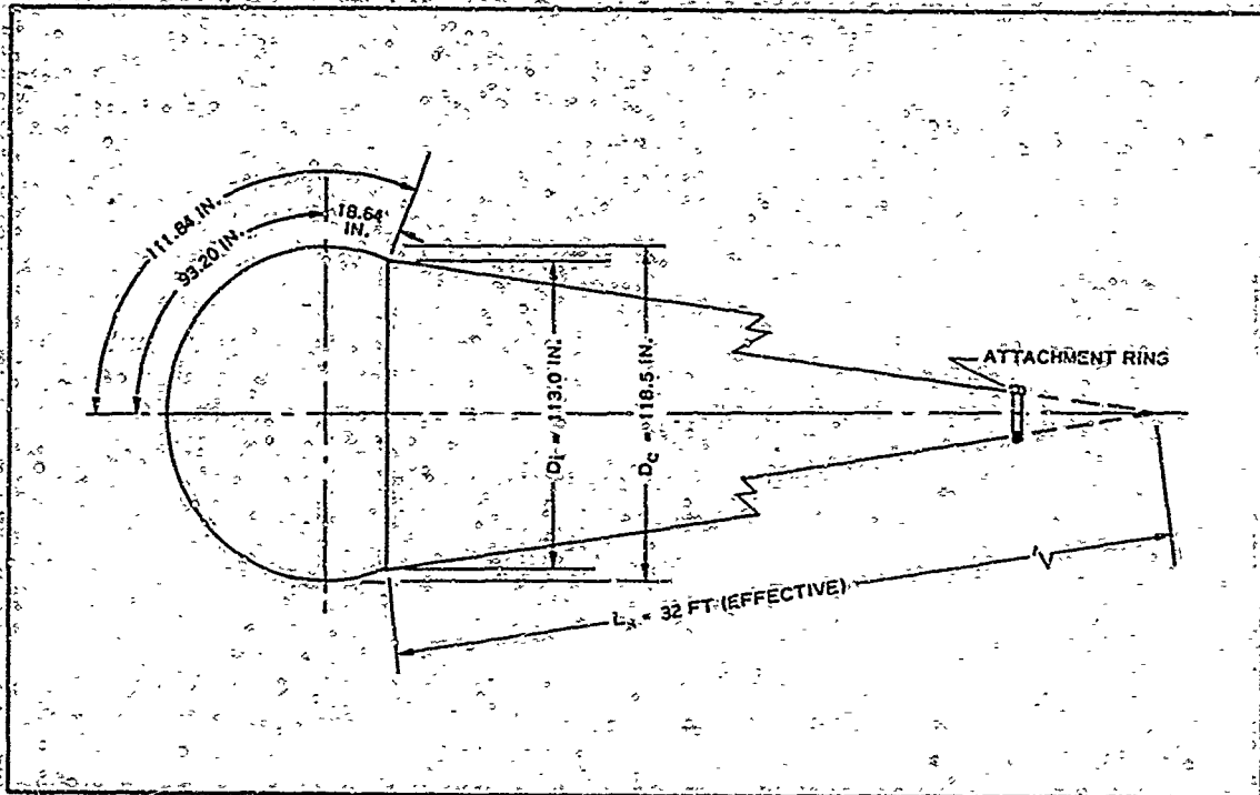
Figure 15 - Sixteen-Foot D Hemisflo Profile Dimensions
