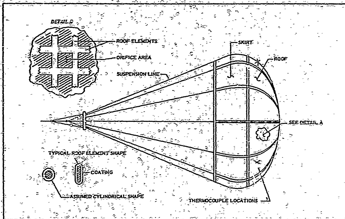
Figure 35 - Schematic of PARASONIC Test Parachute
