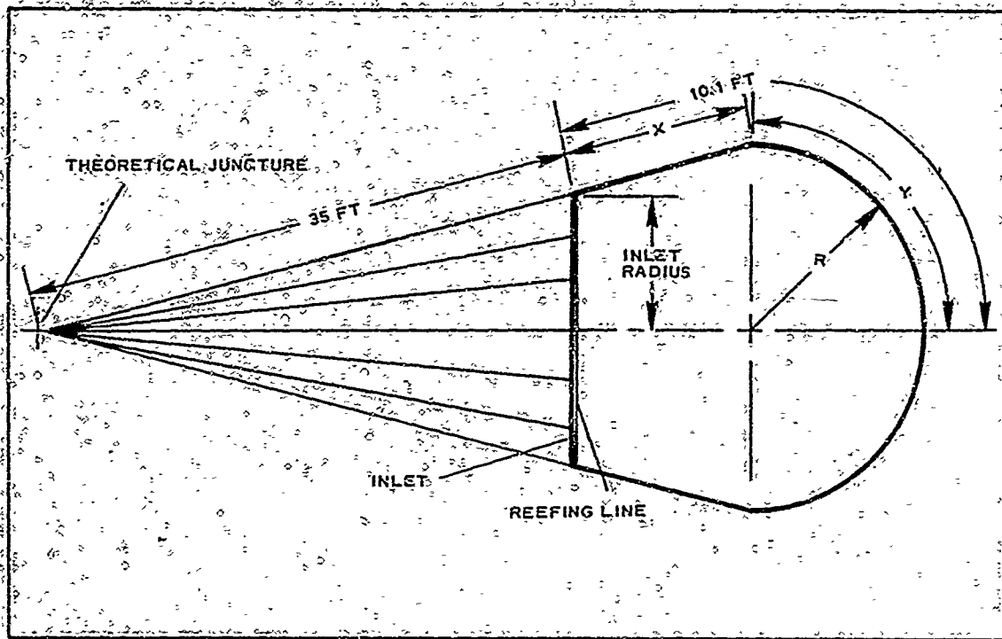
Figure 14 - Geometric Nomenclature
