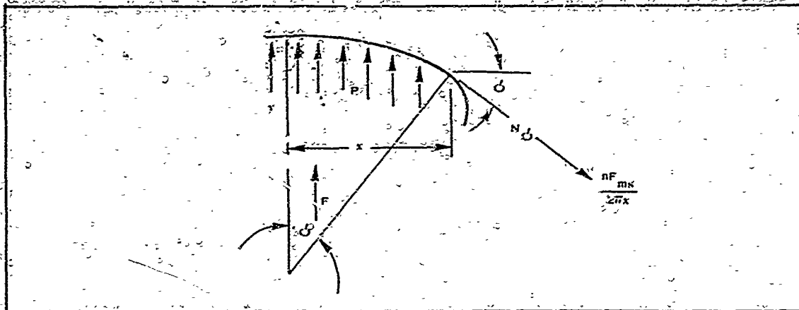
Figure 33 - Structural Load Definitions
