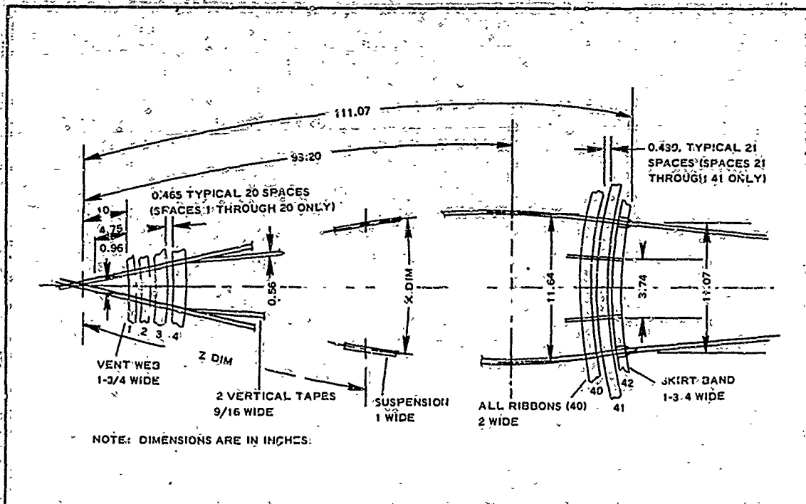
Figure 15 - Sixteen-Foot D Hemisflo Profile Dimensions
