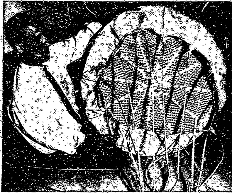
Figure 32 - PARASONIC Parachute with Coated Mesh Roof
