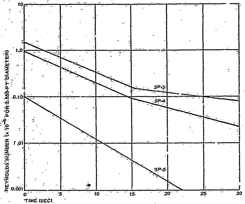
(C) REYNOLDS NUMBER VERSUS TIME
