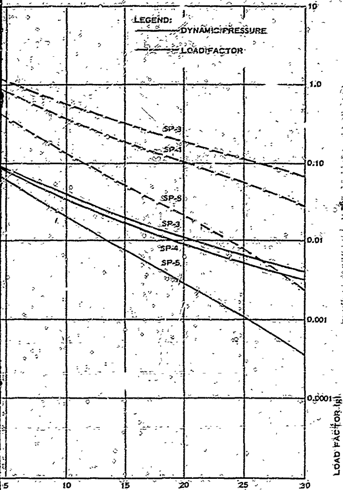
(A) PRESSURE AND LOAD FACTOR VERSUS TIME
