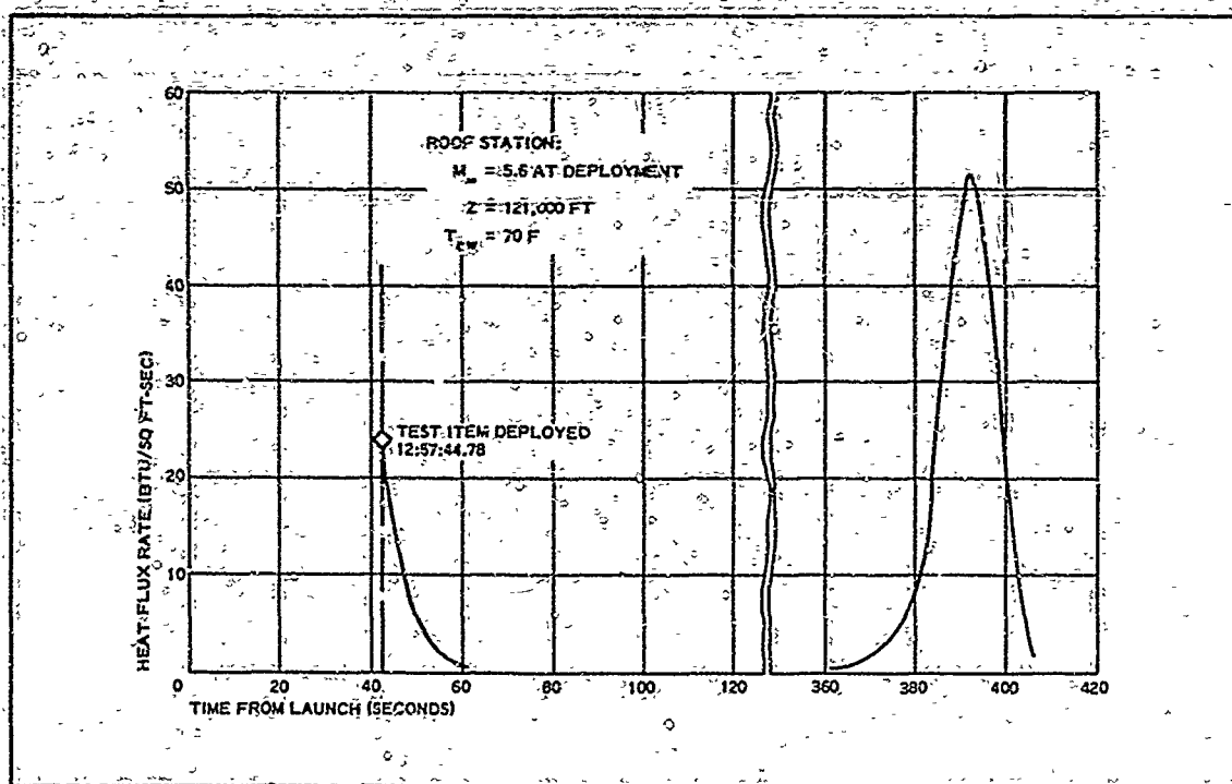
Figure 36 - Calculated Gold Wall Heat Flux Rates
