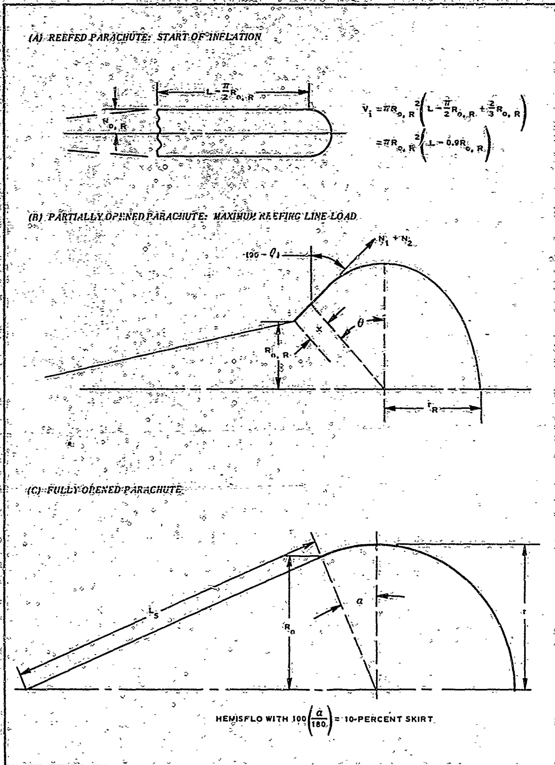
Figure 42 - Reefed, Partially Opened, and Fully Opened Large Parachute
