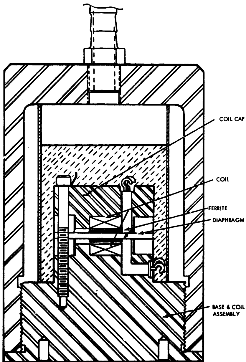
Figure 35. Cross-section of a typical SRI-FMX accelerometer.
