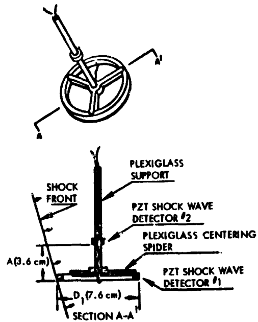
Figure 31. Sandia shock-wave detector.
