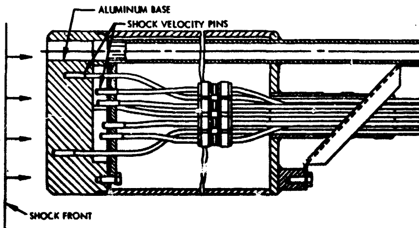
Figure 32. UCRL pin gage.
