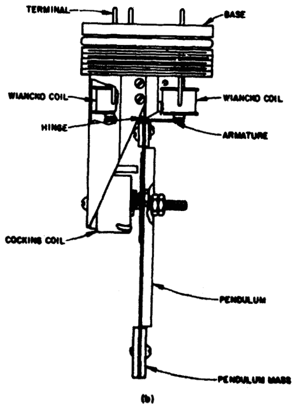
Figure 42. Horizontal and vertical Mark II velocity gage.
