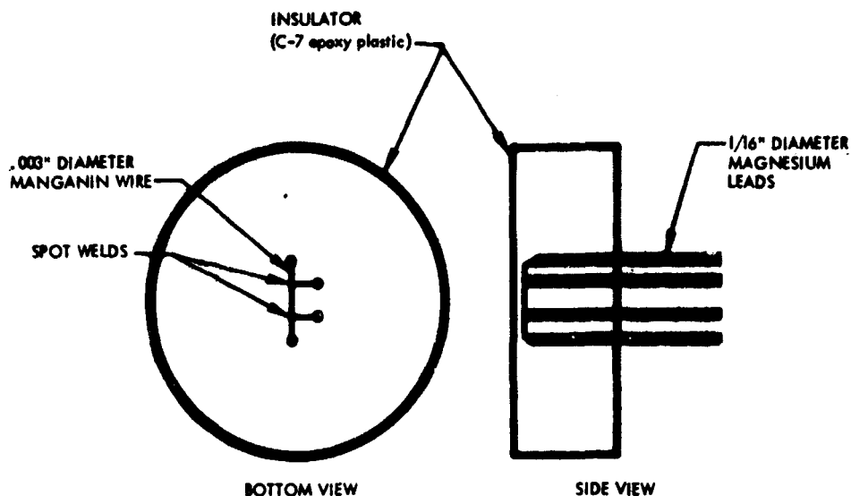
Figure 26. Configuration of SRI manganin gage in C-7 epoxy gage.
