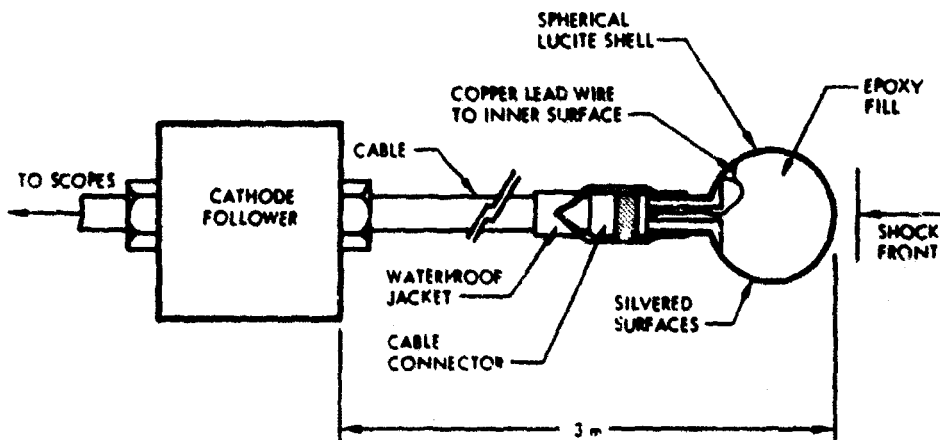
Figure 30. UCRL peak-pressure plastic gage.
