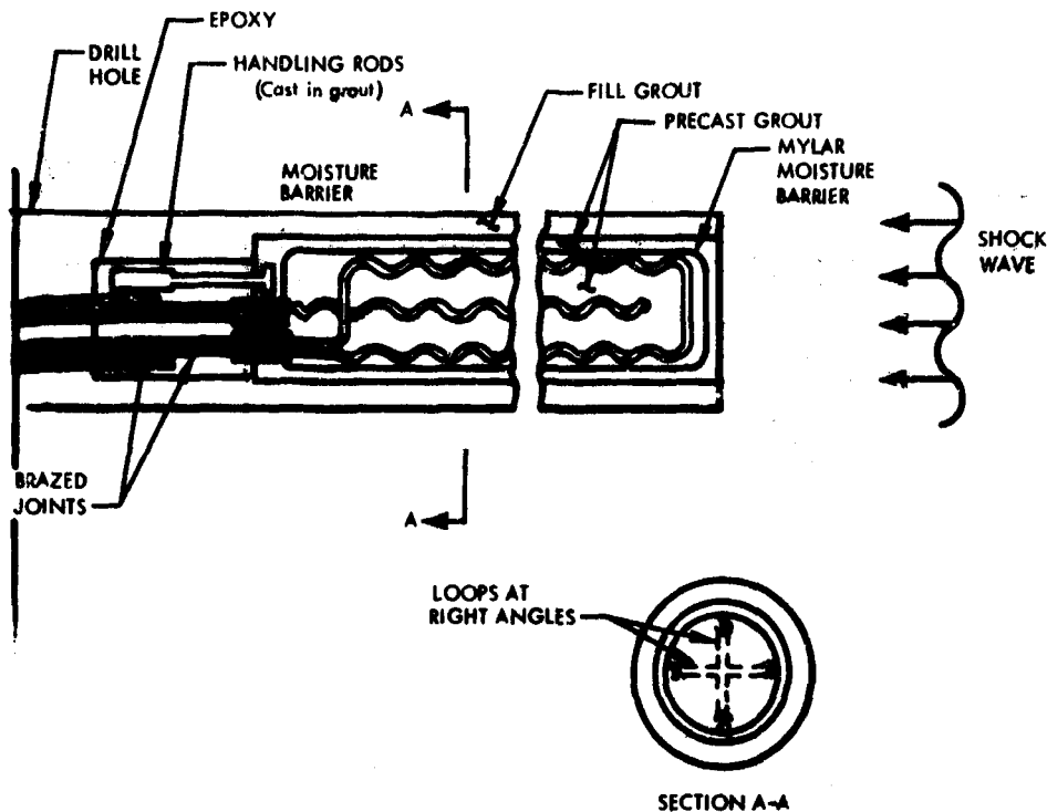
Figure 33. EPCO Faraday induction velocimeter.
