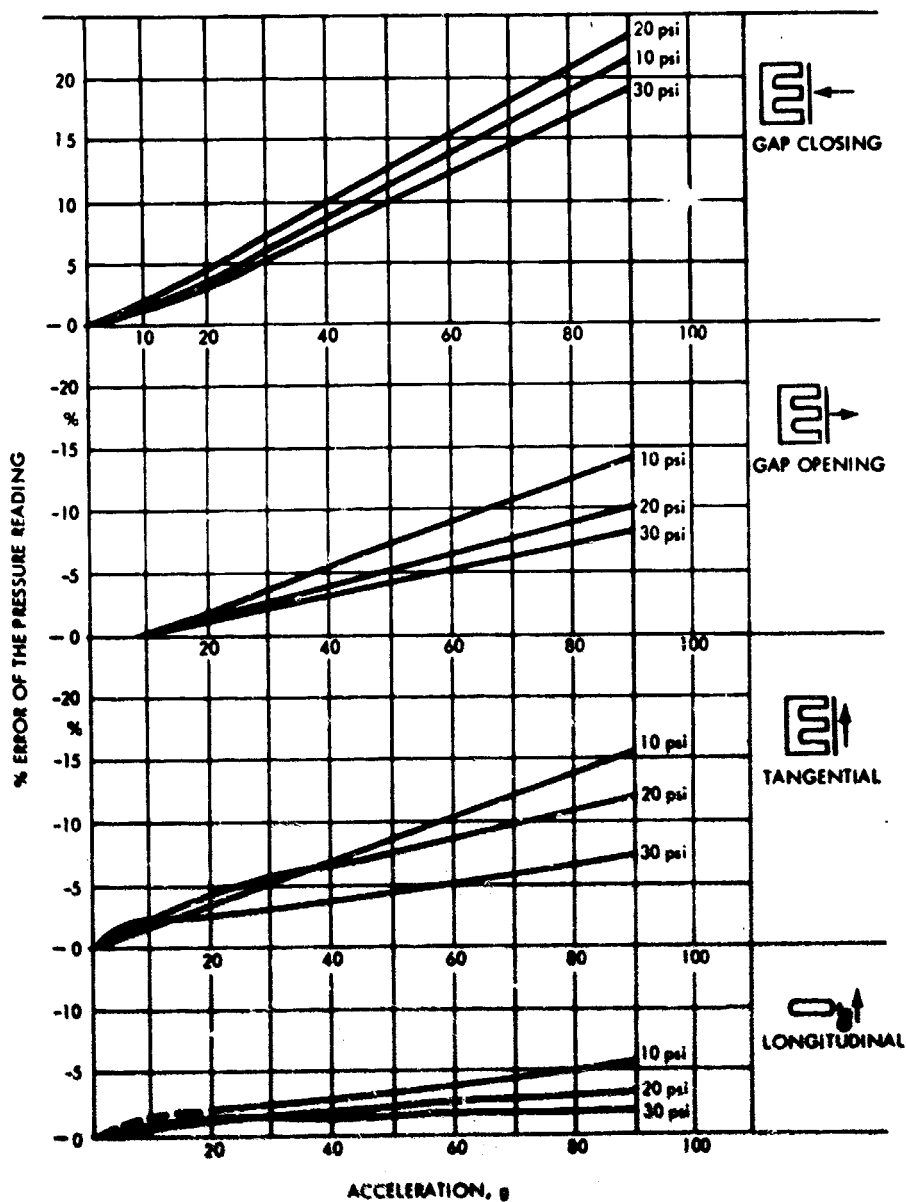
Figure 6. Effects of acceleration on 30-psi Wiancko gage (data from Reference 7).
