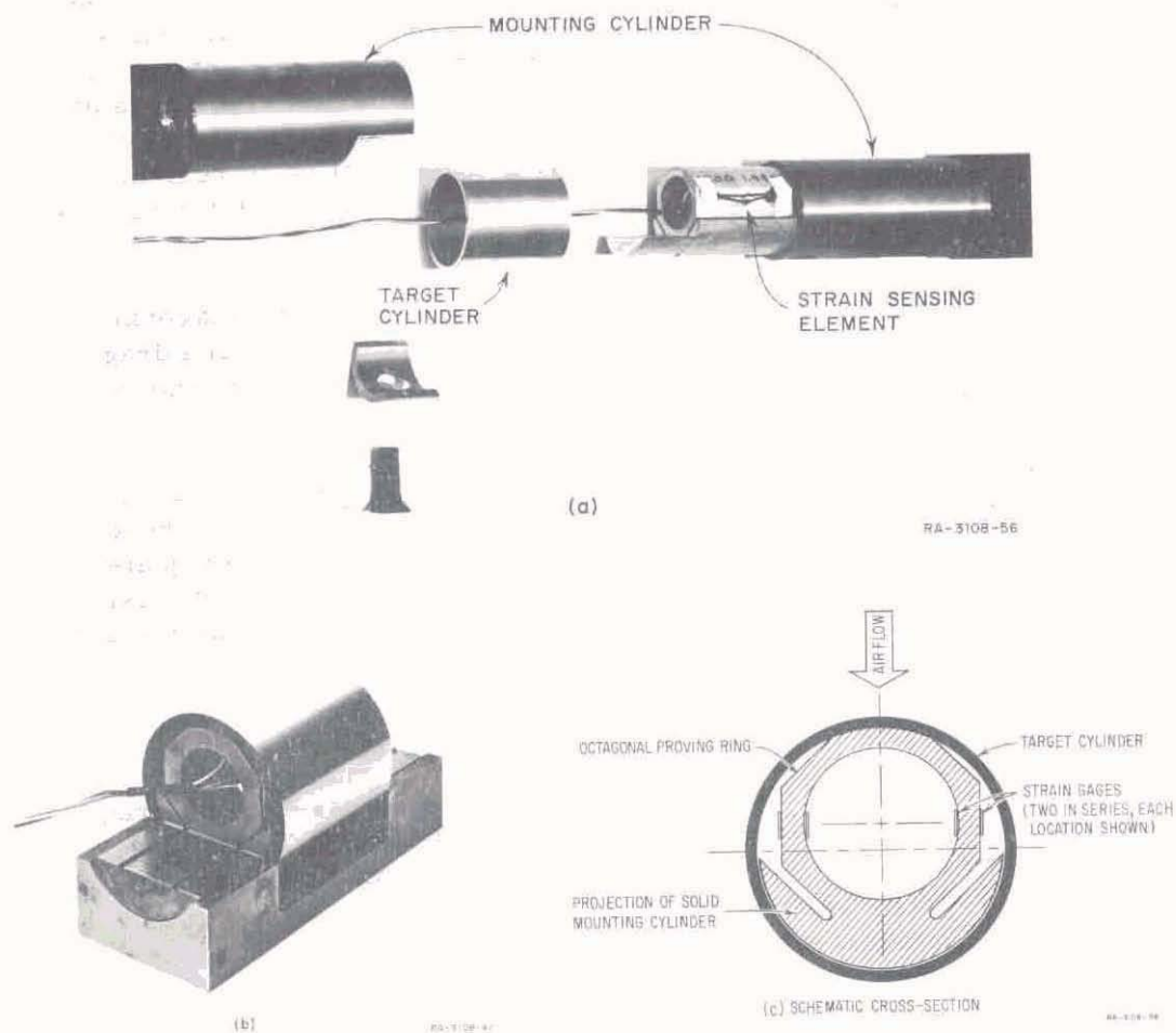
Figure 21. Total drag probe assembly: (a) exploded view—drag probe shown is for 50 psi overpressure region, (b) 500-psi probe shown on calibrating jig, (c) schematic cross-section.
