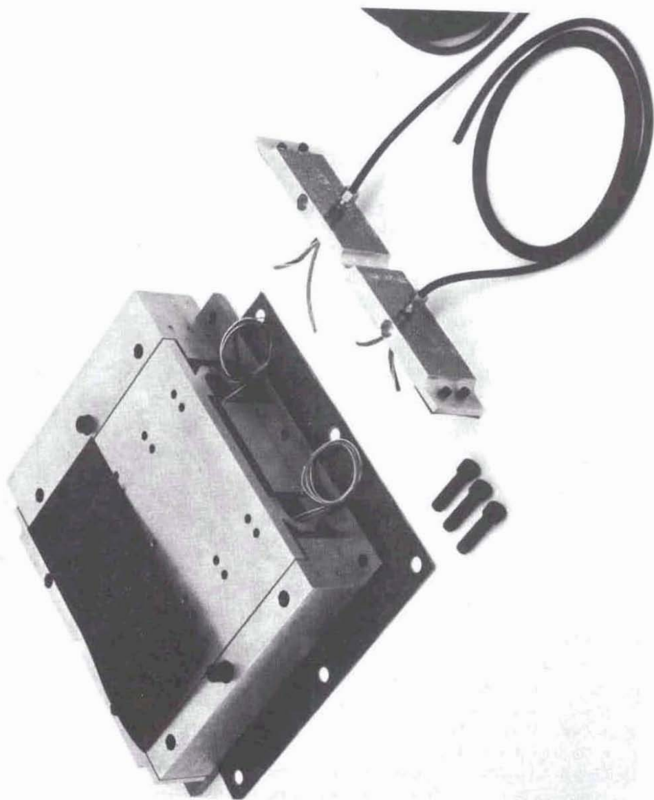
Figure 38. SRI surface shear gage.
