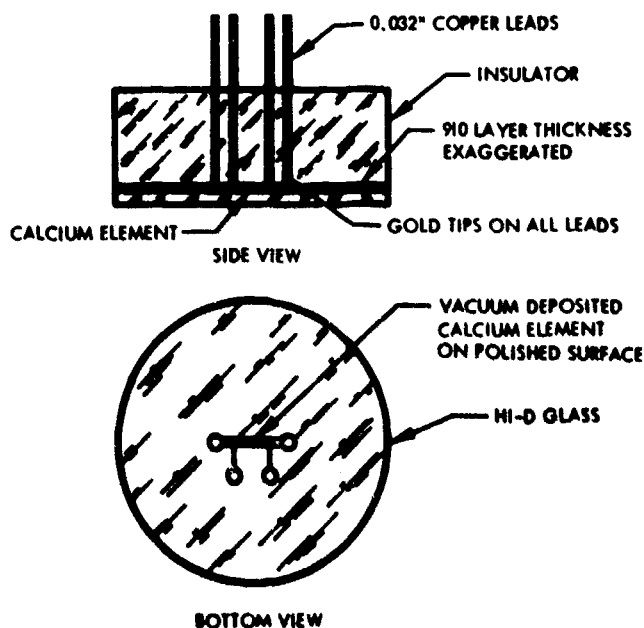
Figure 28. SRI calcium pressure gage.
