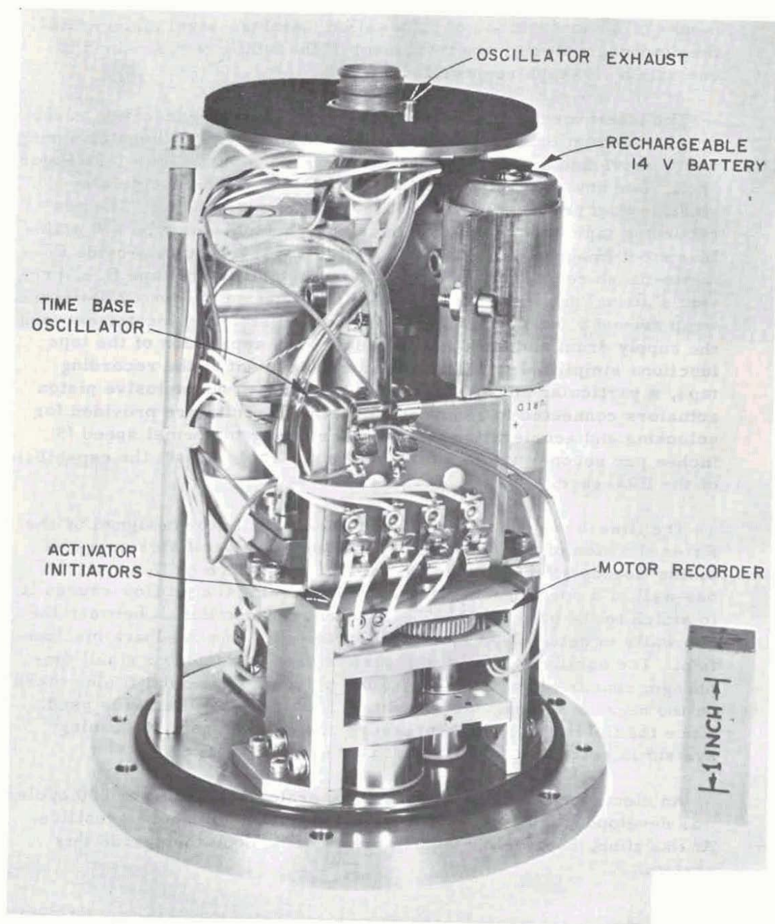
Figure 12a. BRL self-recording system.
