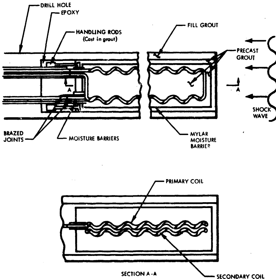
Figure 34. EPCO self-inductance particle velocimeter.
