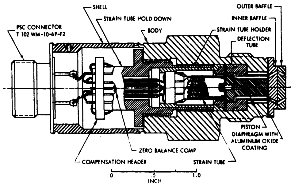
Figure 10. BRL high pressure airblast gage using the Dynisco pressure transducer.
