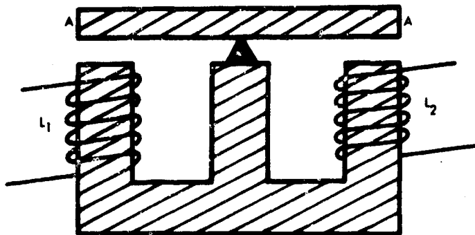
Figure 3. Schematic diagram of a variable reluctance sensor.
