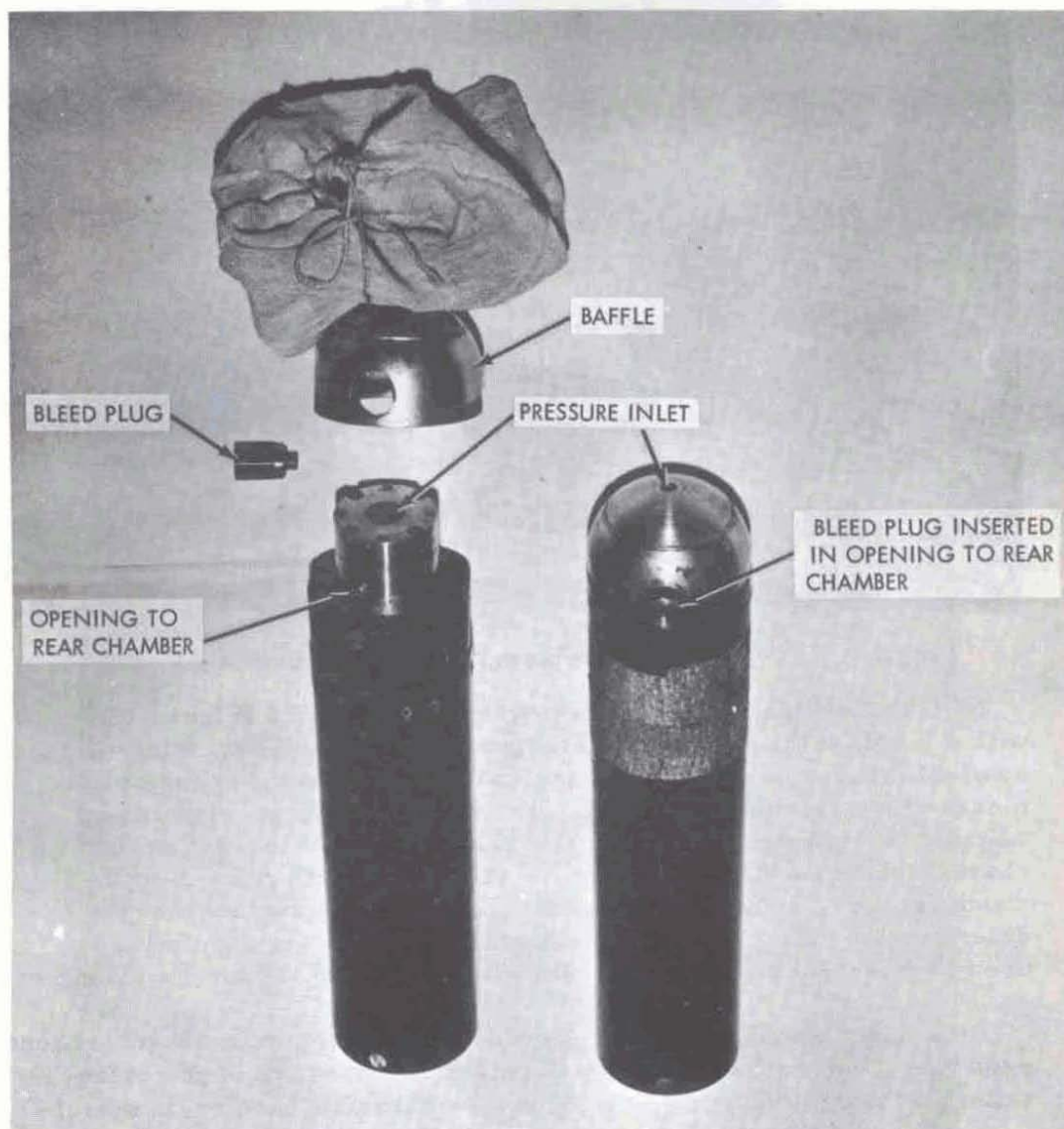
Figure 16. NOL airblast gage with hemispherical baffle.
