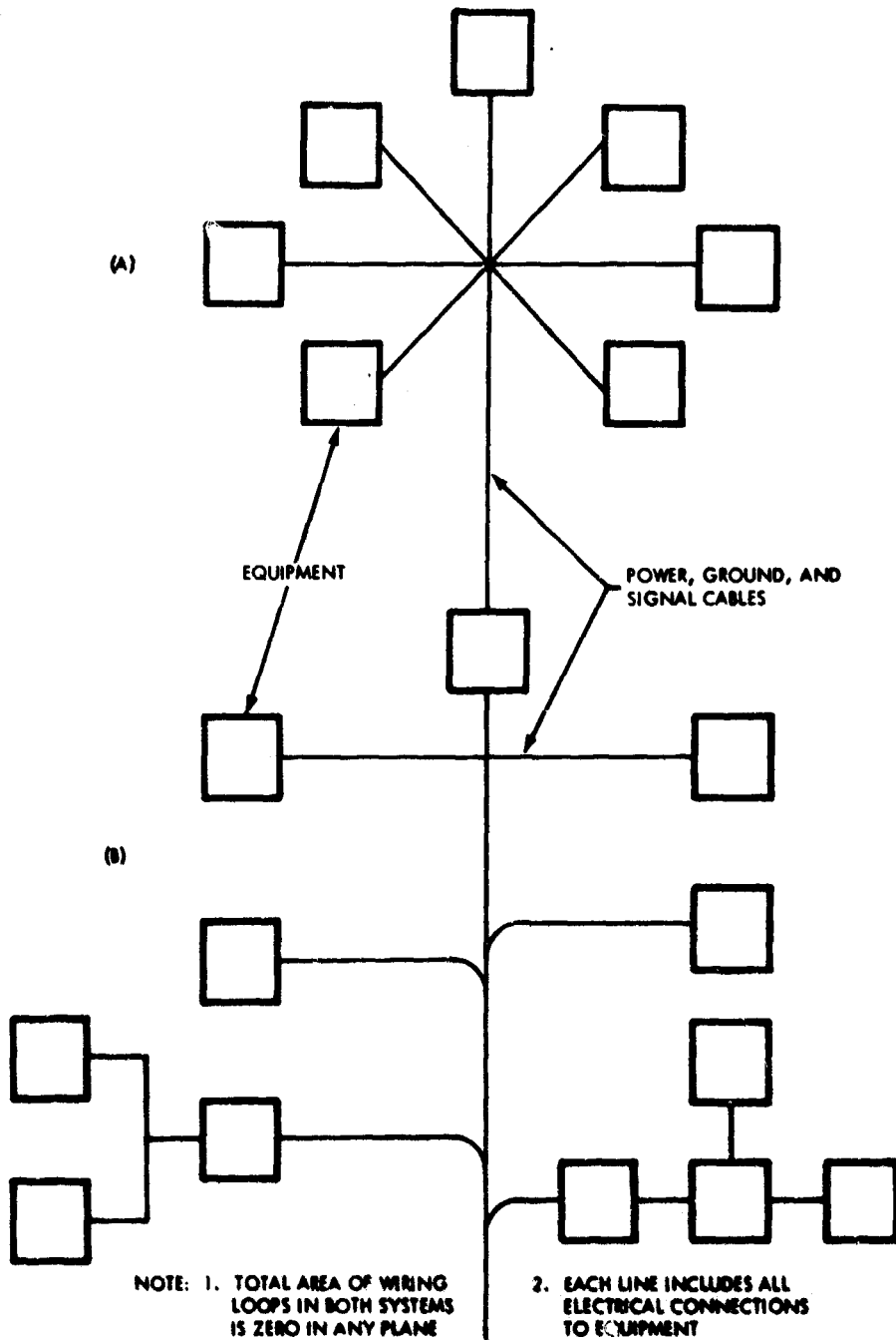
Figure 5. Wiring to reduce EMP susceptibility (A) Radial, (B) "TREE" wiring system.
