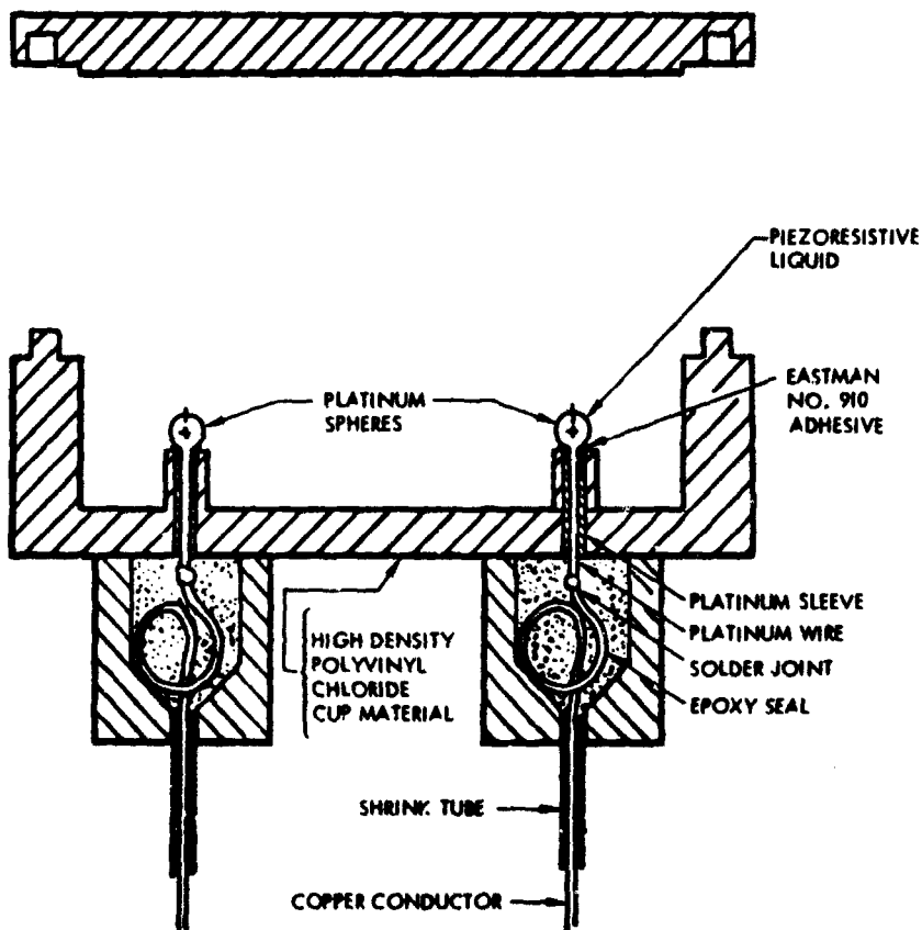
Figure 29. IITRI high-pressure electrolytic cell shock pressure gage.
