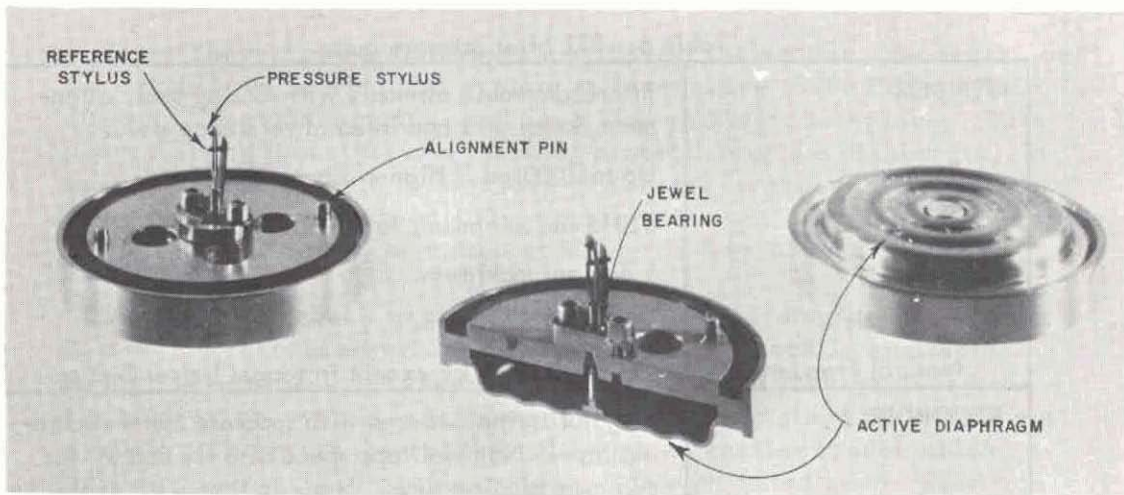
Figure 12b. BRL self-recording system.
