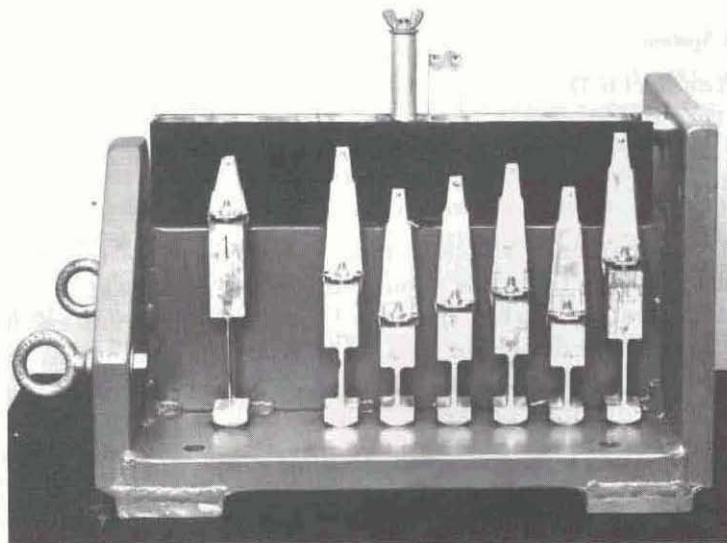
Figure 44. TRW reed gage.
