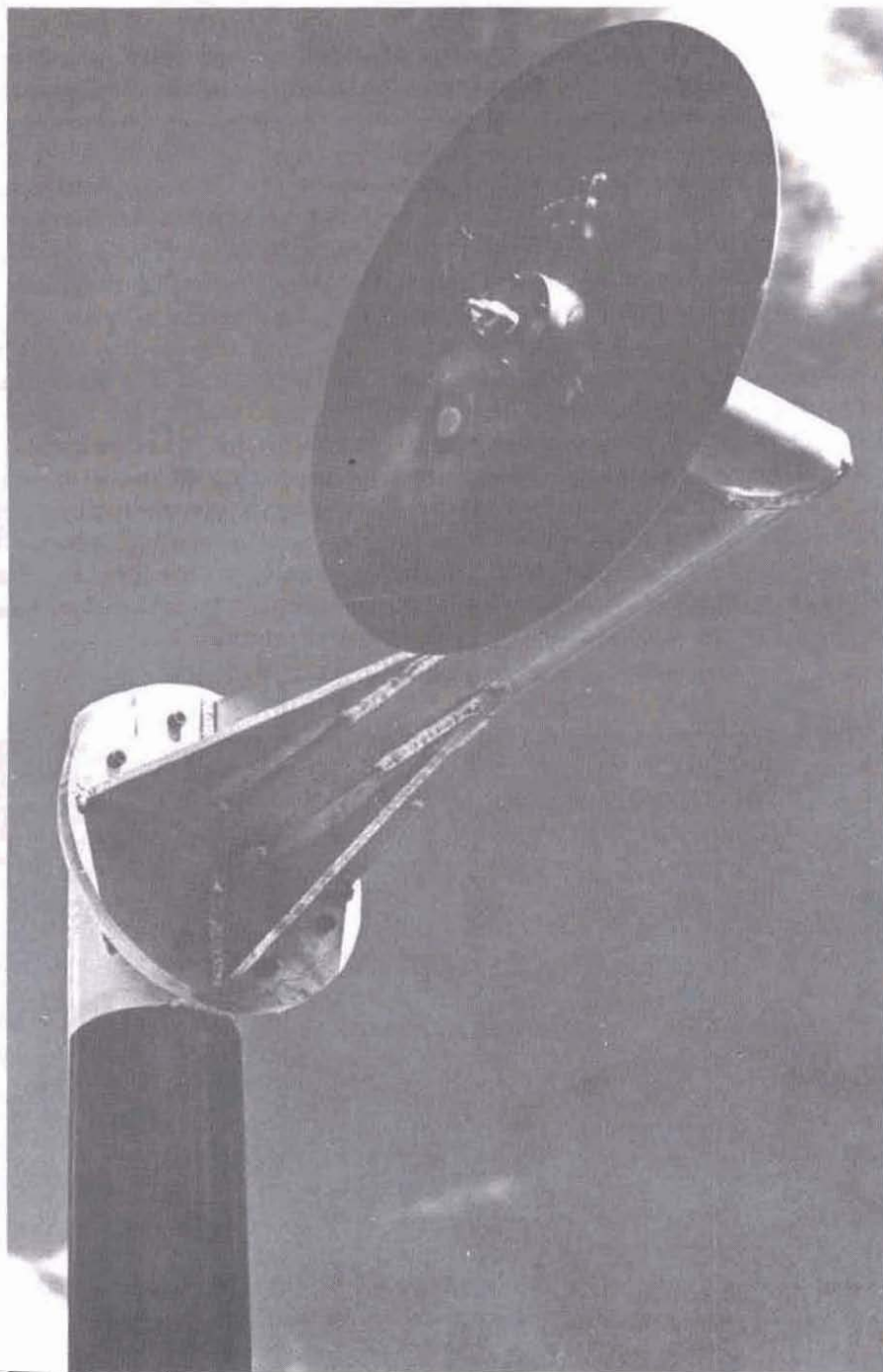
Figure 14. Side-on baffle for an airblast gage.
