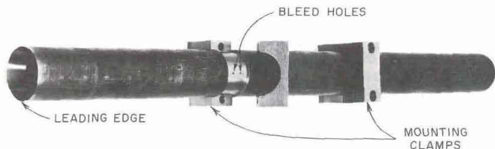
Figure 20. Dust sampler (explosive closures not shown).
