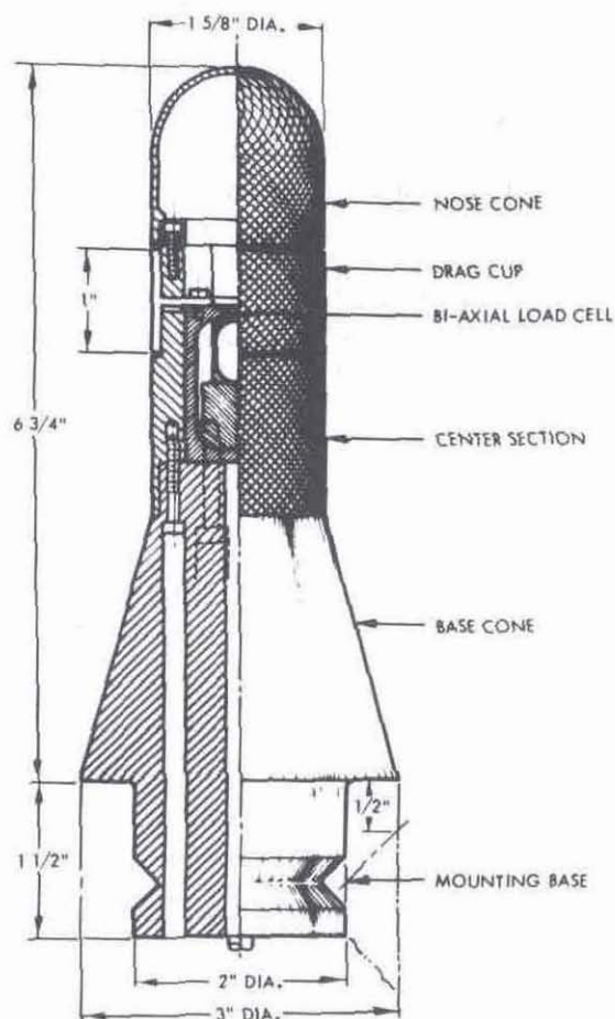
Figure 23. Assembly drawing of BRL bi-axial drag gage.
