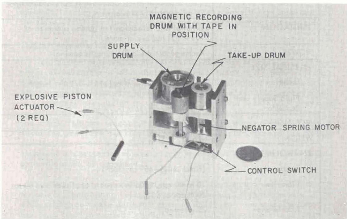
Figure 12c. BRL self-recording system.
