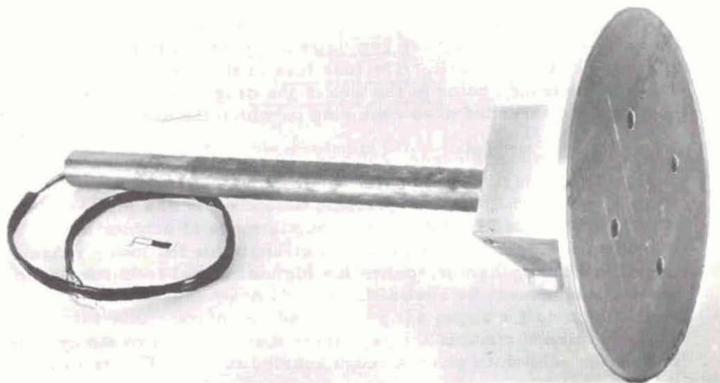
c. SRI-BRL circular plate drag force gage.
