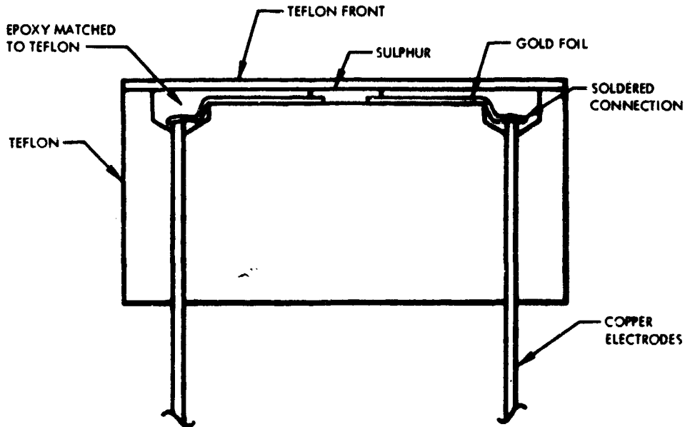
Figure 27. BRL sulphur gage.
