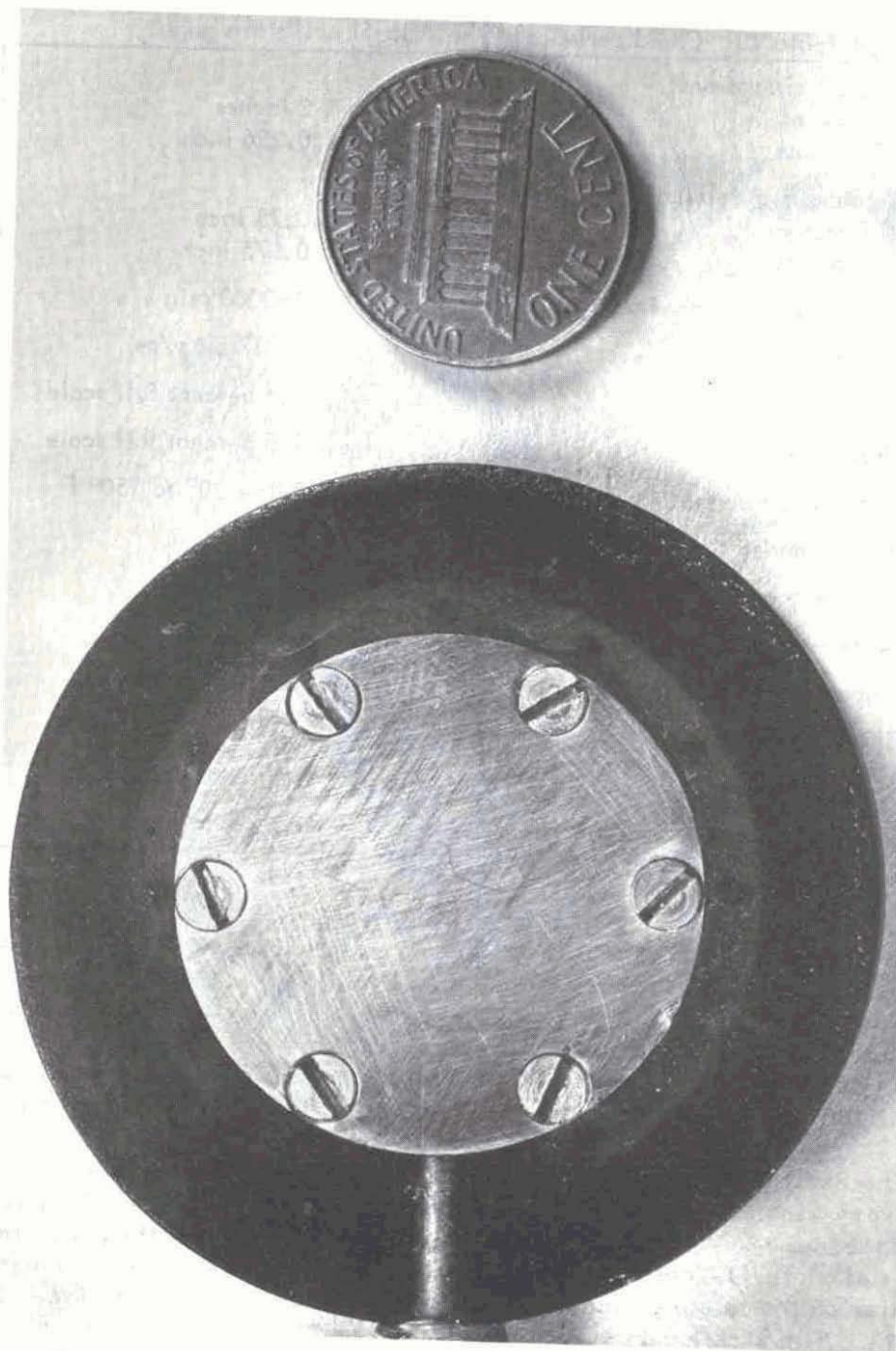
Figure 37. WES-SE soil stress gage.
