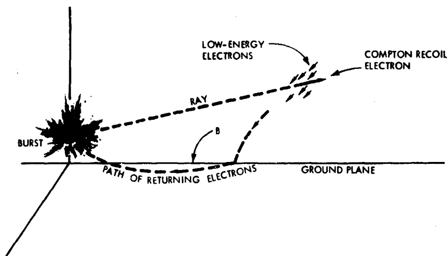
Figure 4. Influence of ground on return conduction current.
