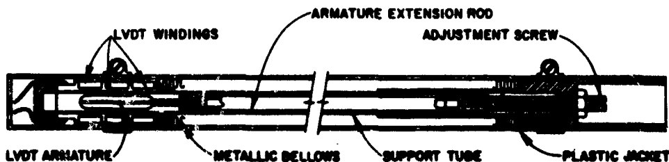
Figure 40. SRI strain gage.
