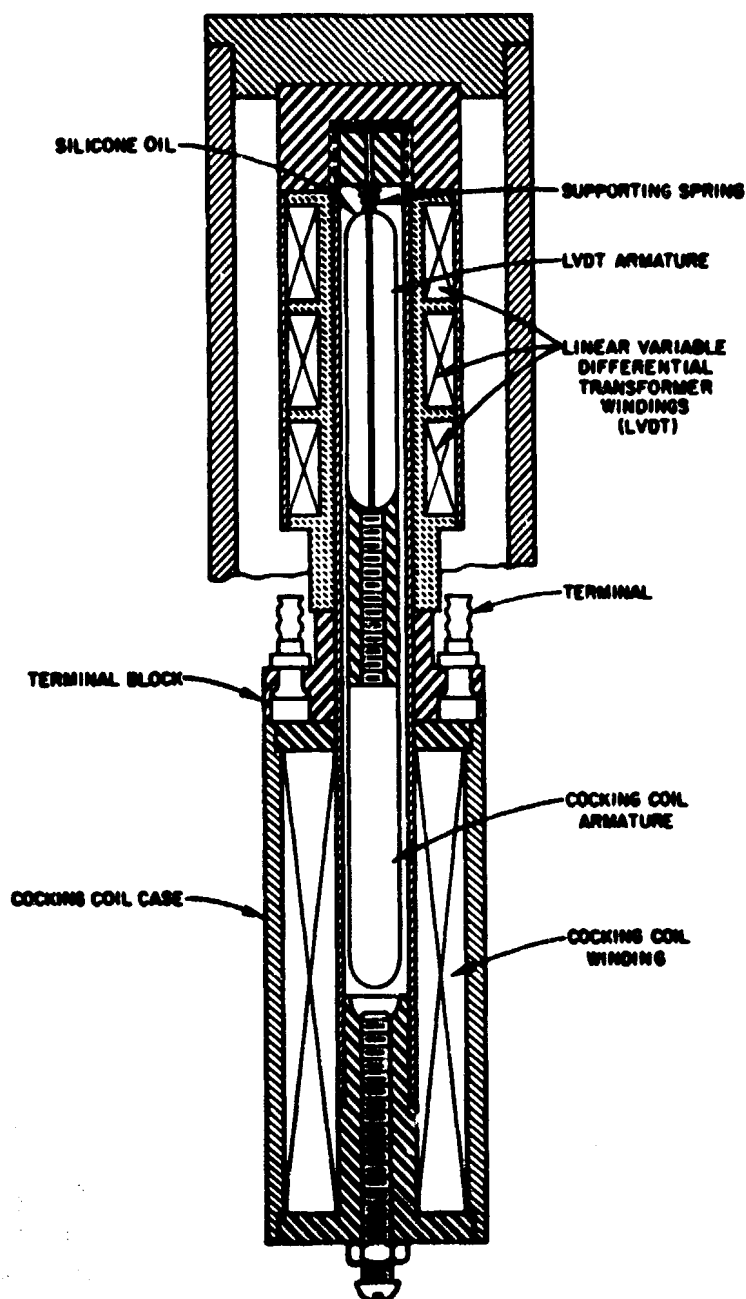
Figure 41. SRI Mark I velocity gage.
