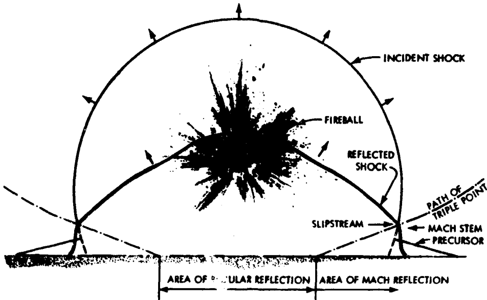
Figure 2. Blast wave terminology for low air burst.
