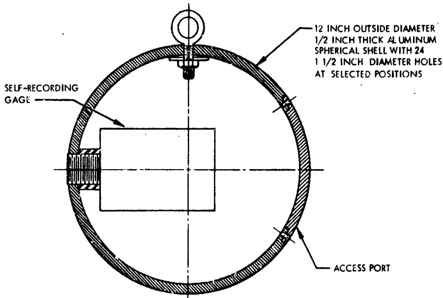
Figure 17. BRL non-directional gage mount for the BRL mechanical self-recording gage.
