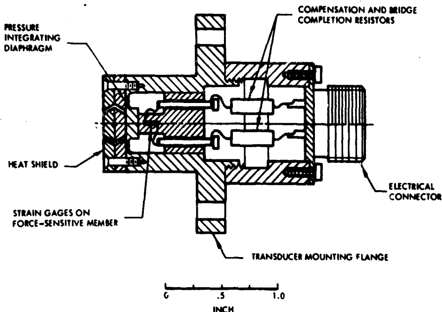
Figure 11. Bytrex pressure transducer used by BRL.
