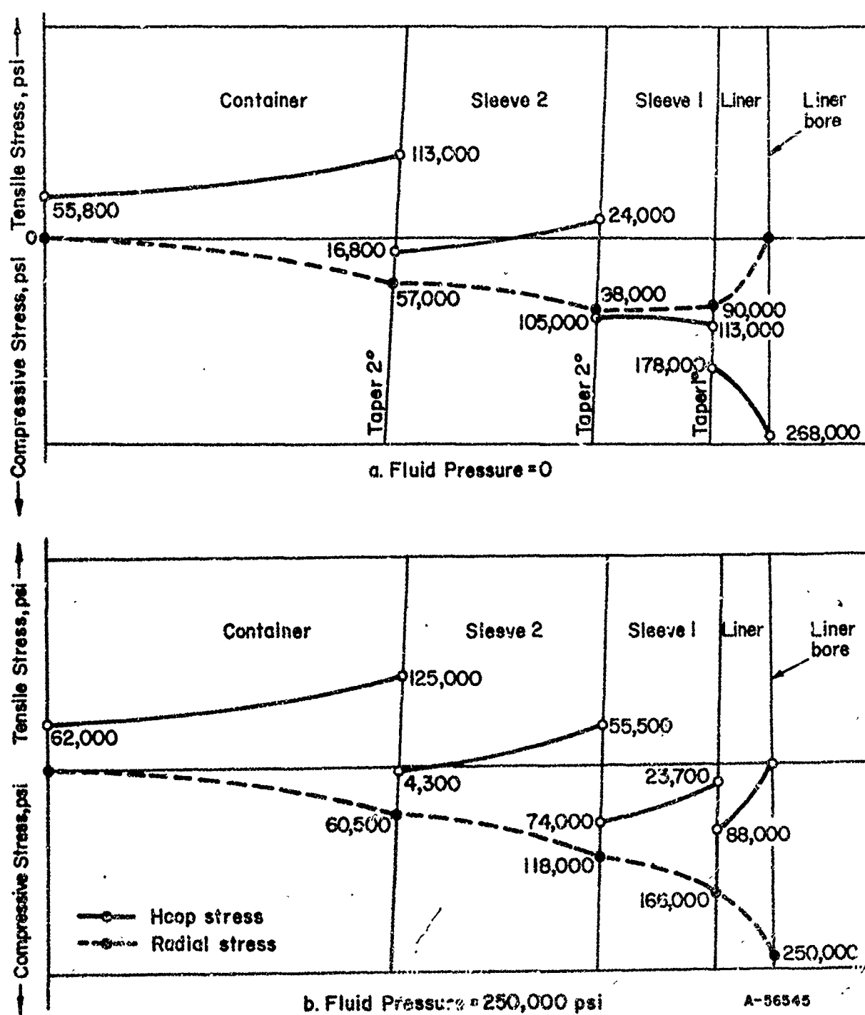
FIGURE 76. DESIGN STRESS PATTERN IN CONTAINER III AT ROOM TEMPERATURE
