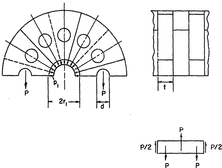
FIGURE 81. LOADING OF PINS
