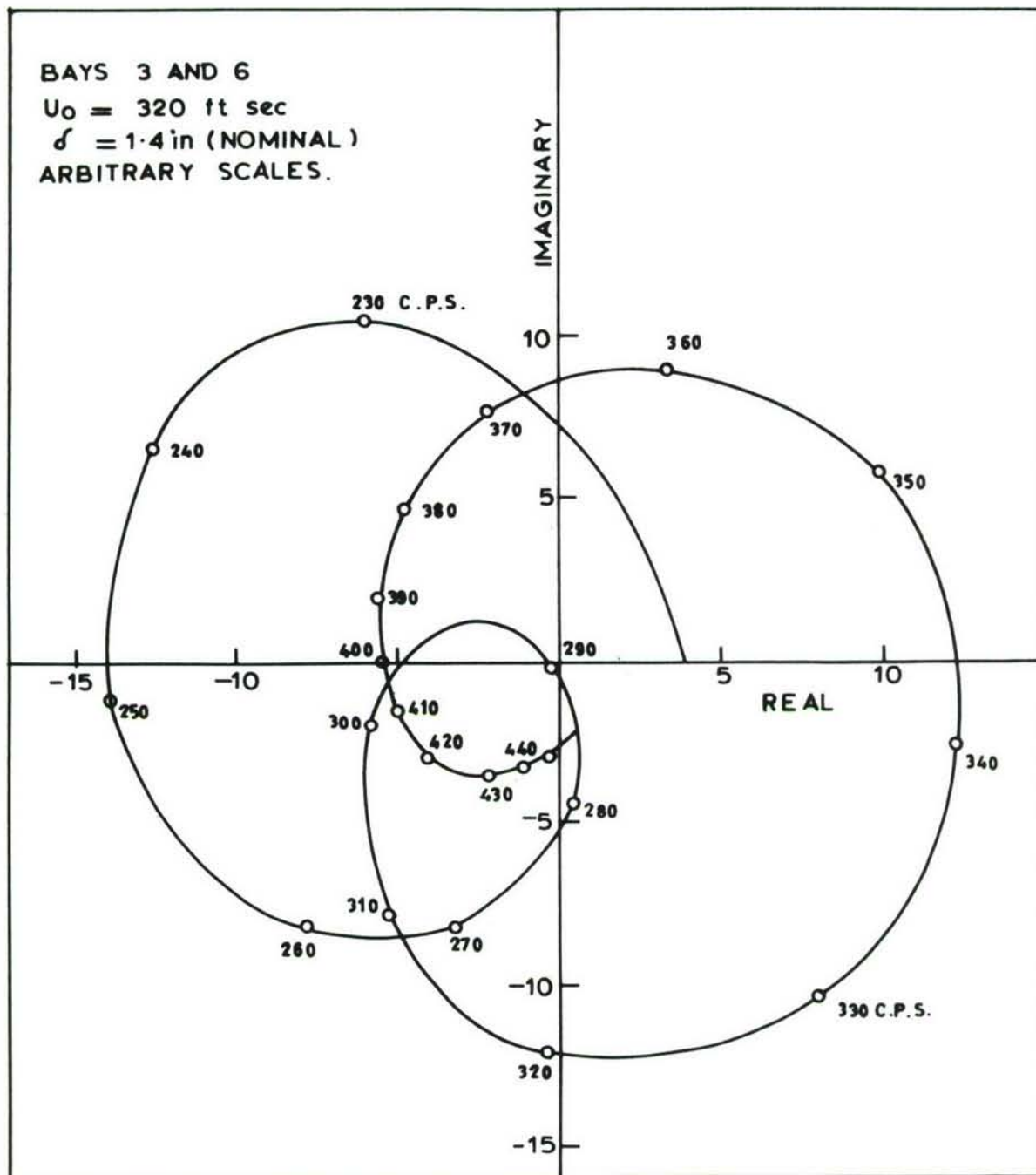
Fig. 47. Displacement cross power spectrum for bays 3 and 6 of 8-bay array : boundary layer excitation.
