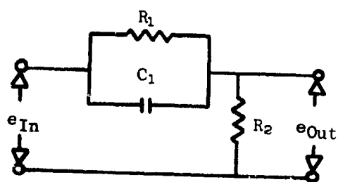
Electrical Circuit
