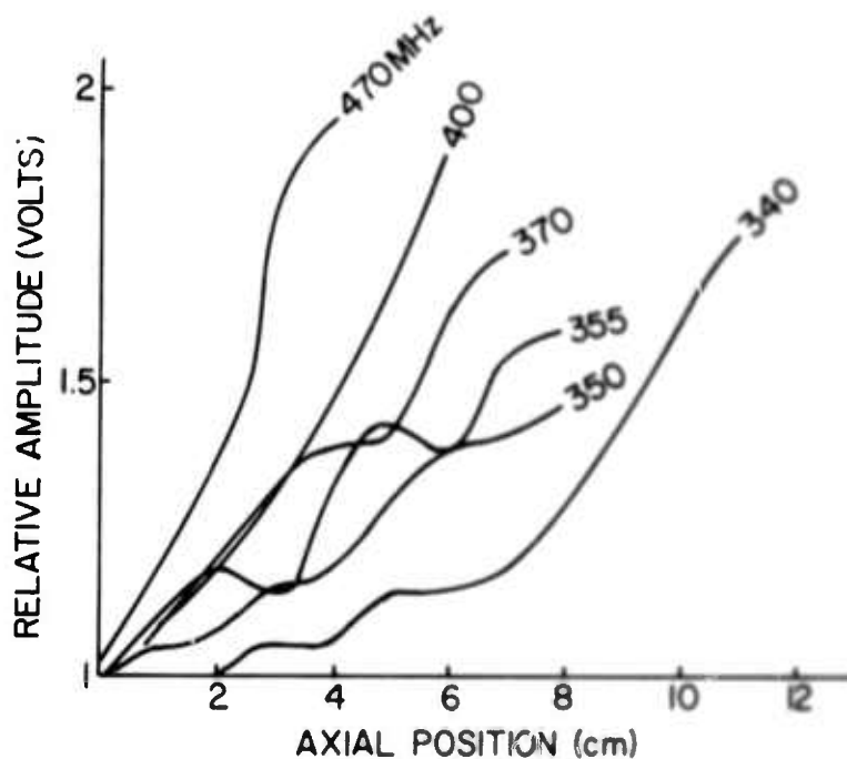
6 Beam-surface wave interaction: Variation of phase and amplitude along the tube.
