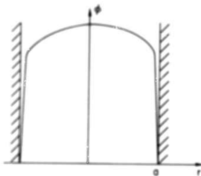
3. Profiles of plasma density, n , and self-consistent potential, \phi , as a function of radius.
