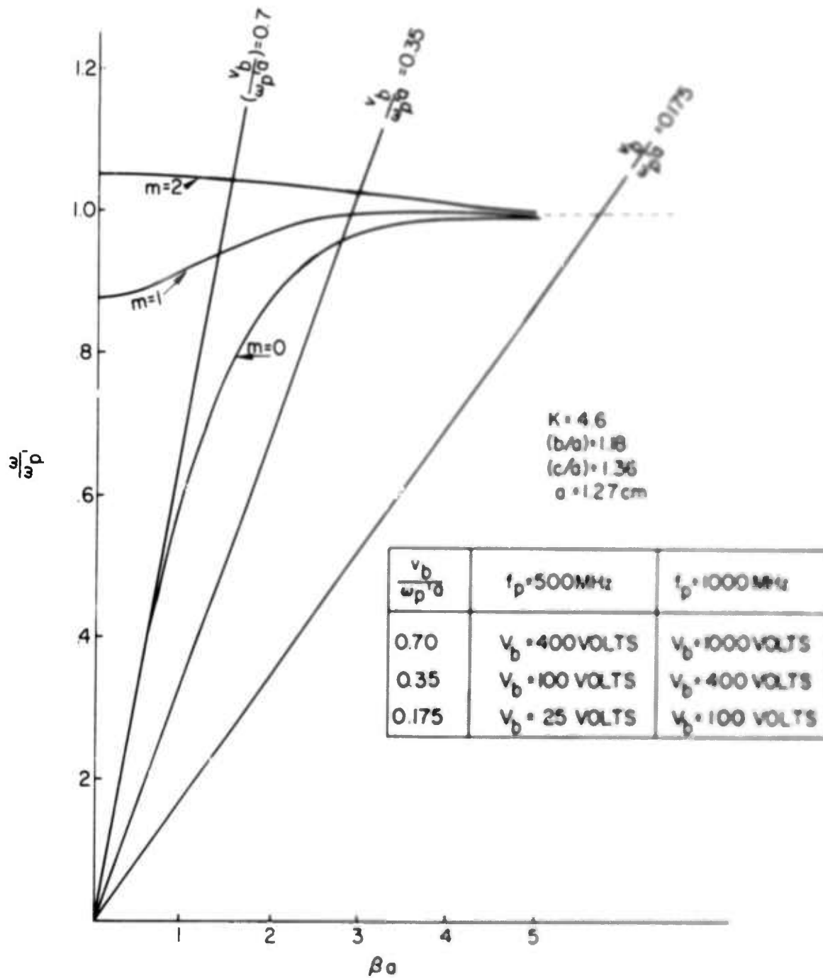
1 (b) Surface Wave Propagation Characteristics, (c/a) = 1.36
