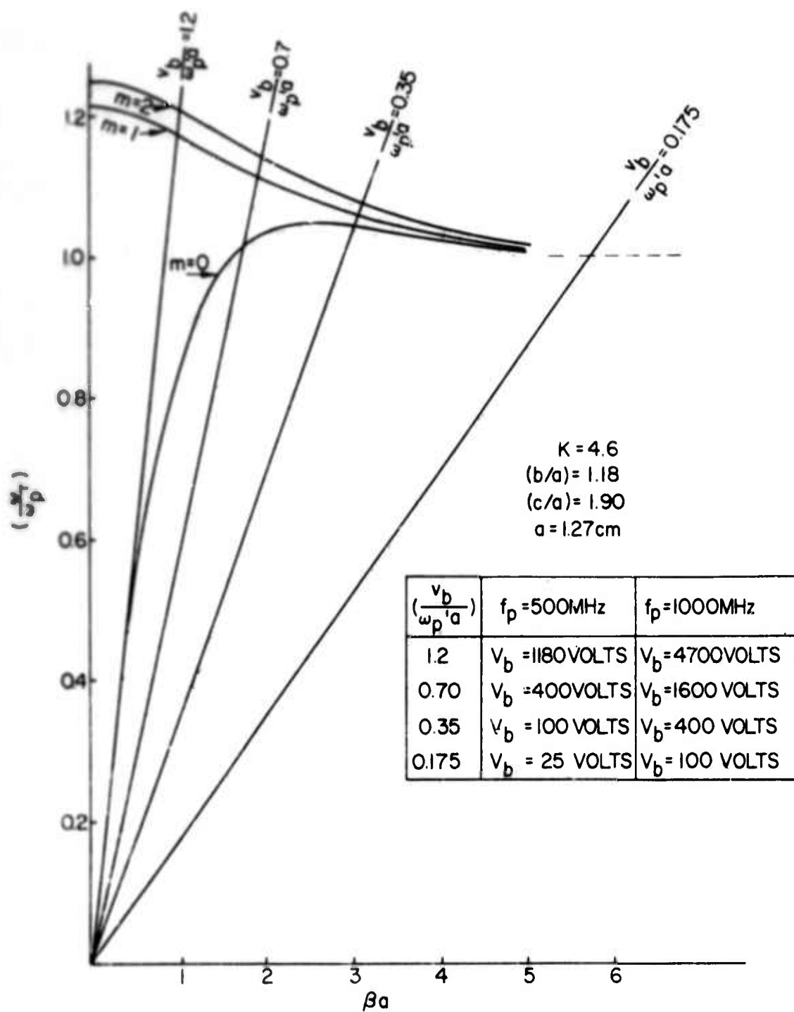
1 (a) Surface Wave Propagation Characteristics. (c/a) = 1.90
