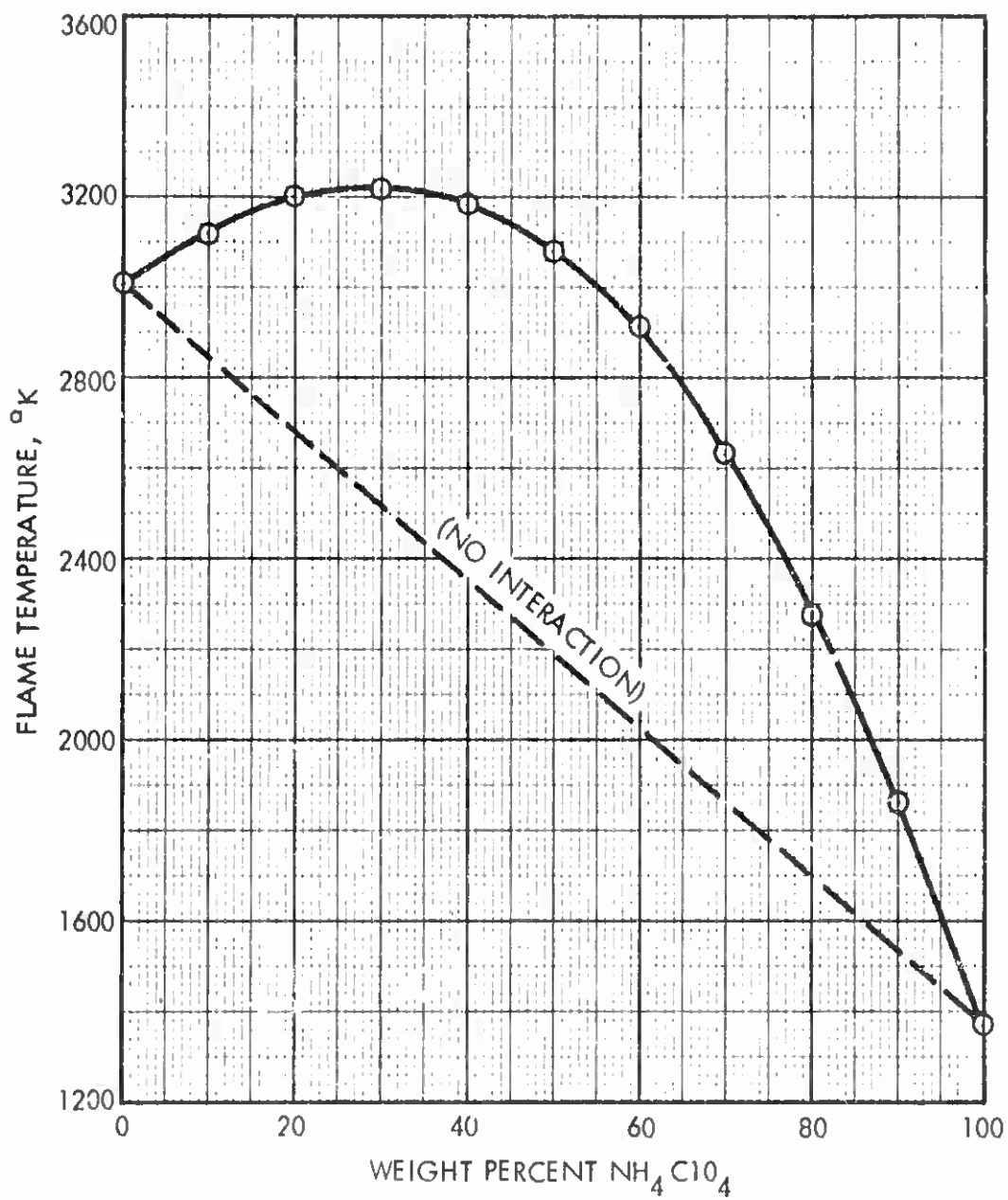
FIGURE C-4. THEORETICAL FLAME TEMPERATURE AT 1500 psia FOR CONSTANT PRESSURE COMBUSTION OF JPN-AP MIXTURES
