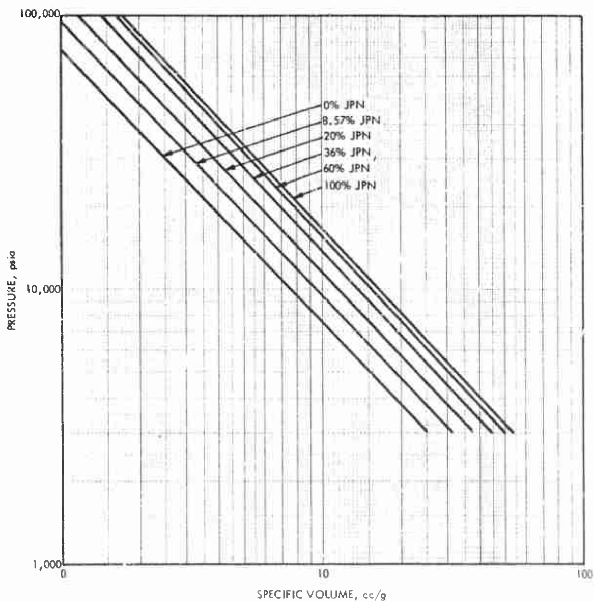
FIGURE C-3. THEORETICAL PRESSURE VERSUS SPECIFIC VOLUME FOR ADIABATIC COMBUSTION OF JPN-AP MIXTURES
