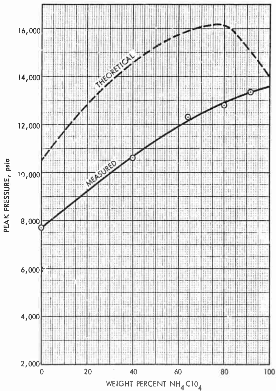
FIGURE C-2. THEORETICAL AND MEASURED PEAK PRESSURES VERSUS WEIGHT PERCENT \text{NH}_4\text{ClO}_4
