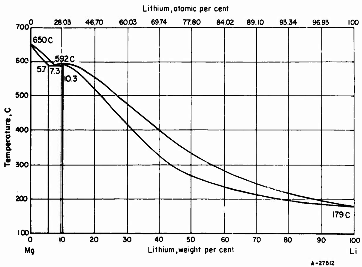
FIGURE 1. MAGNESIUM-LITHIUM EQUILIBRIUM DIAGRAM (GRUBE)
