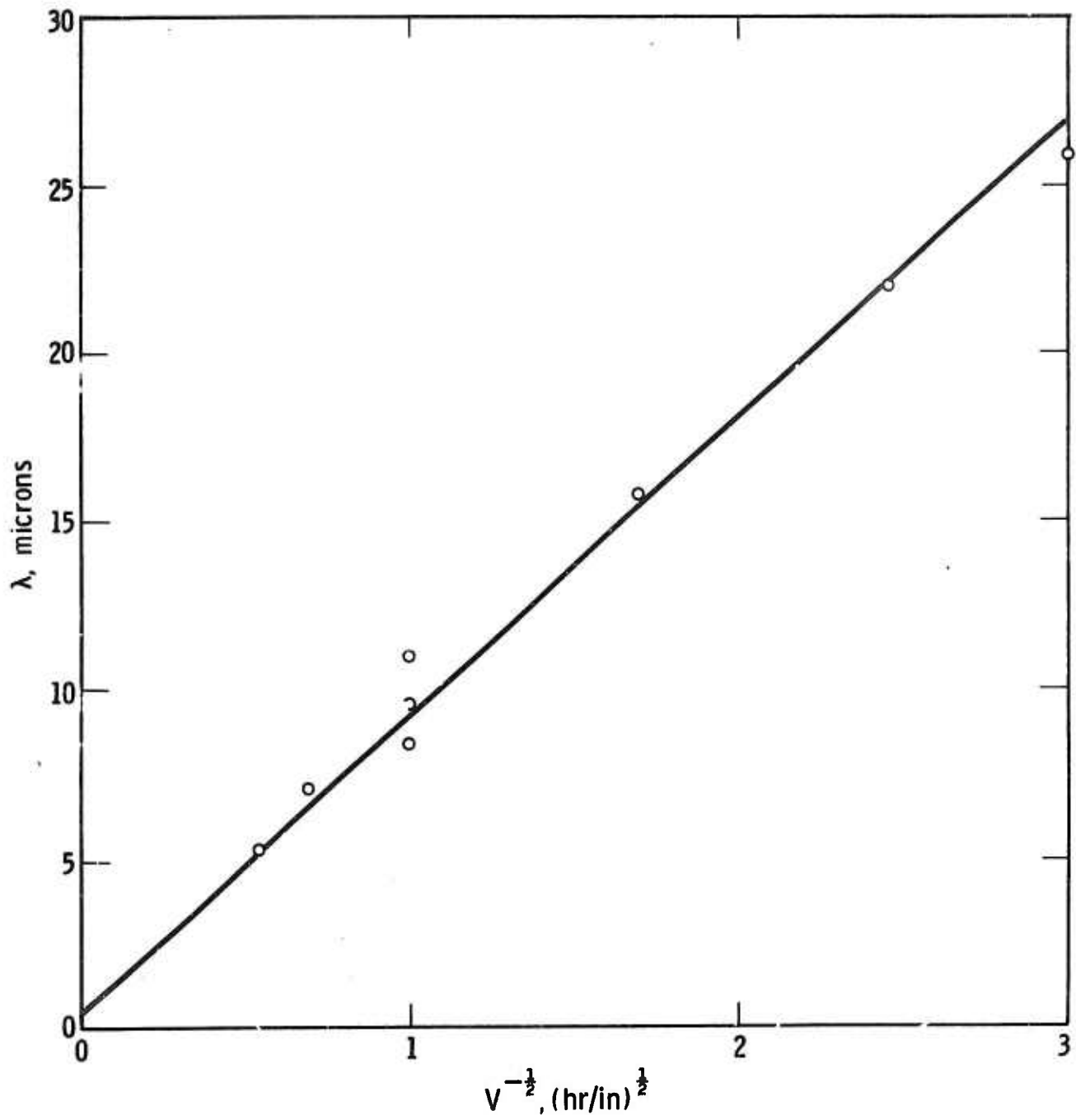
Fig. 6-Lamellar spacing as a function of (\text{velocity})^{-\frac{1}{2}} for Ni-Cr eutectic
