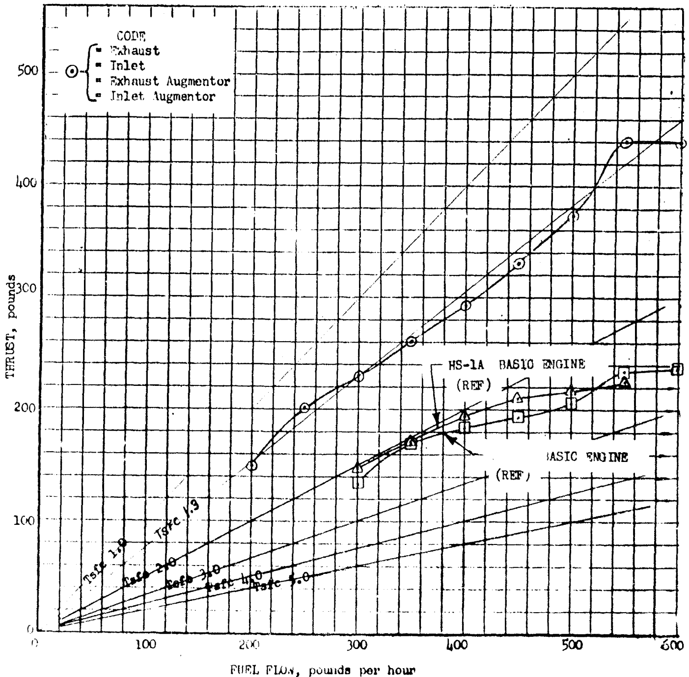
FIGURE A-4: HS-1A ENGINE WITH AUGMENTORS (Basic engines HS-1A and HS-2C Ref)
