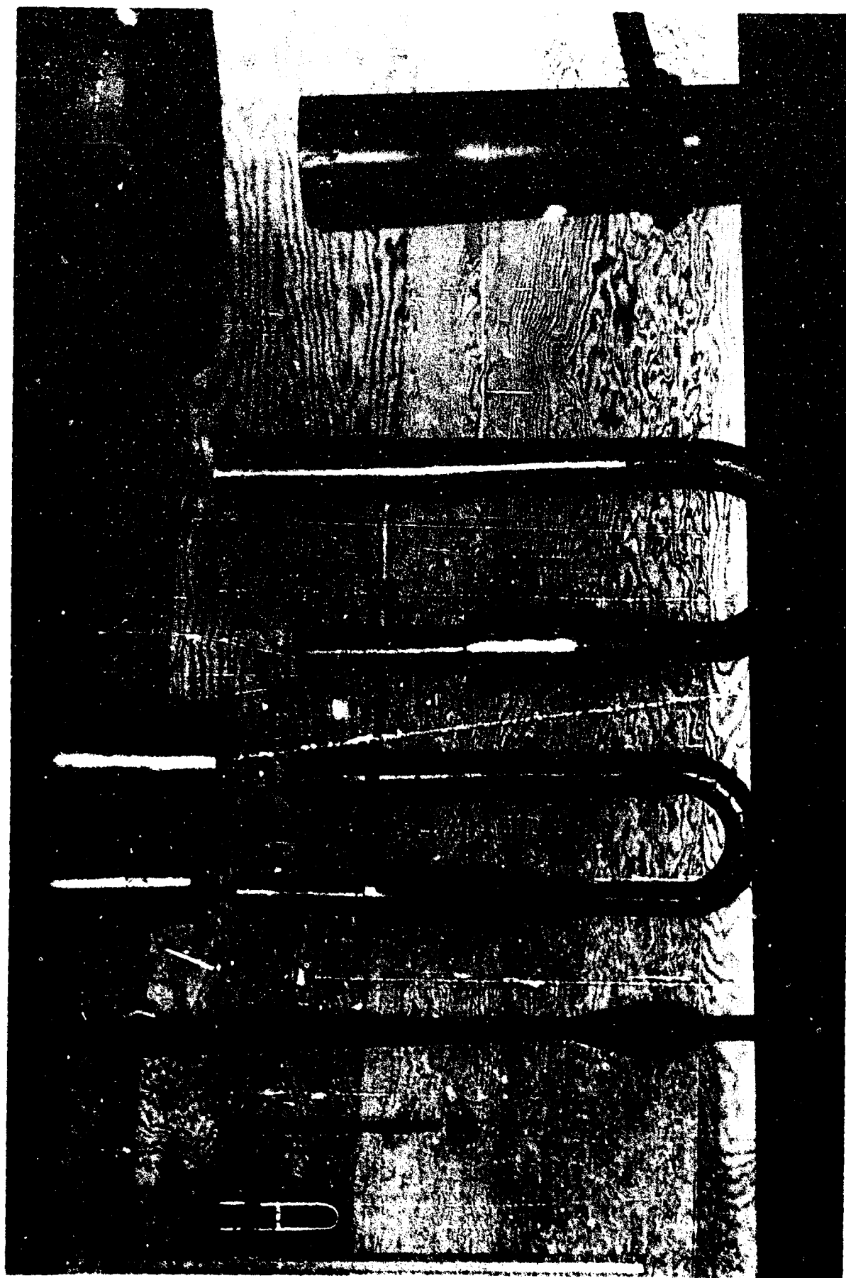
FIGURE A36: EXPERIMENTAL PULSE REACTORS SHOWING A RANGE OF SIZES FROM 0.7 INCH TO 8.6 INCH TAILPIPE DIAMETER
