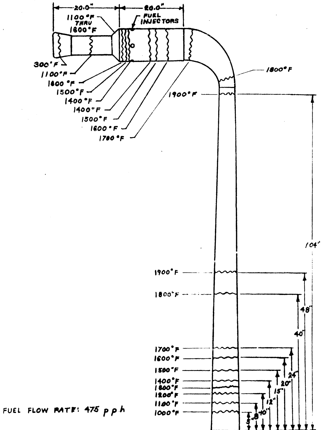
SHELL TEMPERATURE DISTRIBUTION FOR HS-1A ENGINE (UNCOOLED)
