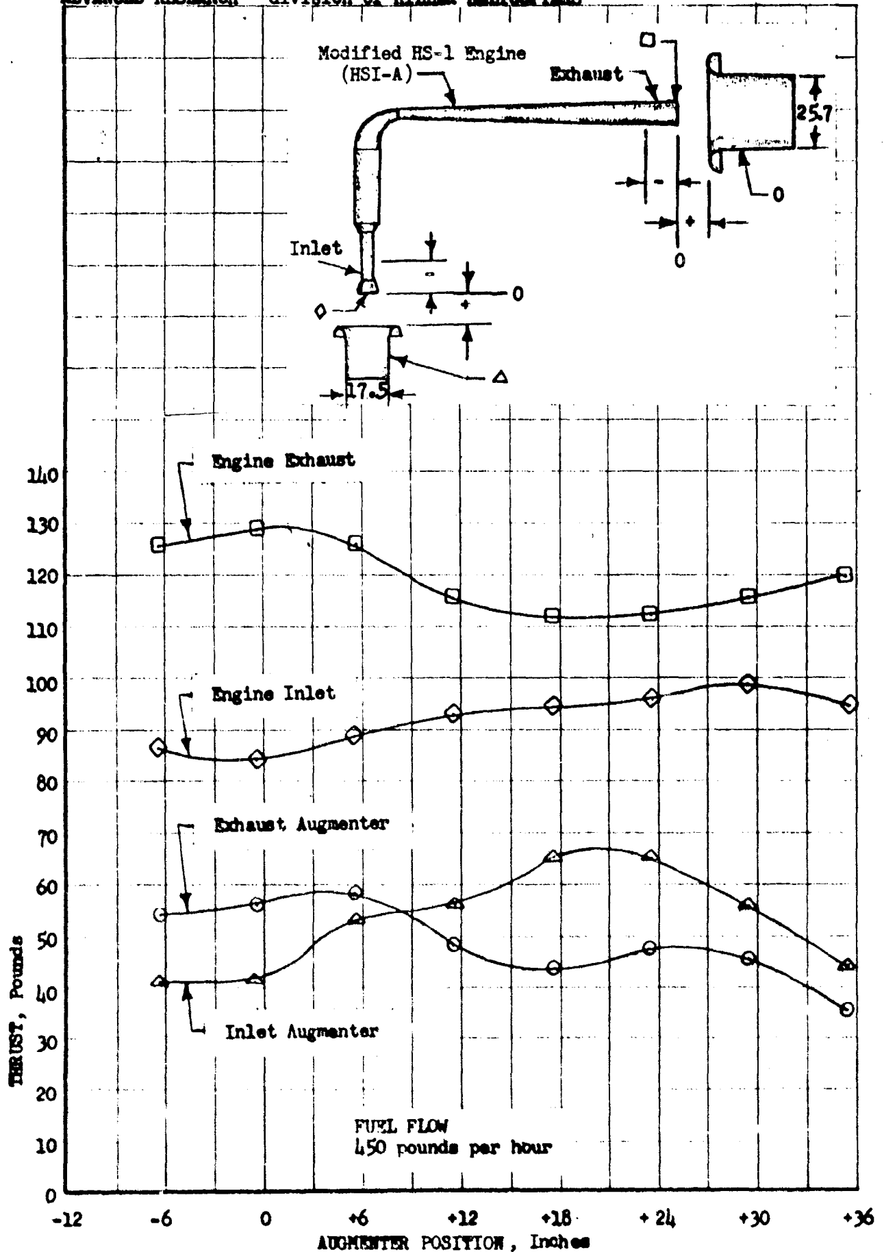
FIGURE A-23: EFFECT OF POSITION OF AUGMENTERS ON ENGINE AND AUGMENTER THRUST
