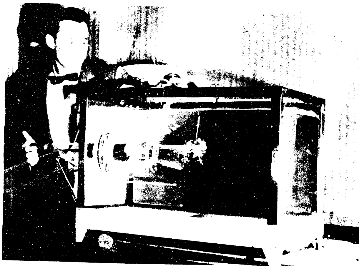
FIGURE 9. WATER TANK DEMONSTRATION OF INTERMITTENT JET FORMATION AND THRUST AUGMENTATION
