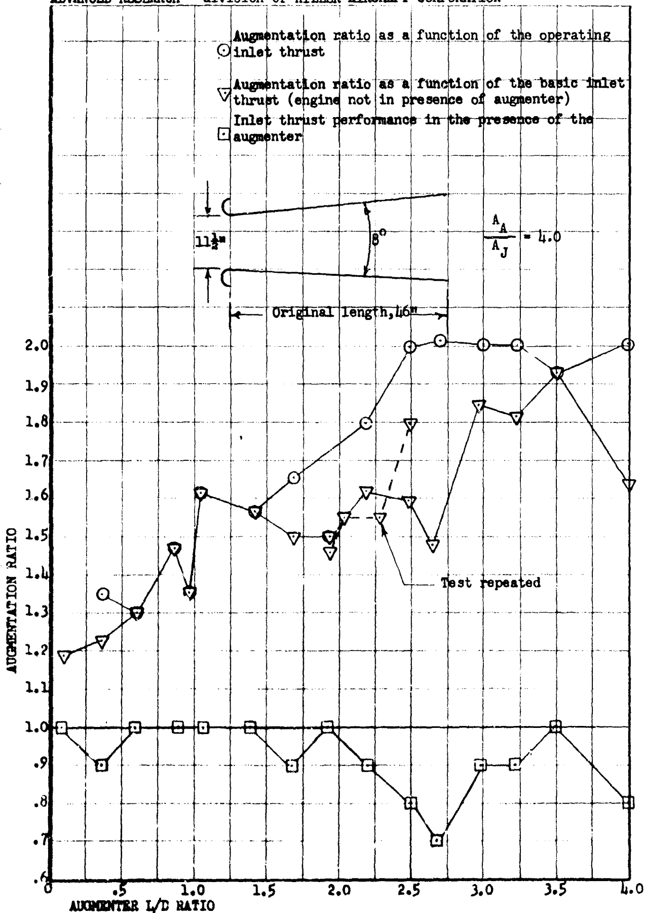
FIGURE A-25: EFFECT OF L/D RATIO ON INLET JET AUGMENTATION PERFORMANCE FOR AN 8° CONICALLY DIVERGENT AUGMENTER
