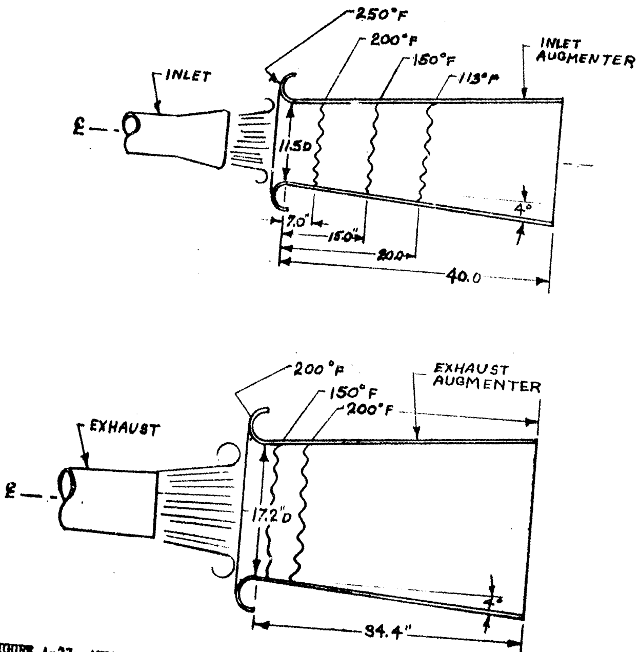
FIGURE A-27: AUGMENTER SHELL TEMPERATURES AT FUEL FLOW OF 475 pph
