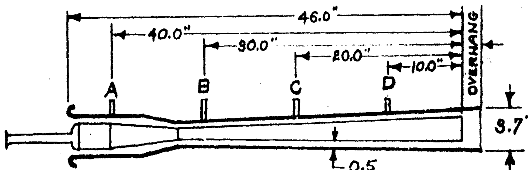
FIGURE A-18: COOLING SHROUD VACUUM INDUCED BY JET PUMPING
