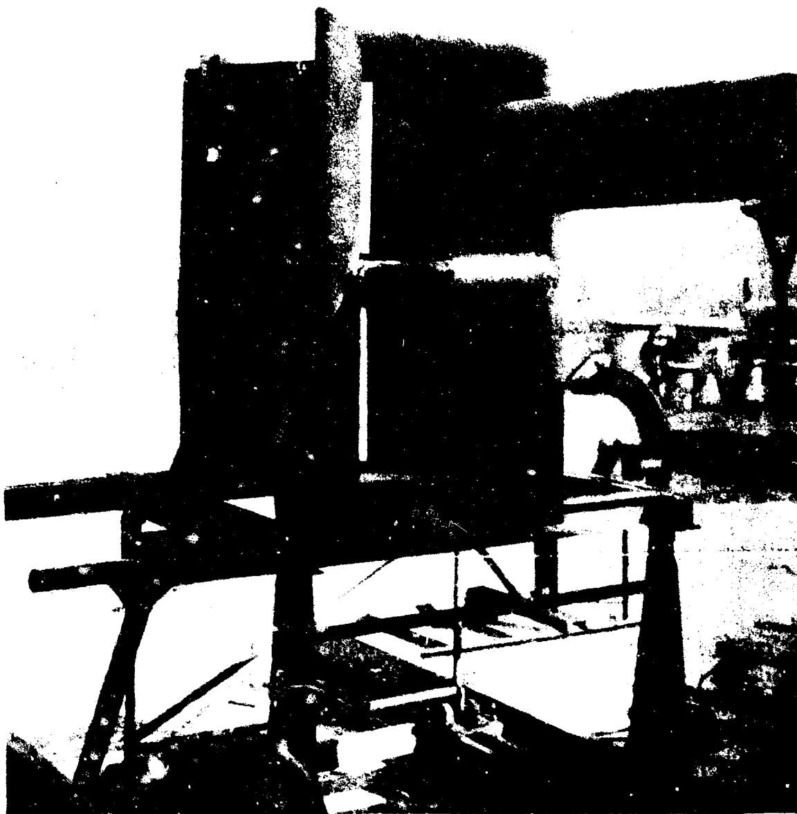
FIGURE A-31 8^\circ DIVERGENT RECTANGULAR AUGMENTER ON TEST STAND
