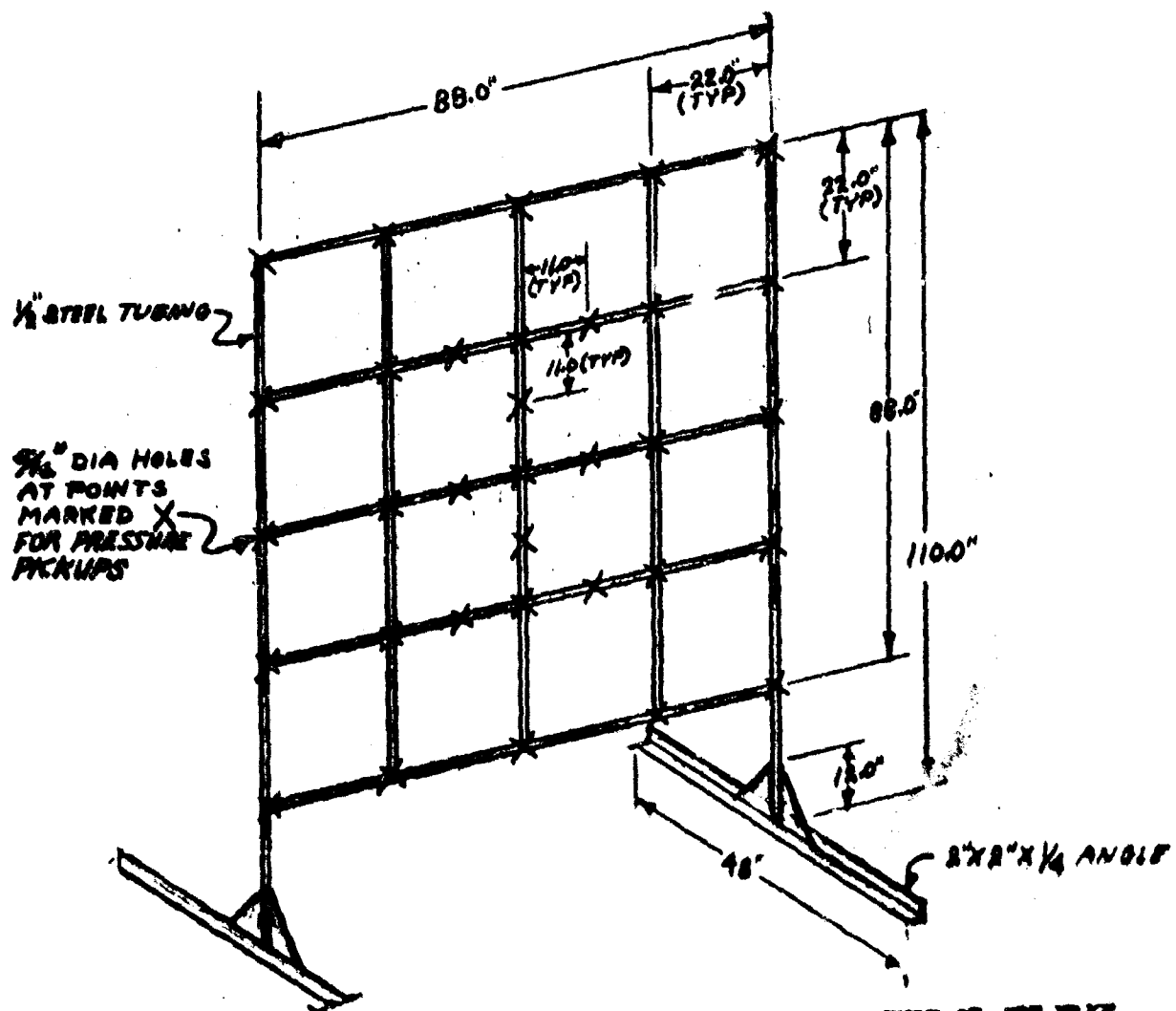
FIGURE A-32: TEST GRID FOR MEASURING PRESSURE AND TEMPERATURE OF JET WAKE.
