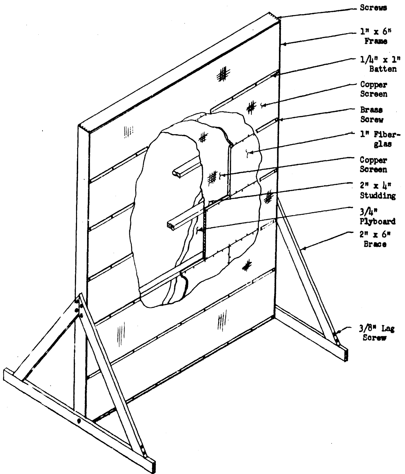
FIGURE A-33: ACOUSTICAL PANELS SHOWING CONSTRUCTION DETAILS AND MATERIAL
