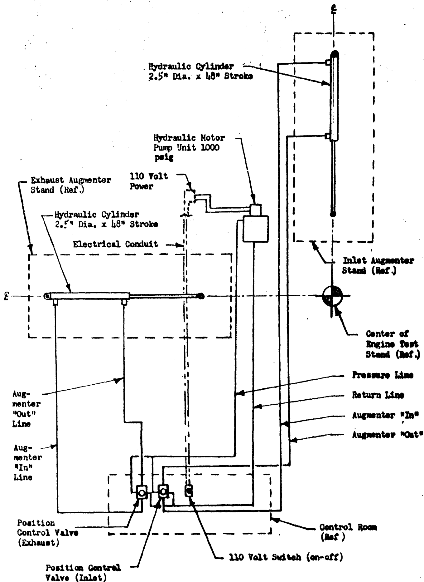
FIGURE A-22: HYDRAULIC-ACTUATED AUGMENTER POSITIONER
