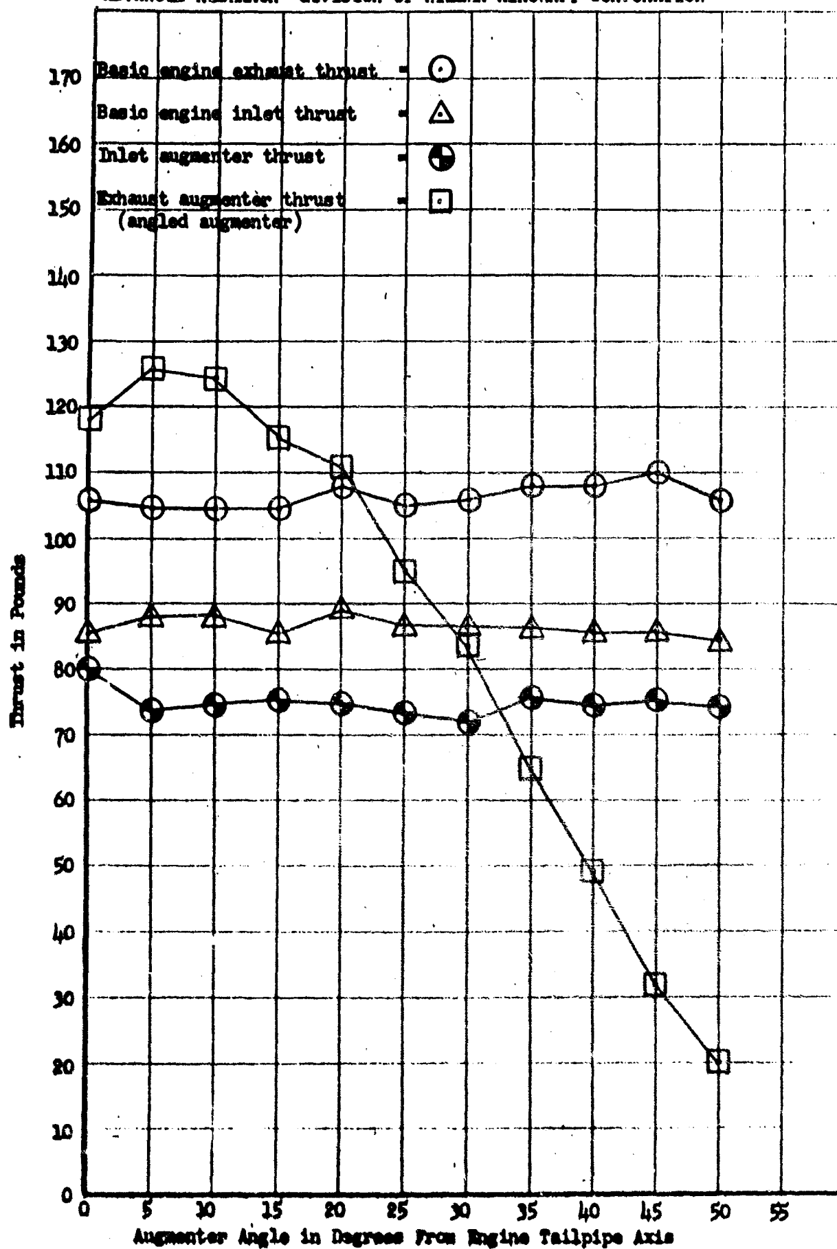
FIGURE A-30: ANGLED AUGMENTER DATA
