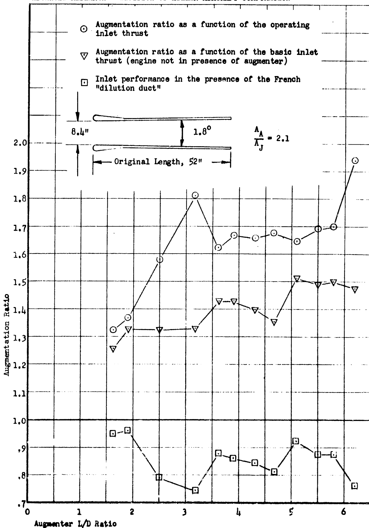
FIGURE A-26: EFFECT OF L/D RATIO ON AUGMENTATION PERFORMANCE FOR THE SNECMA "DILUTION DUCT"
