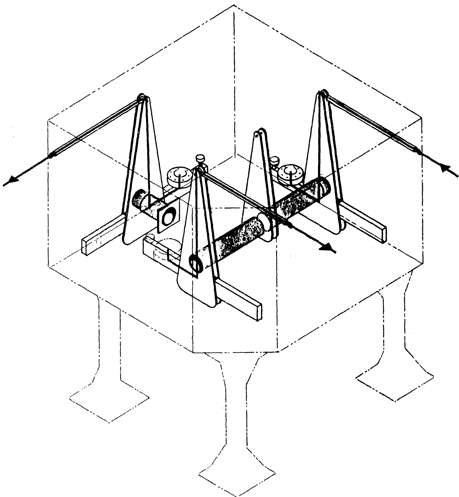
FIGURE A-10: SKETCH SHOWING MECHANISMS FOR TRANSMITTING ORTHOGONAL THRUST VECTORS INTO NULL-BALANCE LOAD CELLS
