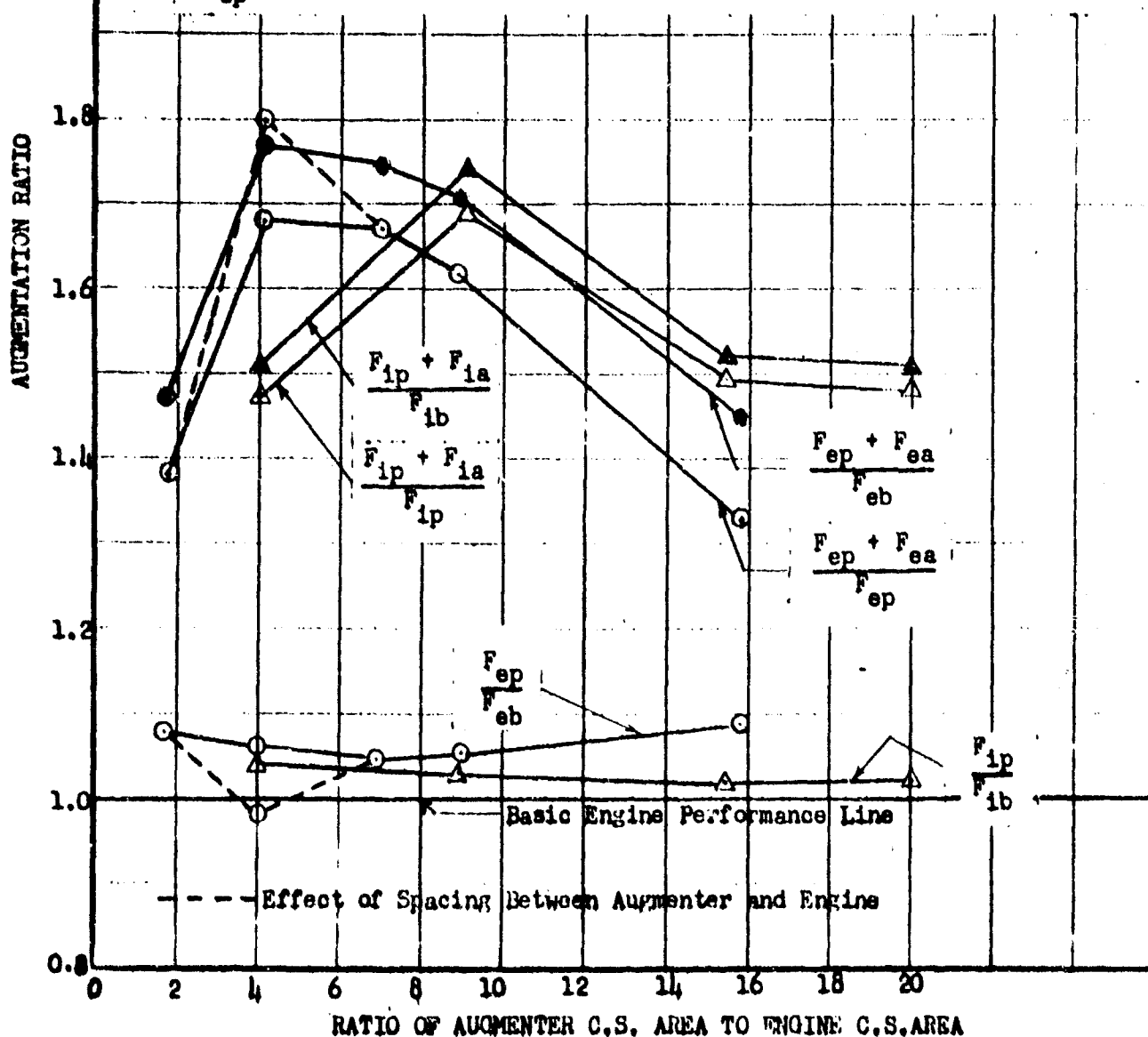
FIGURE 15: PERFORMANCE OF CYLINDRICAL AUGMENTERS
