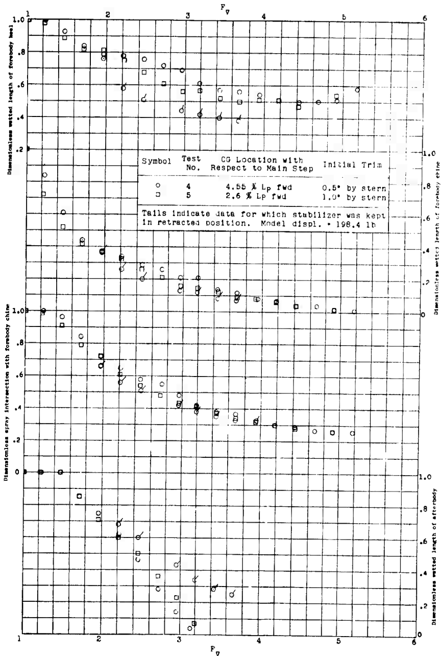
Figure 12 - Wetted Lengths for Model 4461-3 at Two CG Positions, A_p/v^{3/2} = 6.05
