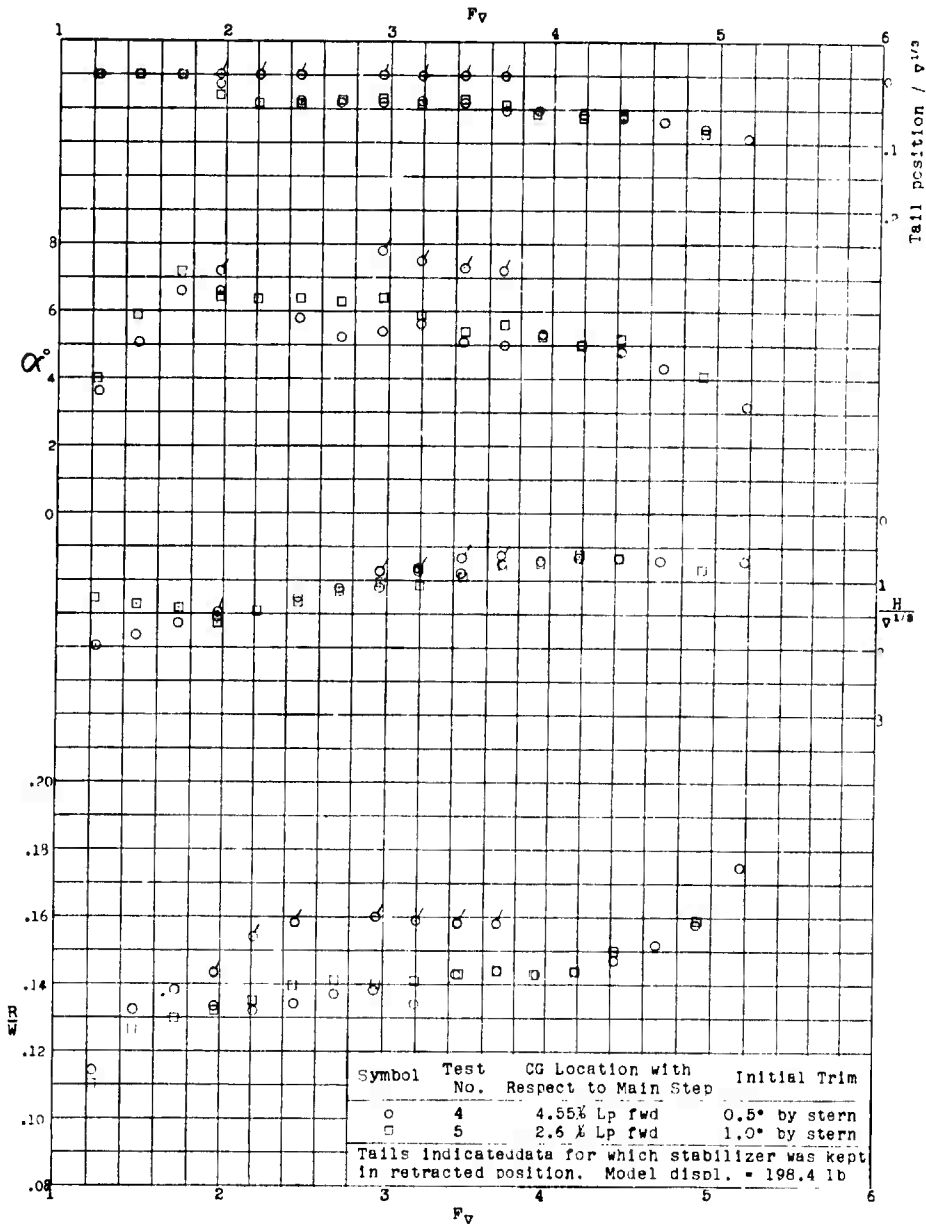
Figure 10 - Resistance, Draft, \alpha , and Stabilizer Position for Model 4461-3 at Two LCG Positions, A_p/v^{2.0} = 6.05
