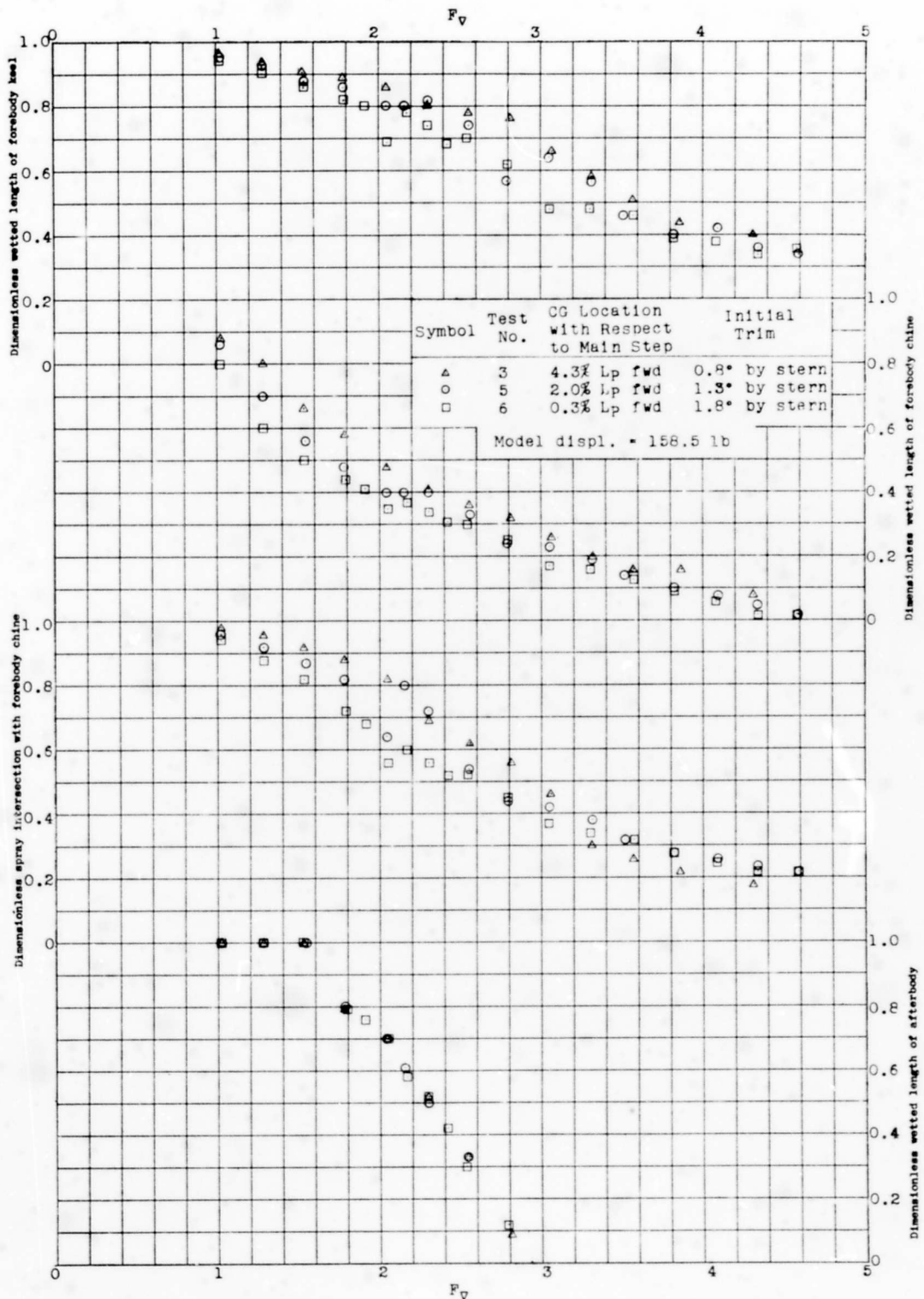
Figure 8 - Wetted Lengths for Model 4335-1 at Three LCG Positions, A_p/V^2 = 7.0
