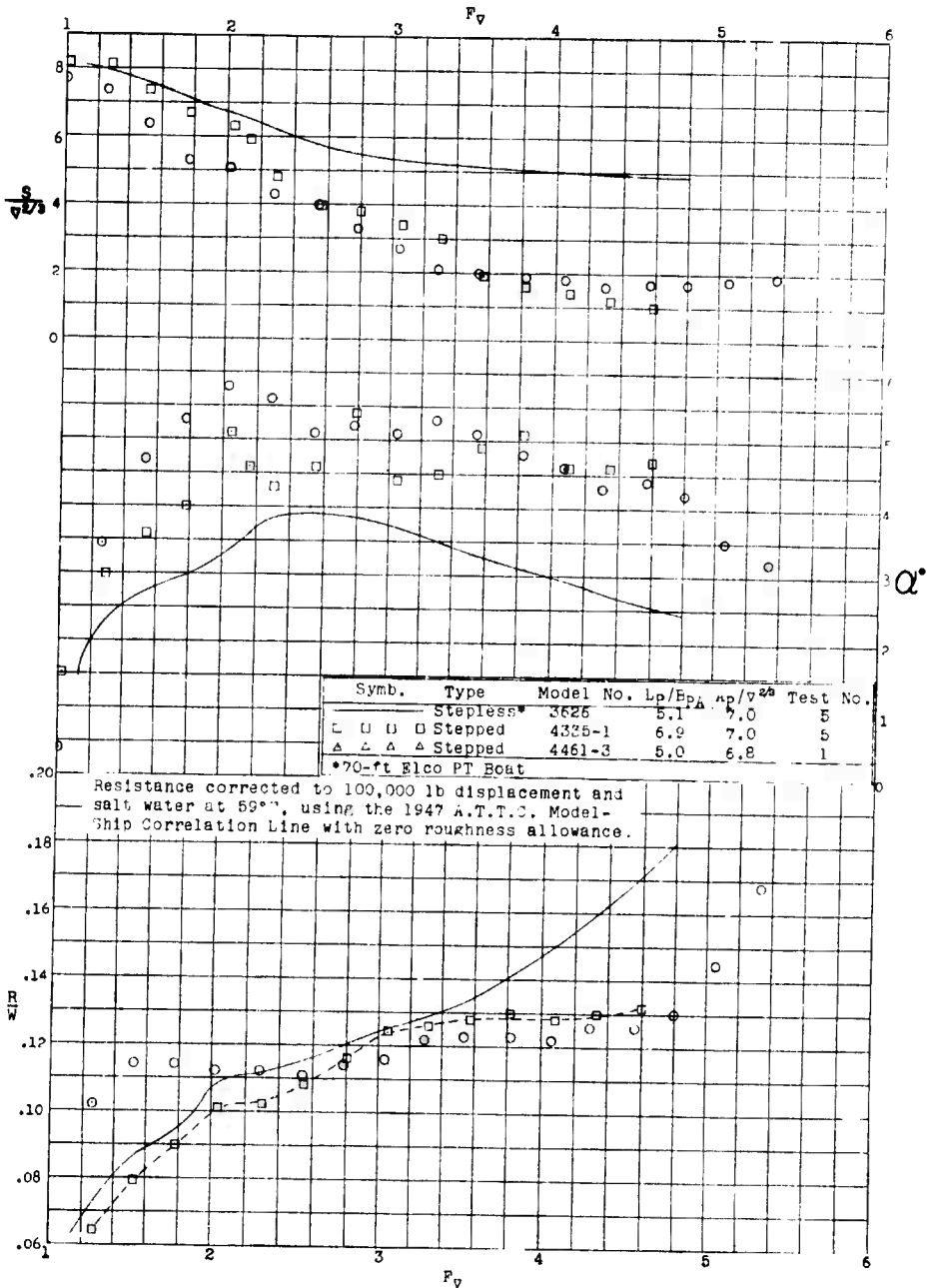
Figure 14 - Comparison of Resistance, \alpha , and Wetted Surface for the Two Stepped Hulls and a Conventional Planing Boat Design
