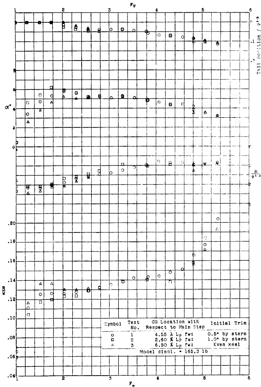
Figure 9 - Resistance, Draft, \alpha , and Stabilizer Position for Model 4461-3 at Three LCG Positions, Ap/v^2 = 6.84
