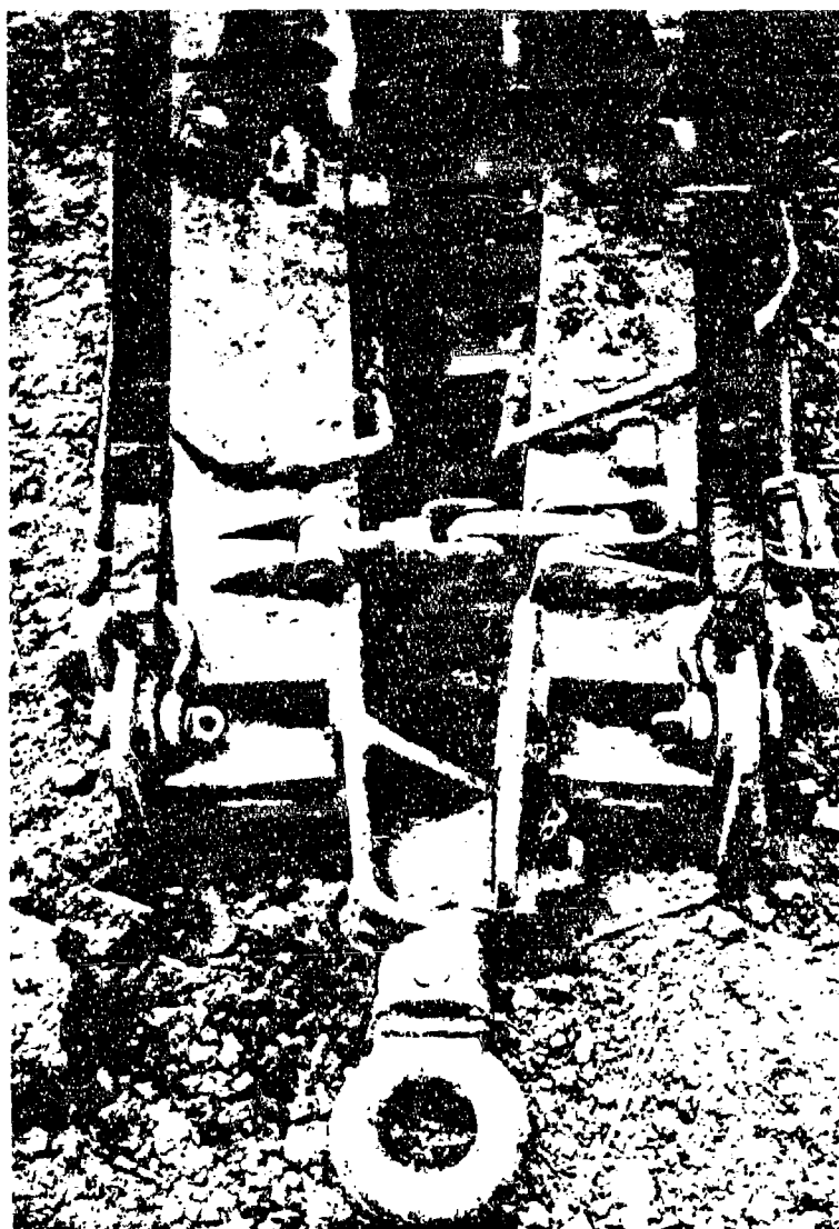
FIGURE 3. The sixteen foot sling legs attached to trails of 155mm howitzer. These legs are attached after the placement of the 9 foot legs under the tube.
