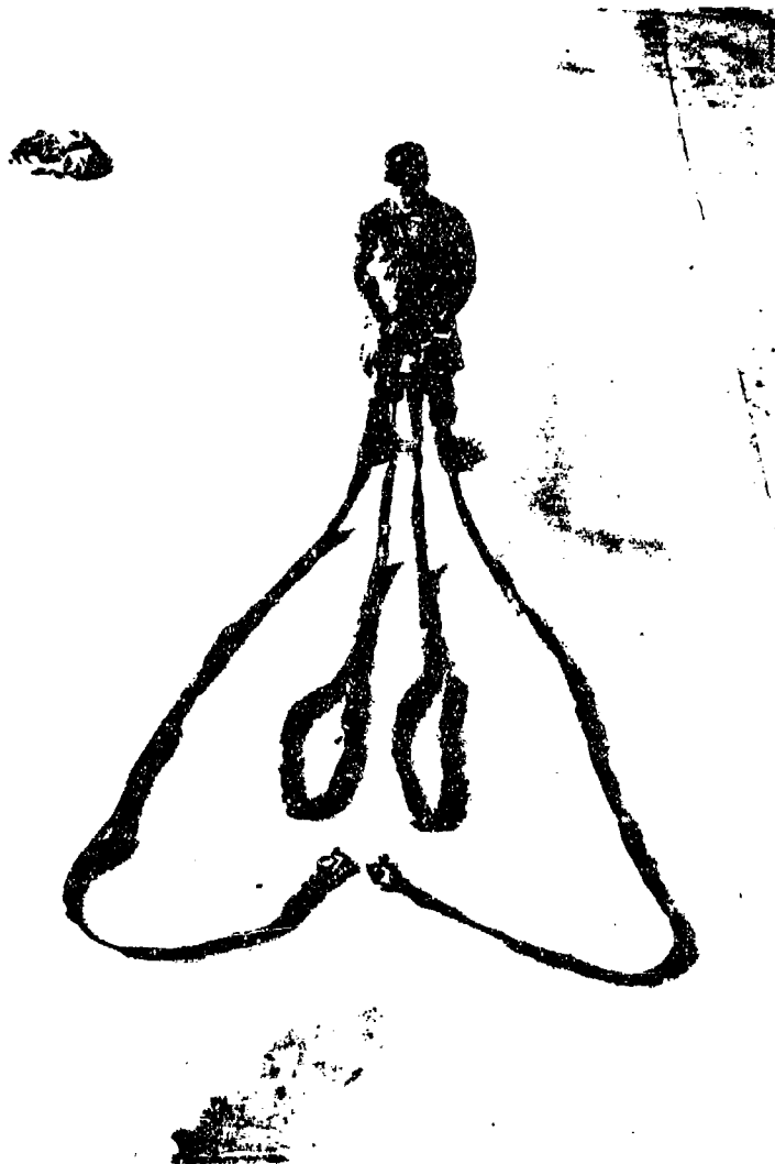
FIGURE 1. The complete sling for lifting the 155mm howitzer by CH-47 (Chinook) consists of a donut (held by Pathfinder) and four sling legs. Each sling leg is rated at 13,500 lbs strength. Two of the legs are 16 feet long and have a medium clevis attached to each, the other two legs are 9 feet in length and are insulated and taped to prevent friction damage.
