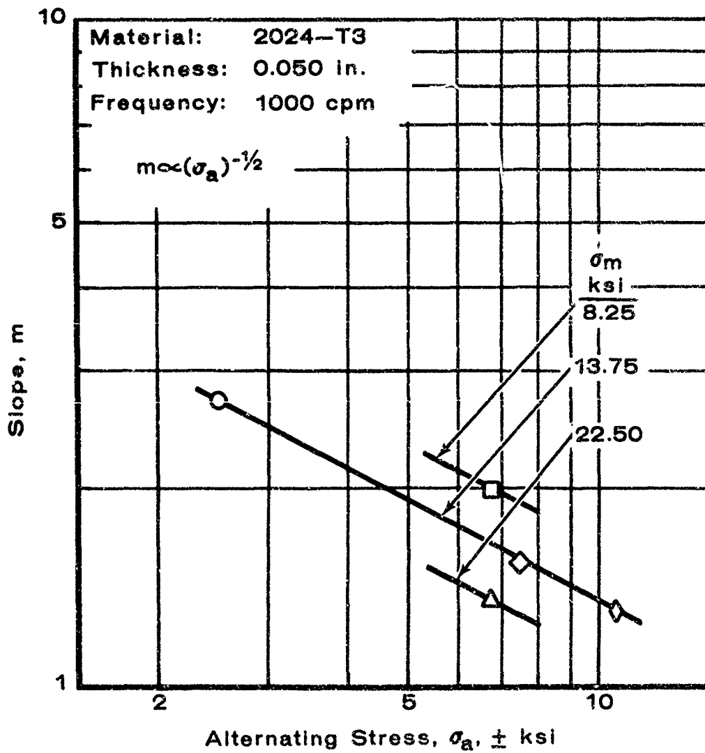
Figure 18. Effect of Alternating Stress on Slope, m
