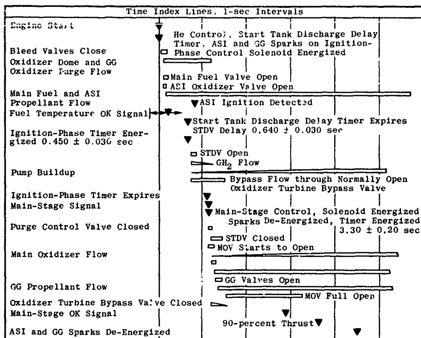
a. Start Sequence
