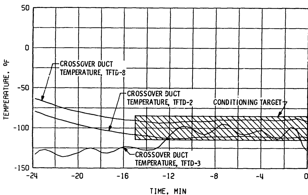
b. Turbines and Crossover Duct
