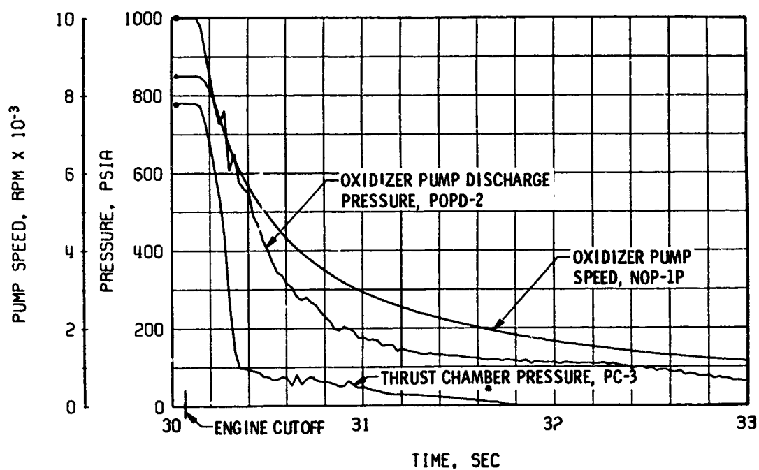
d. Thrust Chamber Oxidizer System, Cutoff Fig. 12 Continued
