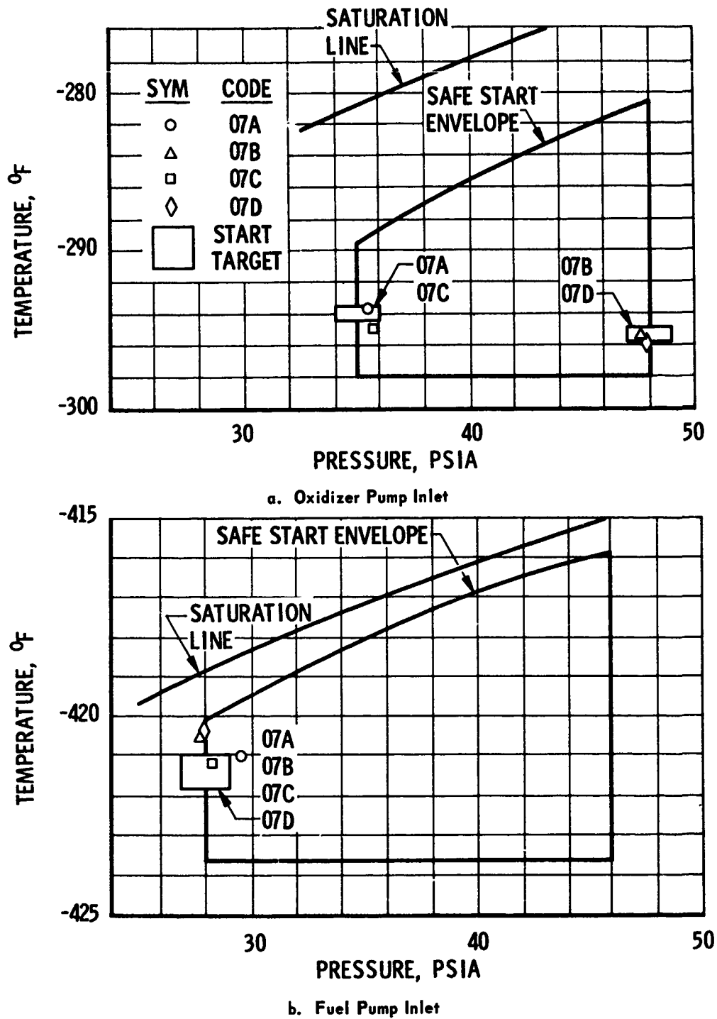
Fig. 8 Engine Start Conditions for Pump Inlets, Starr Tank, and Helium Tank
