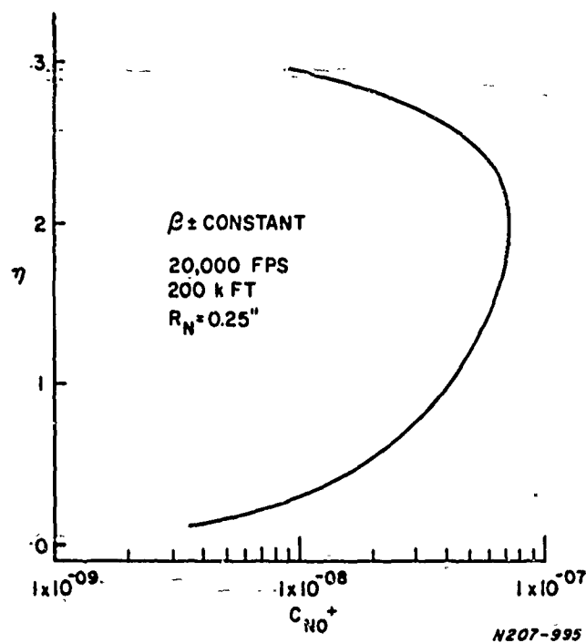
Figure 5. \text{NO}^+ , Stagnation Point
