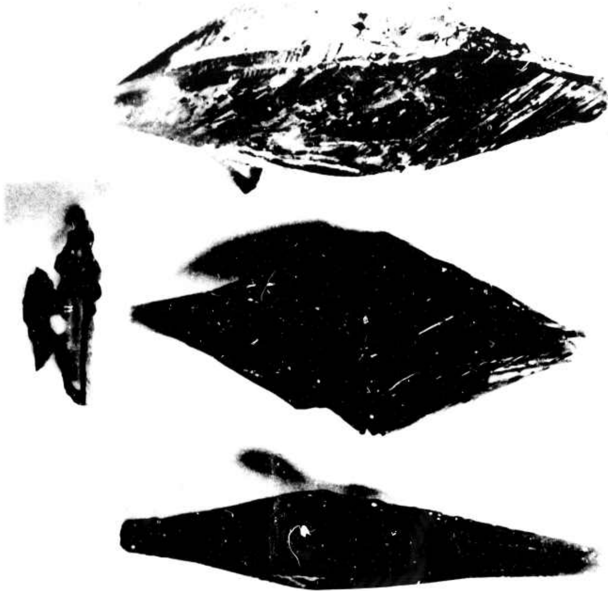
Figure 2: Rubies Grown Simultaneously in Horizontal "Cross Flow" Furnace.
