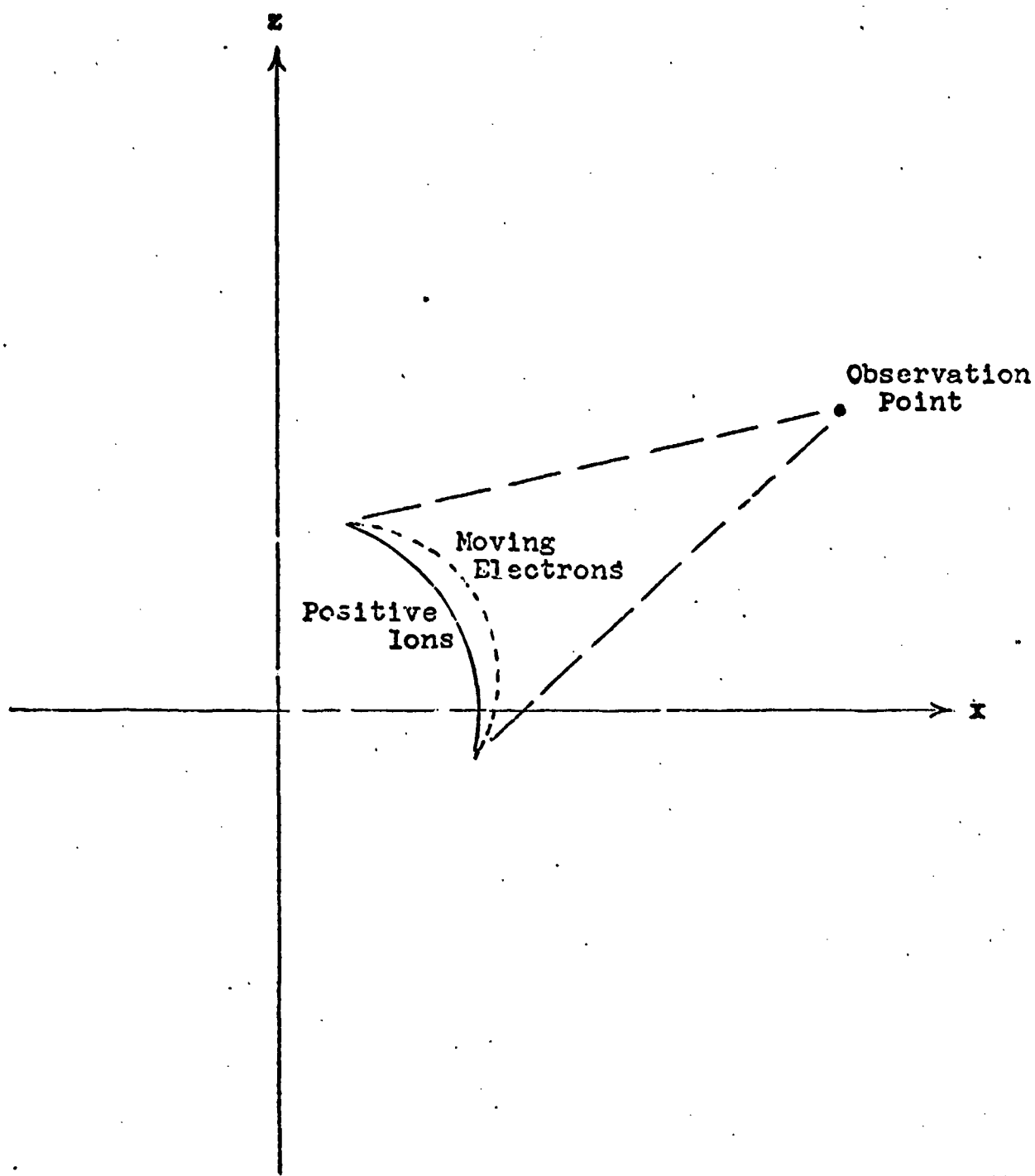
Figure 1. The shell model, as seen from the observation point at an early instant, before any of the stopped electrons (negative ions) can be seen.
