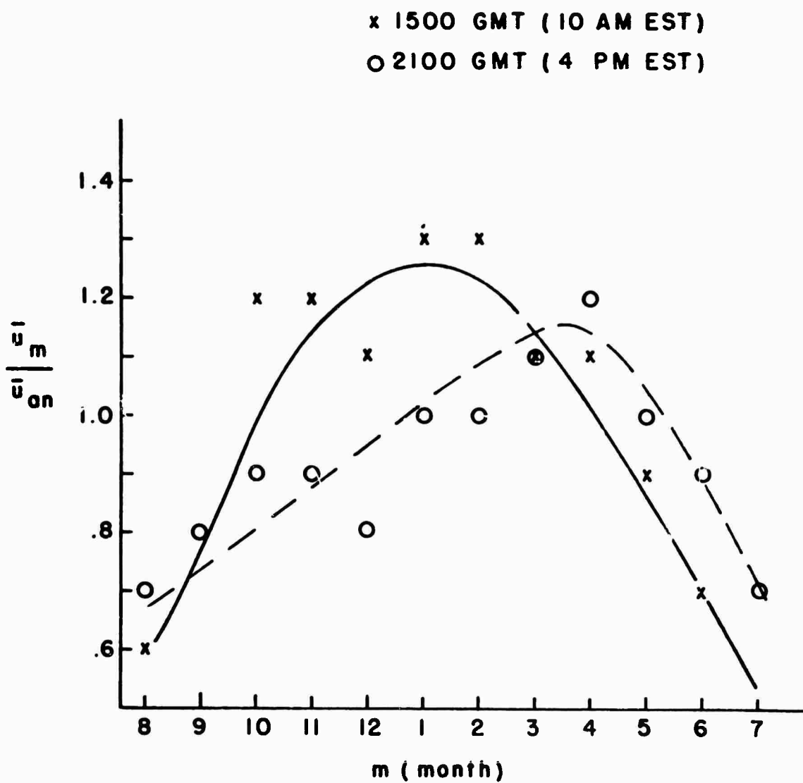
FIG. 16. MONTHLY-TO-YEARLY CLIMATIC-WIND-SPEED RATIOS AT 300 M FOR UNSTABLE CONDITIONS OVER SMOOTH TERRAINS (FOR 1500 AND 2100 LST).
