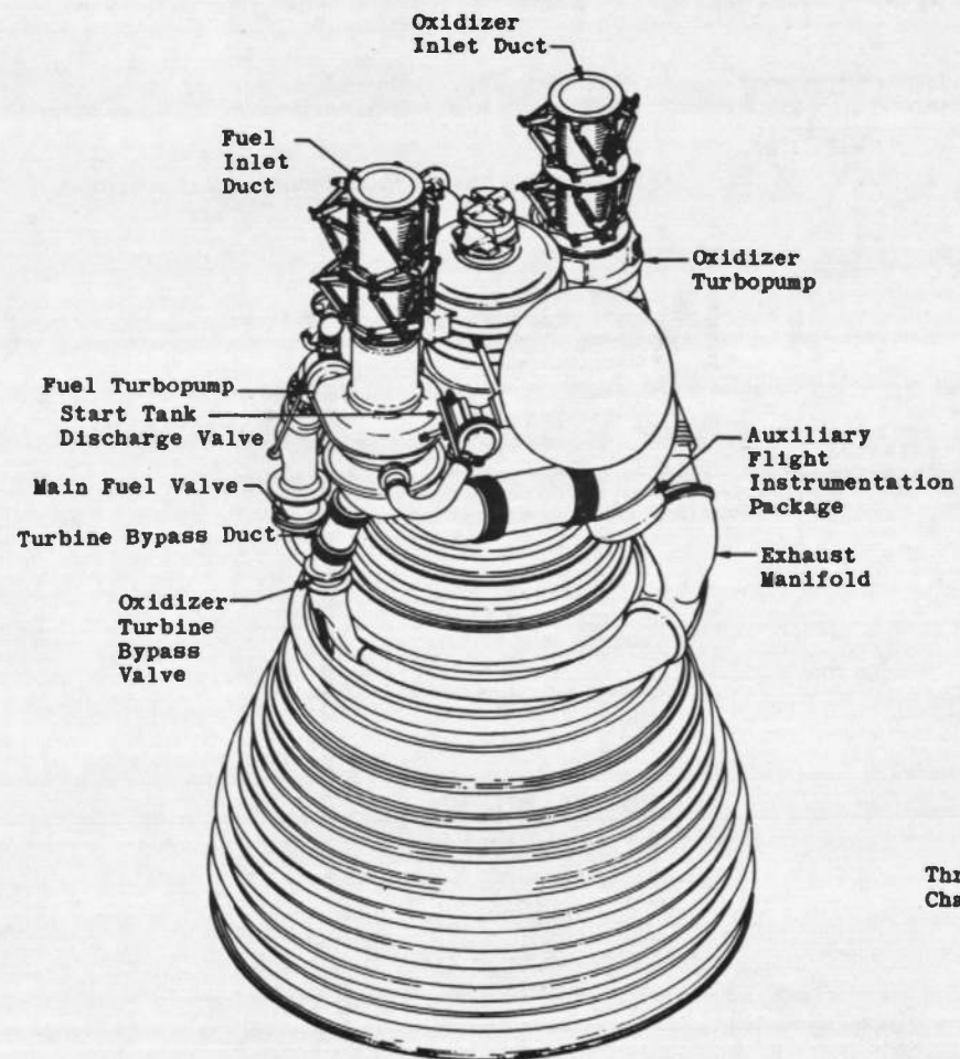
Fig. 3 Engine Details
