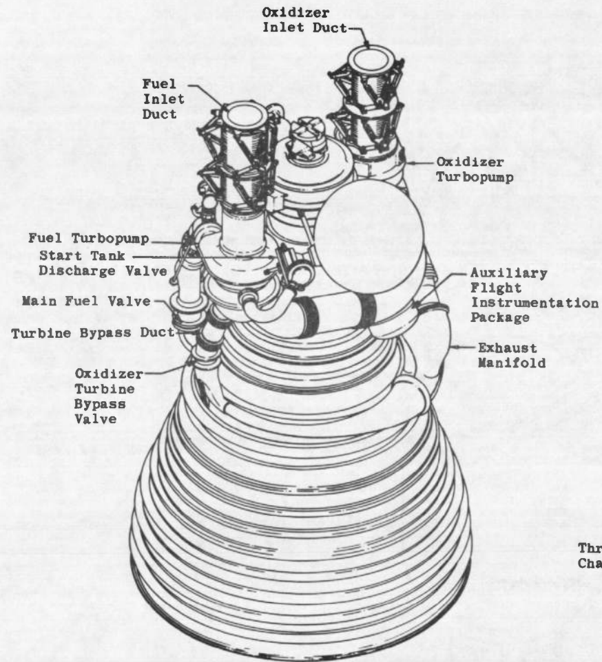
Fig. 3 Engine Details
