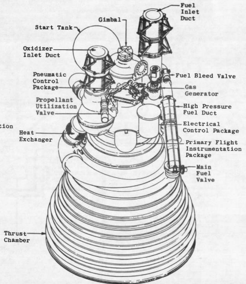
Fig. 3 Engine Details
