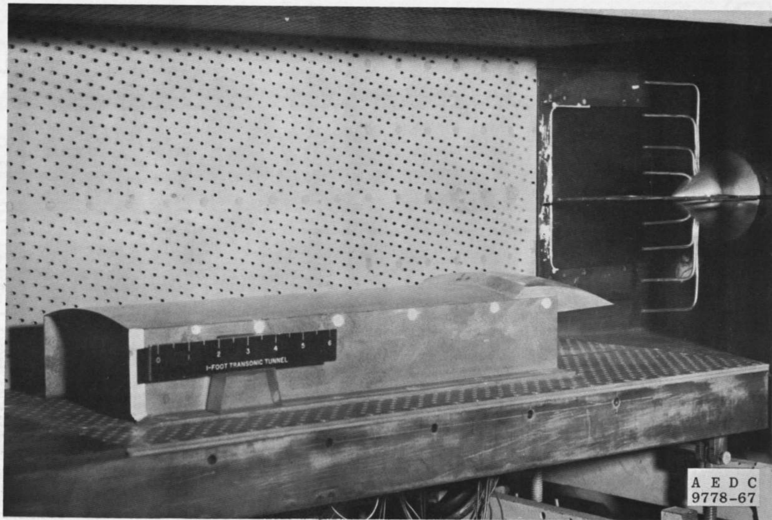
b. Configuration h_2 + BT_1
