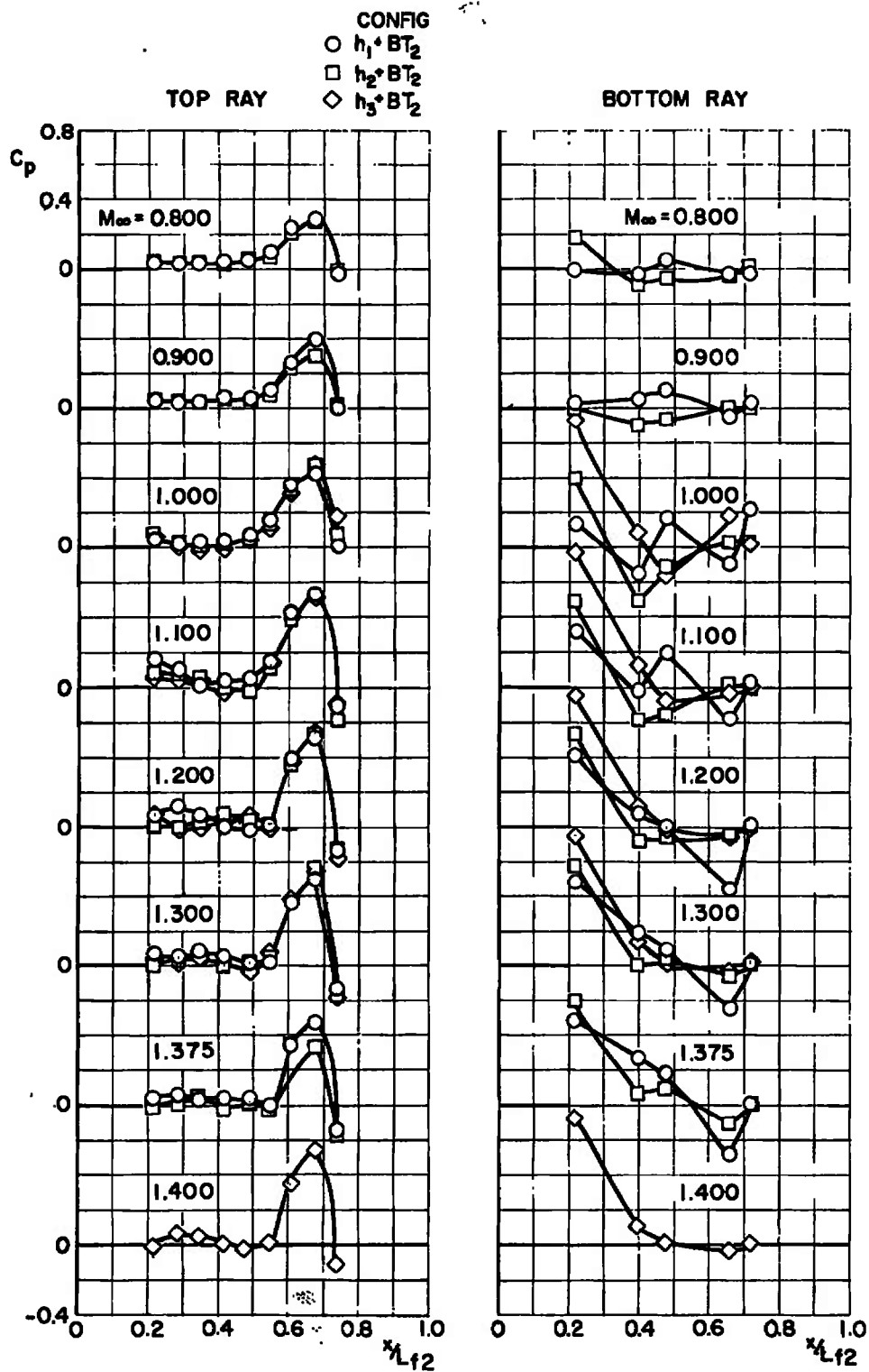
b. Boottail Configuration BT_2
