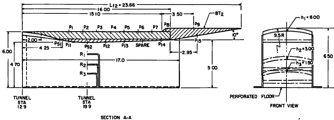
b. Configurations h_1 , h_2 , h_3 , and BT_2 Fig. 5 Concluded
