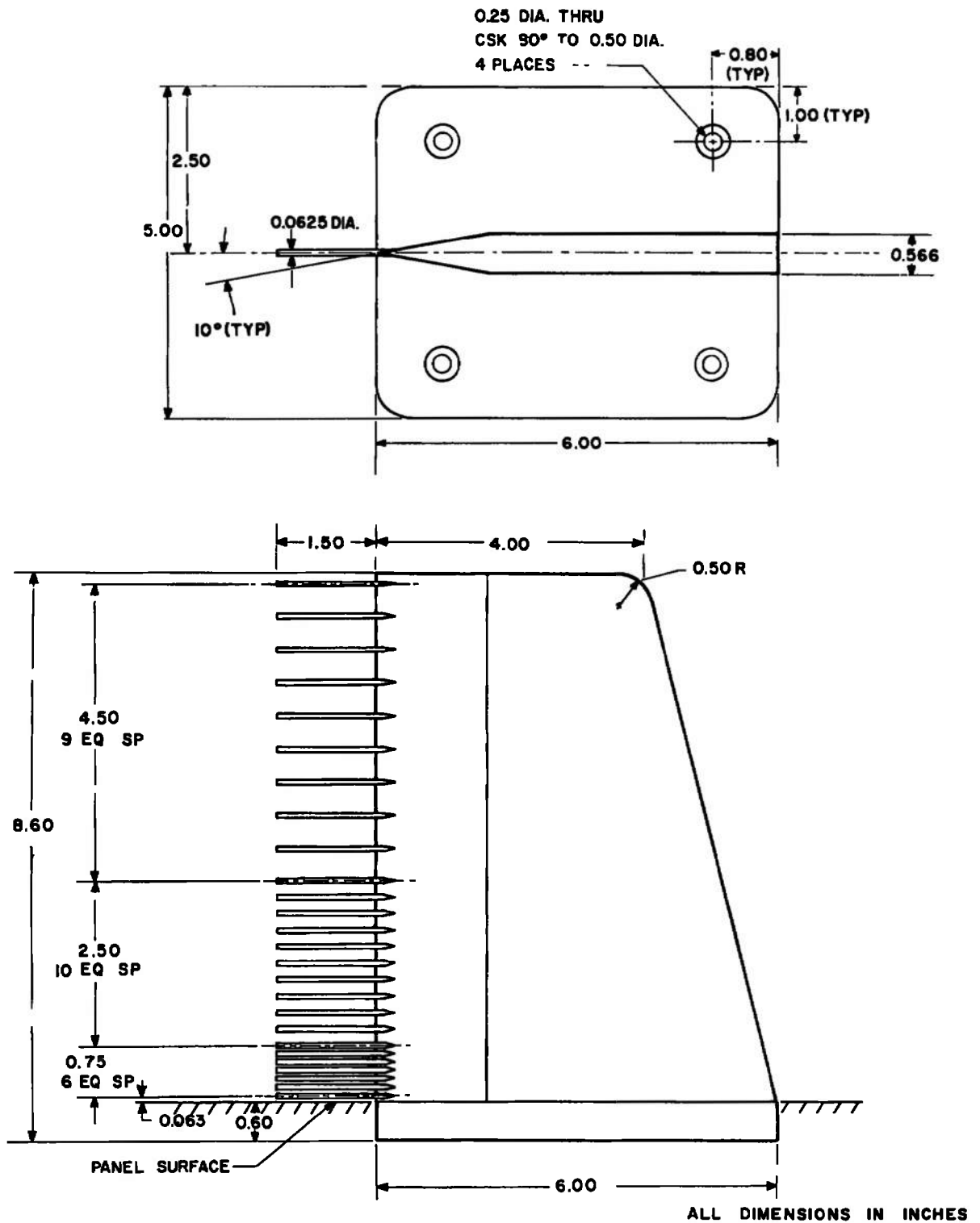
Fig. 8 Boundary-Layer Rake
