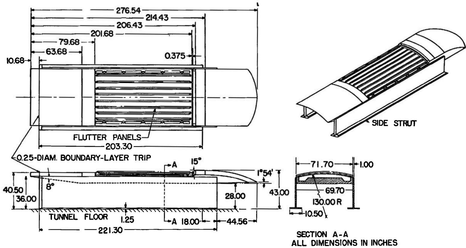
Fig. 7 Details of Test Fixture with Flutter Panel Installed
