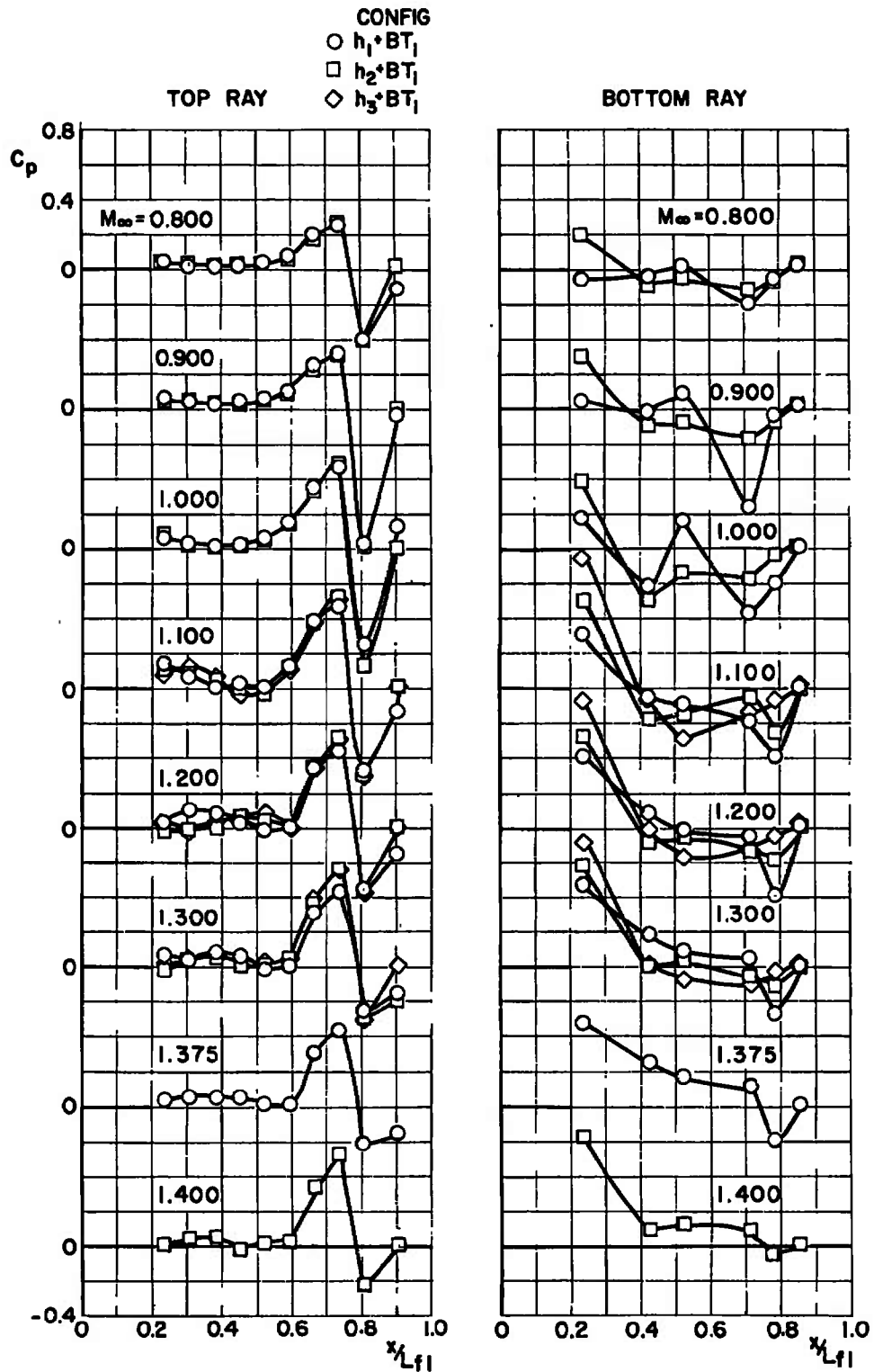
Fig. 13 Variation of Pressure Coefficient along the Calibration Model
