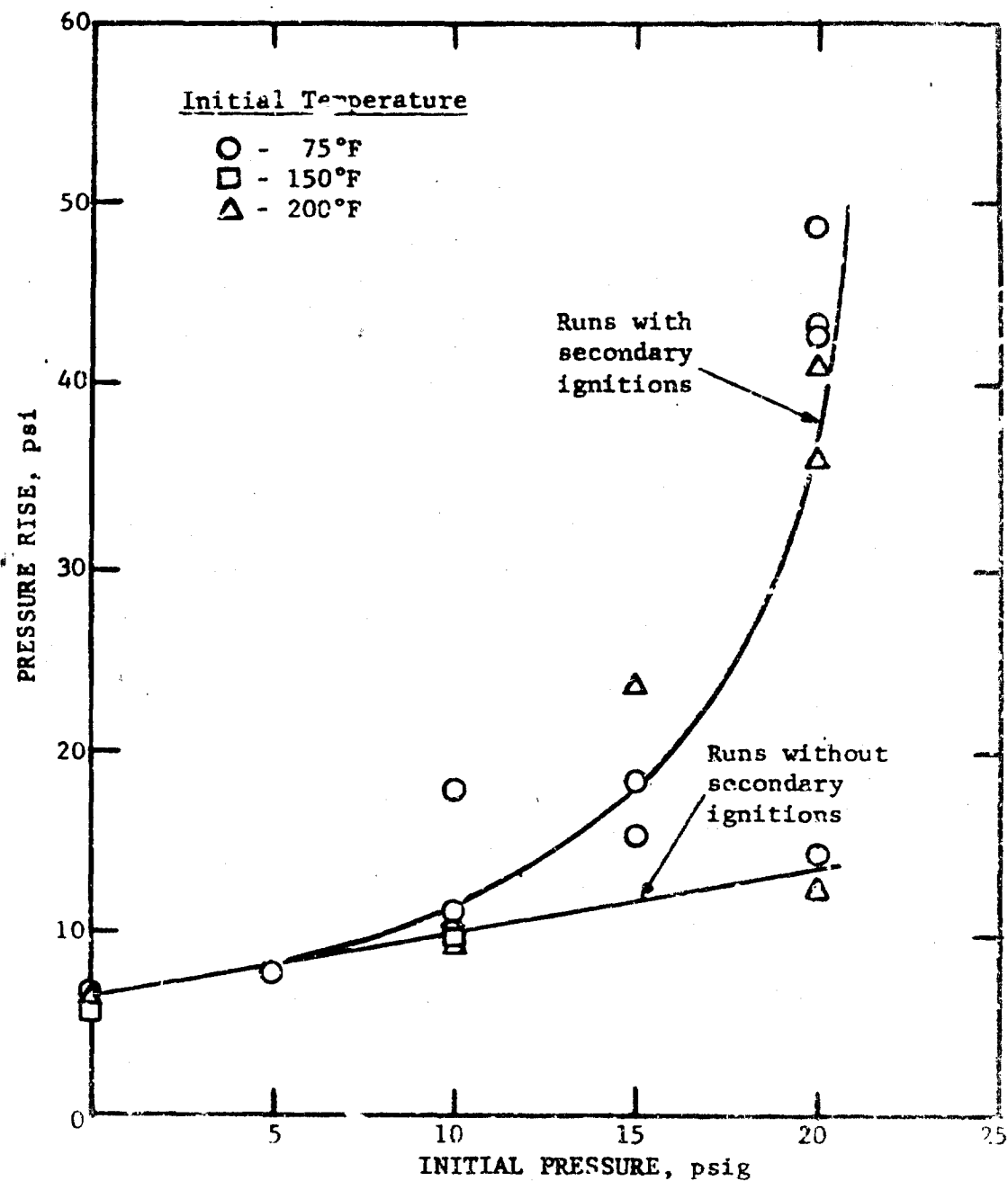
FIGURE 7. - Pressure rise vs initial pressure for experiments with arrestor material A (20 pores/inch) and ~2.5 percent n-pentane-air mixtures at various initial temperatures. Arrestor length/ignition void length = 30"/18"; 1 ft 3 cylindrical steel vessel (6" diameter and 60" length).
