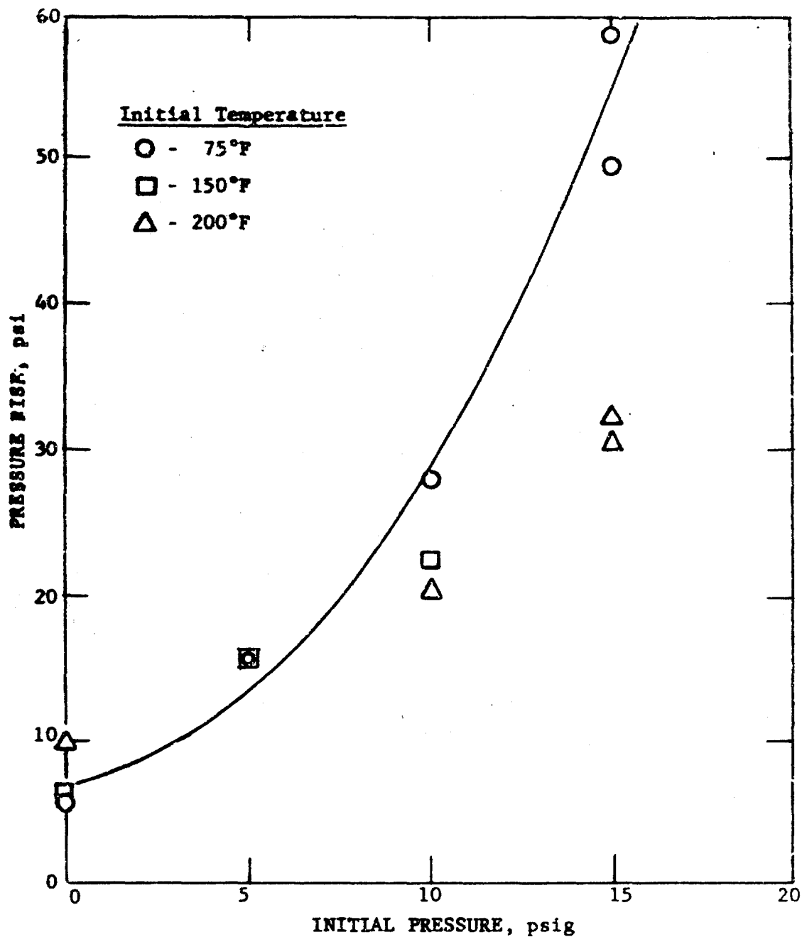
FIGURE 6. - Pressure rise vs initial pressure for experiments with arrestor material A (10 pores/inch) and \sim 2.5 percent n-pentane-air mixtures at various initial temperatures. Arrestor length/ignition void length = 30"/18"; 1 ft 3 cylindrical steel vessel (6" diameter and 60" length).
