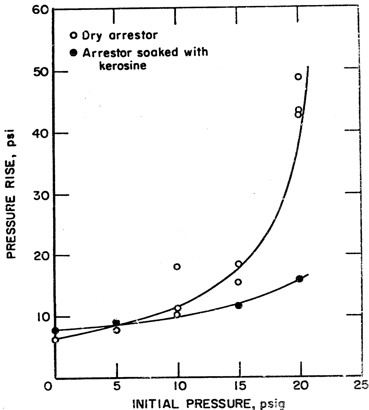
FIGURE 5. - Effect of initial pressure on pressure rise in experiments with wet and dry arrestor material A (20 pores/inch) and ~2.5 percent n-pentane-air mixtures. Arrestor length/ignition void length = 30"/18"; 1 ft 3 cylindrical steel vessel (6" diameter and 60" length).
