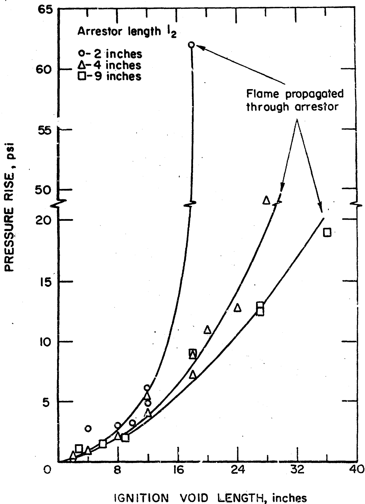
FIG. 8. - Effect of ignition void length on pressure rise in experiments with 2, 4, and 9-inch segments of the 20 pores/inch arrestor material A and ~2.5 percent n-pentane-air mixtures at atmospheric pressure; 1 ft 3 cylindrical steel vessel (6" diameter and 60" length).
