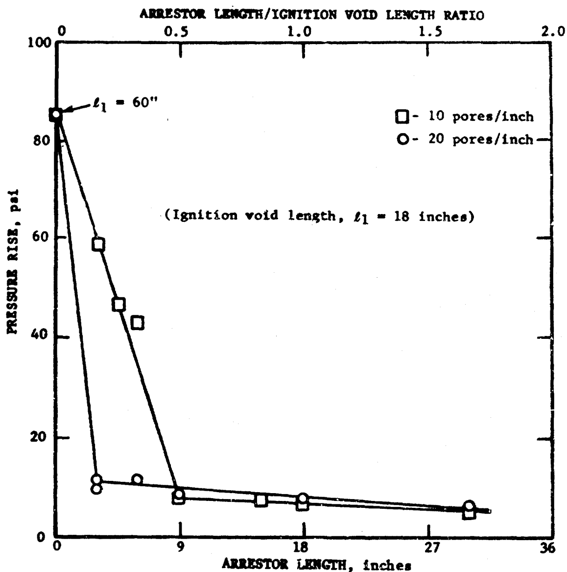
FIGURE 3. - Effect of arrestor length on pressure rise in experiments with 10 and 20 pore/inch arrestor material A and \sim 2.5 percent n-pentane-air mixtures at 0 psig; 1 ft 3 cylindrical steel vessel (6" diameter and 60" length).
