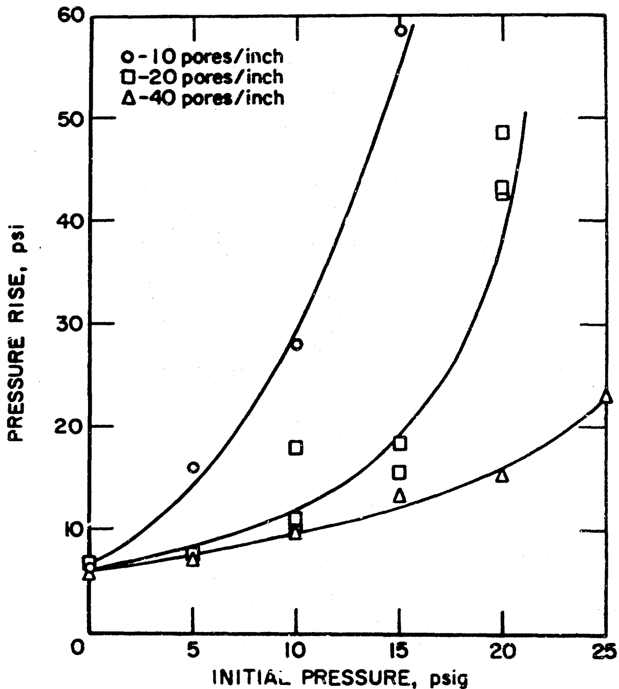
FIGURE 4. - Effect of initial pressure on pressure rise in experiments with 10, 20 and 40 pores/inch arrestor material and ~2.5 percent n-pentane-air mixtures. Arrestor length/ignition void length = 30"/18"; 1 ft 3 cylindrical steel vessel (6" diameter and 60" length).
