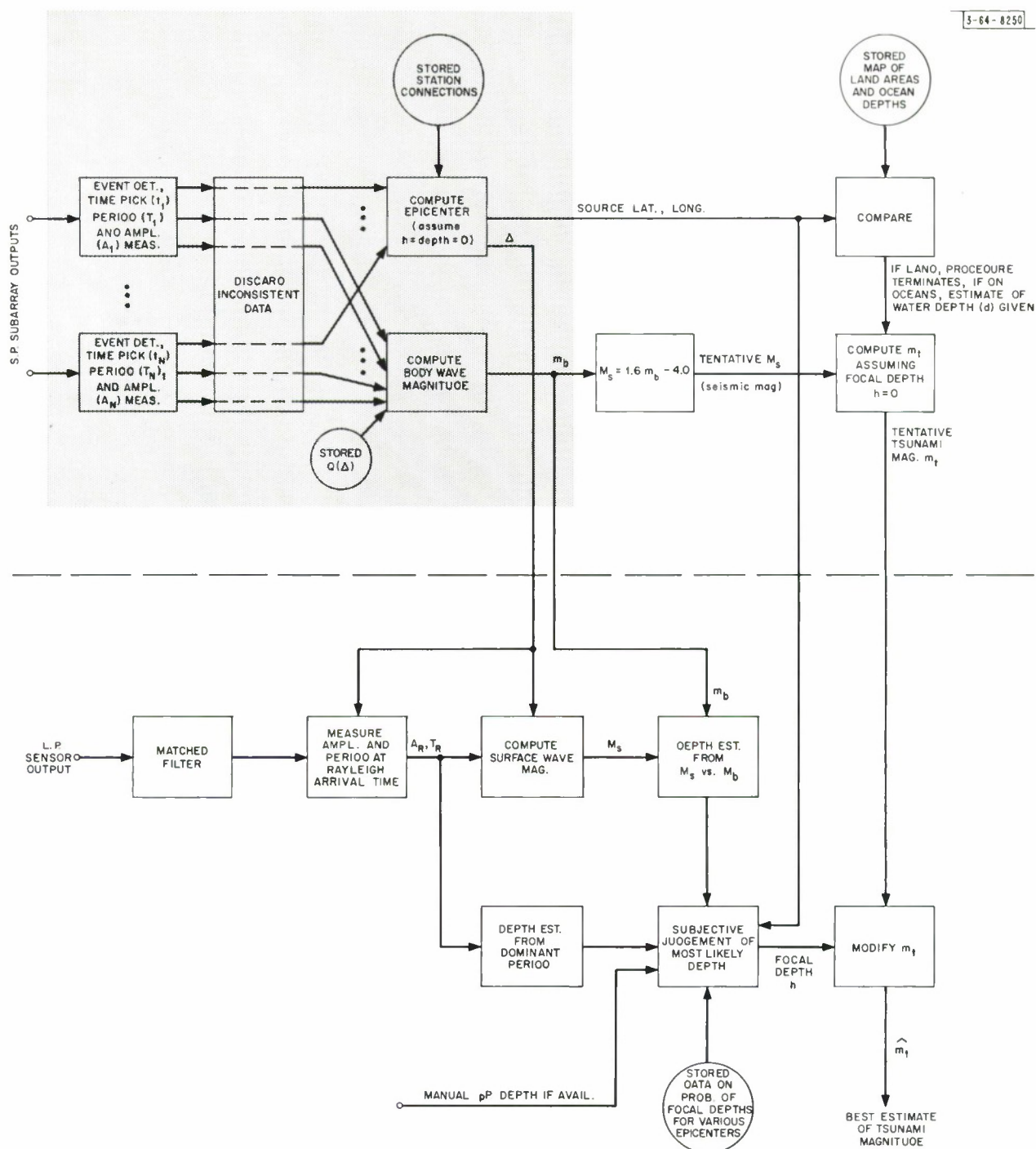
Fig. 11. Flow diagram of the sequence of large array signal handling operations for generating tsunami warning information. (Shaded area indicates currently employed station bulletin program.)
