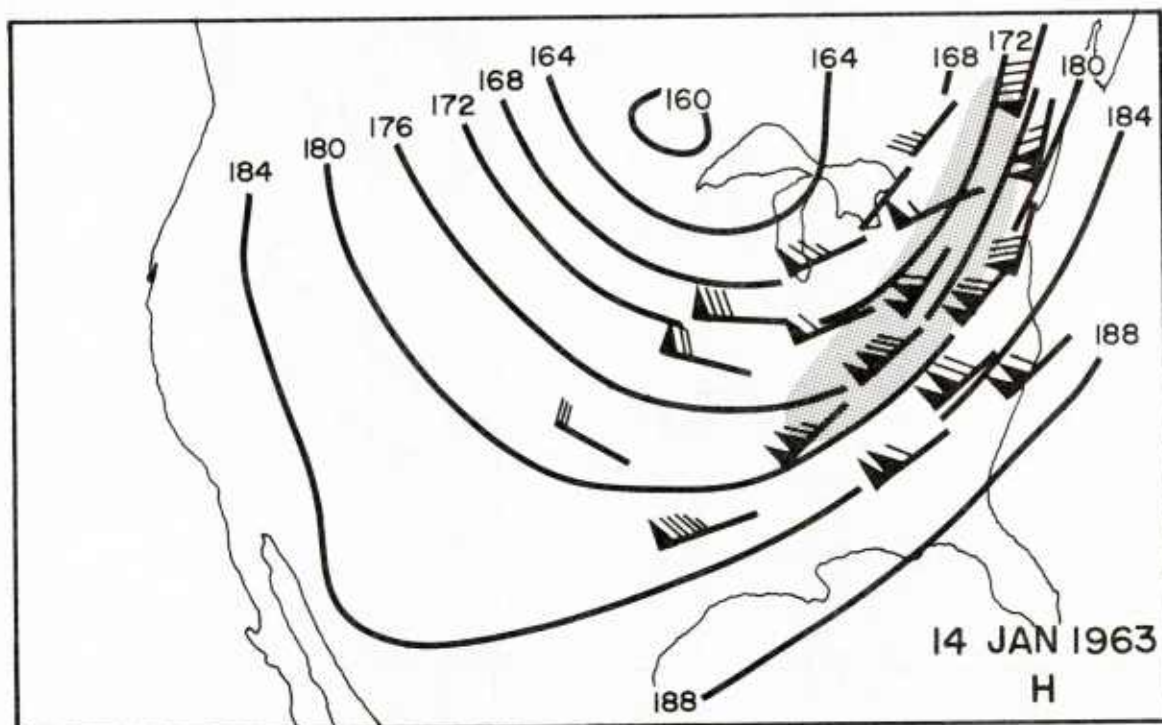
Figure 3.6. 500-mb. Contours (100's of feet) and Winds on 14 January 1963, 0000 GMT, In and Near Area with Critical Temperature Gradient.
