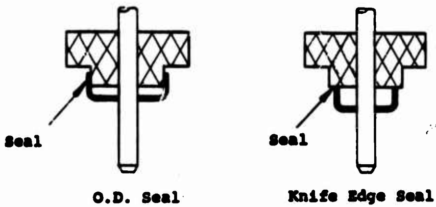
Figure 3. Knife Edge Seal vs. No Knife Edge Seal
