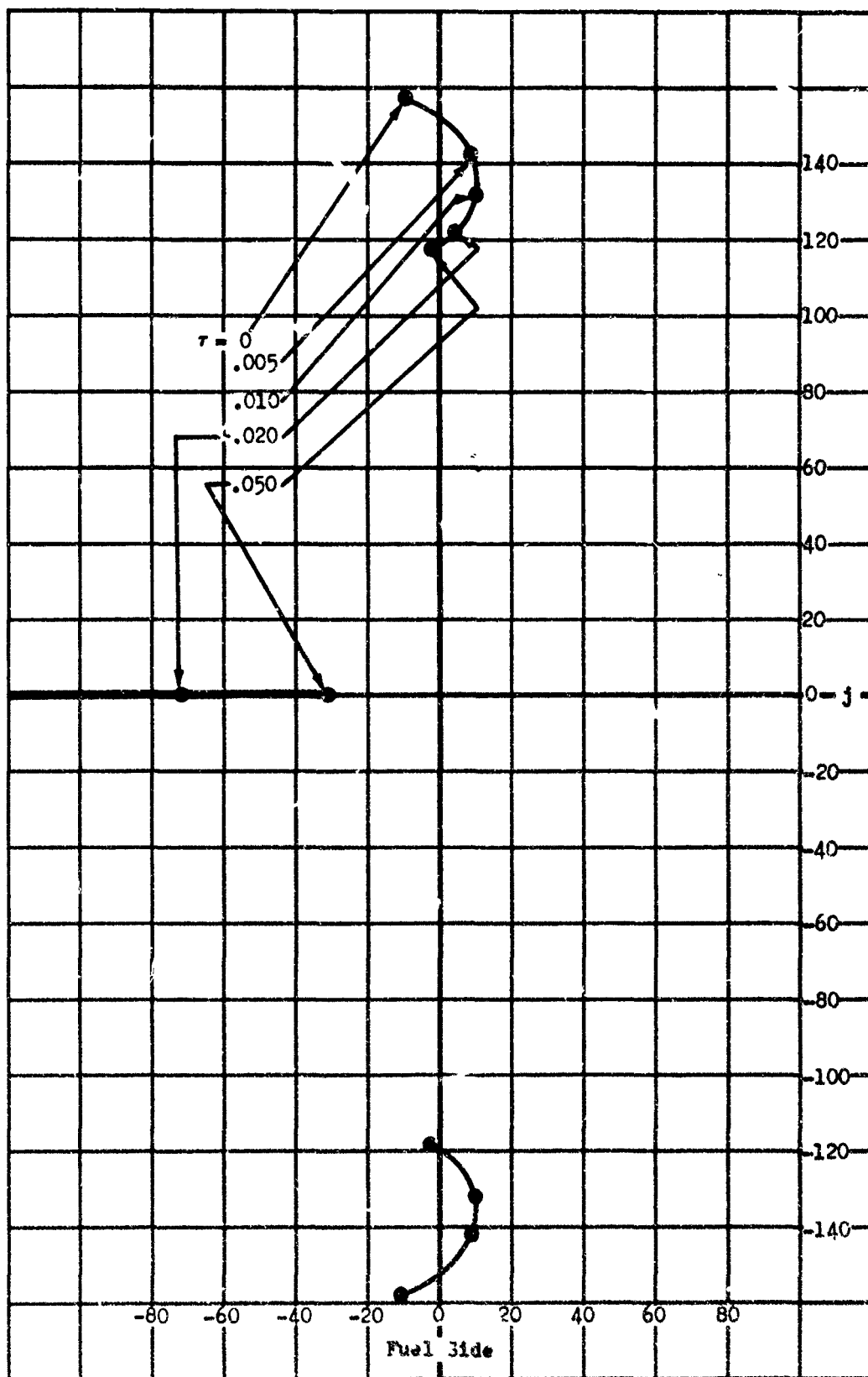
Figure 17 P_s/g_G Poles in "S" Plane - A_{Gf} = -50
