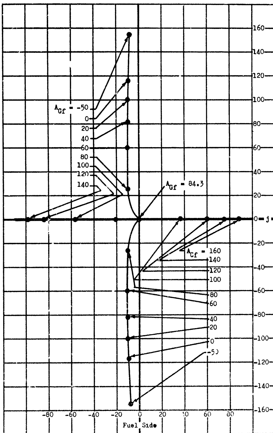
Figure 16 P_s/g_G Poles in "S" Plane -\tau = 0
