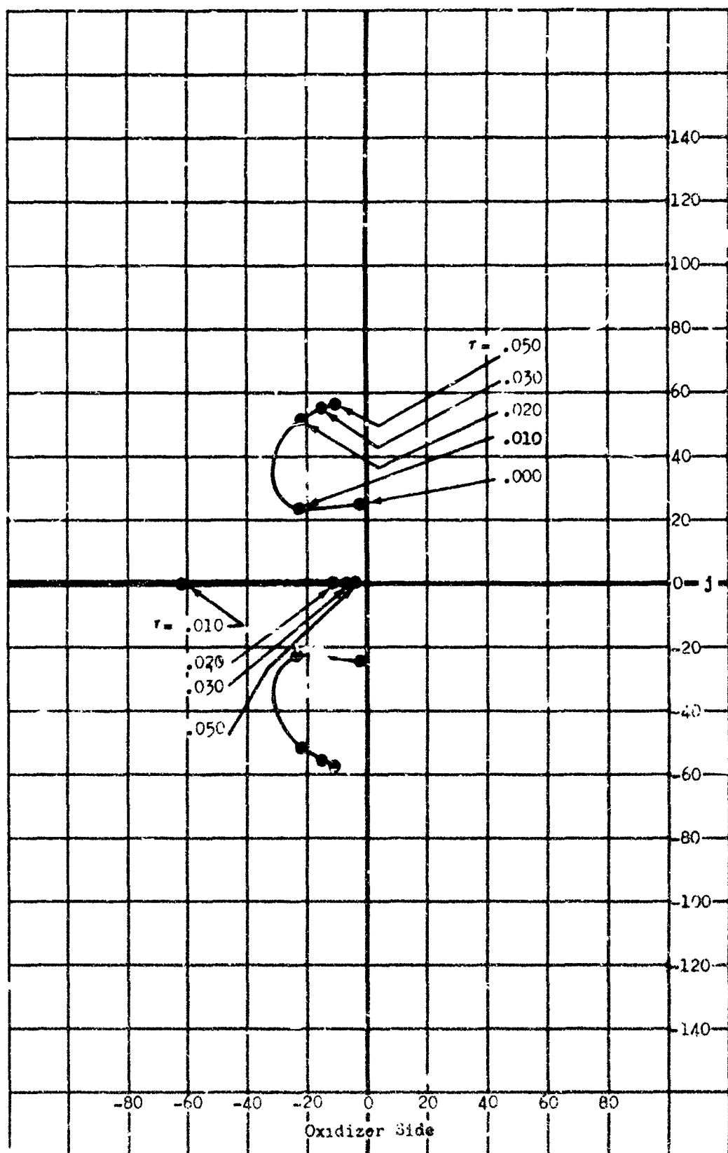
Figure 15 P_s/g_a Poles in 3 rd Plane - A_{00} = 50
