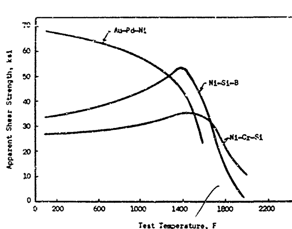
FIGURE 1. PROPERTIES OF BRAZED JOINTS IN RENÉ 41 (8)
