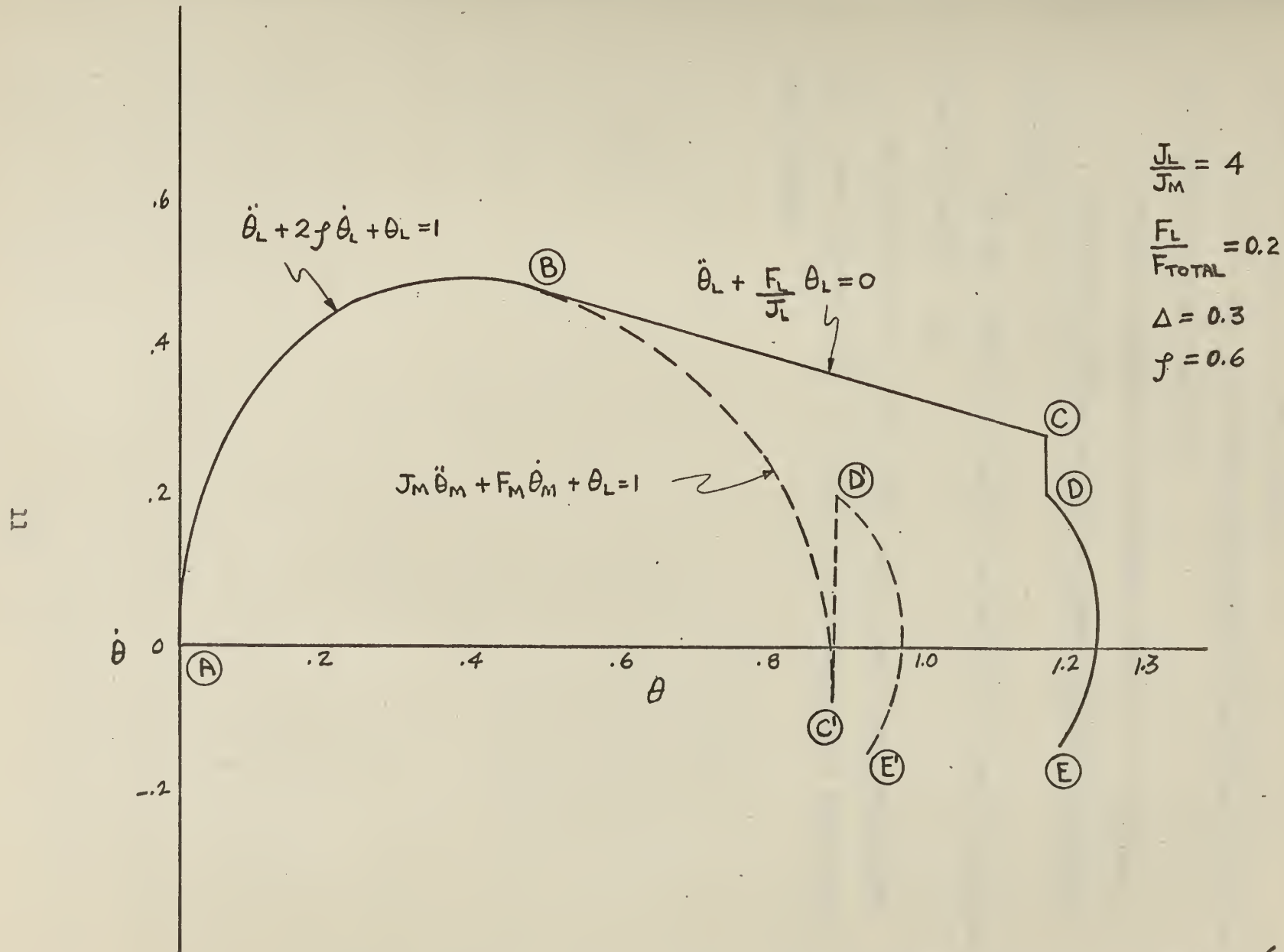
FIG. 4 PHASE TRAJECTORY FOR SHOWING BACKLASH EFFECTS (EXAMPLE 2)
