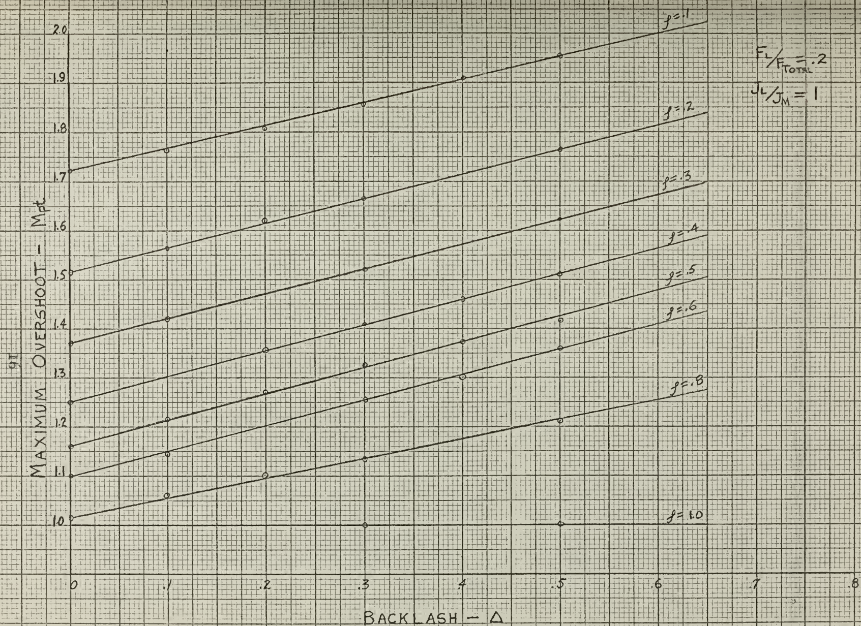
FIG. 5 MAXIMUM OVERSHOOT VS. BACKLASH FOR FRICTION RATIO OF .2 AND J_L/J_M OF 1.0
