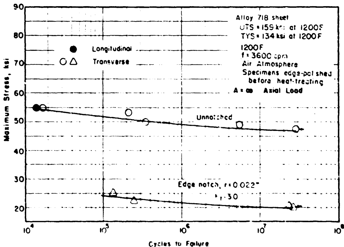
S-N DIAGRAM FOR ALLOY 718 SHEET AT 1200 F WITH STRESS RATIO, A = - (unnotched and edge-notched)
