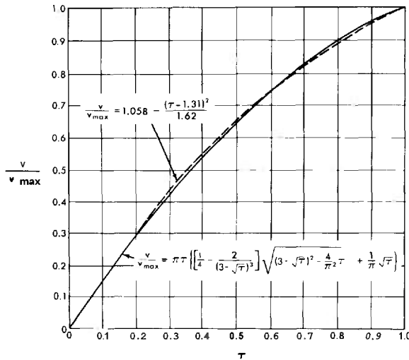
FIGURE 3-97. CANOPY VOLUME DURING INFLATION
