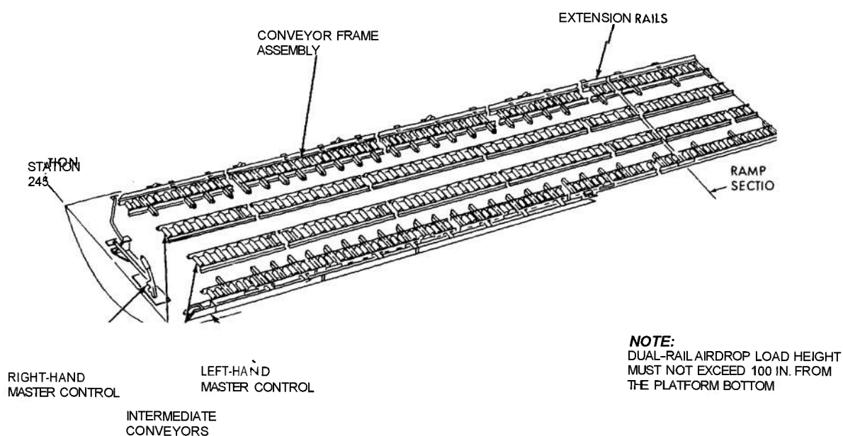
FIGURE 3-22. MODEL AF/A32H-1A DUAL-RAIL SYSTEM COMPONENTS
