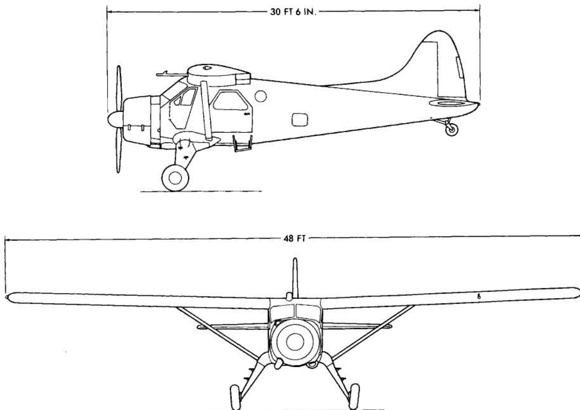
FIGURE 4-105. U-6A AIRCRAFT
