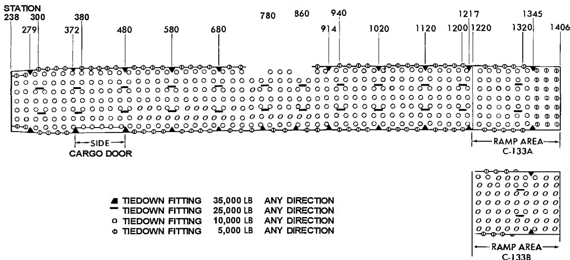
FIGURE 4-72. ANCHORING ARRANGEMENT, C-133 AIRCRAFT
