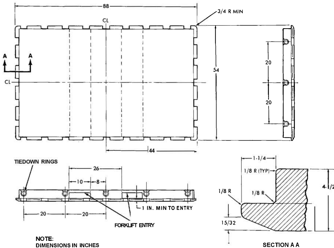
FIGURE 2-78. HCU-10/C CARGO PALLET
