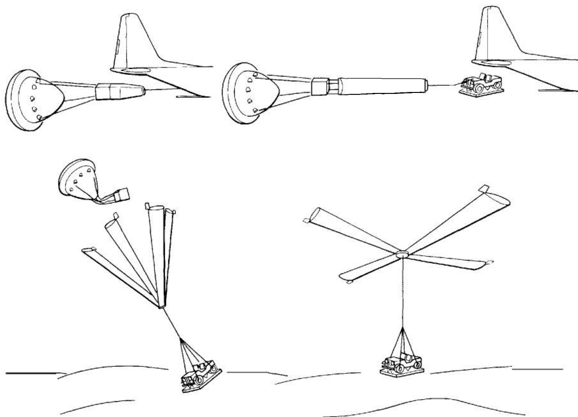
FIGURE 3-8. ROTATING DECELERATORS
