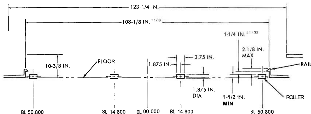
FIGURE 3-25. INTEGRAL SUBSYSTEM CARGO HANDLING SYSTEM (C-141)
