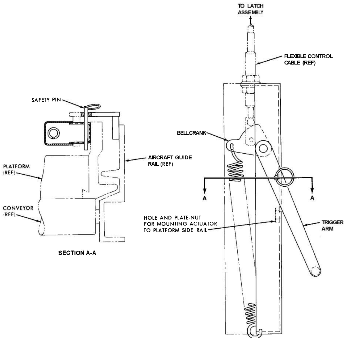
FIGURE 3-54. ACTUATOR ASSEMBLY
