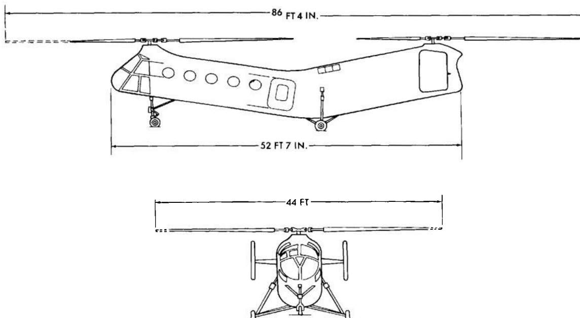
FIGURE 4-111. CH-21 HELICOPTER
