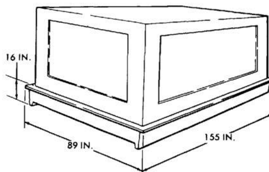
FIGURE 4-60. LOADING WELL CLEARANCE, C-124 AIRCRAFT
