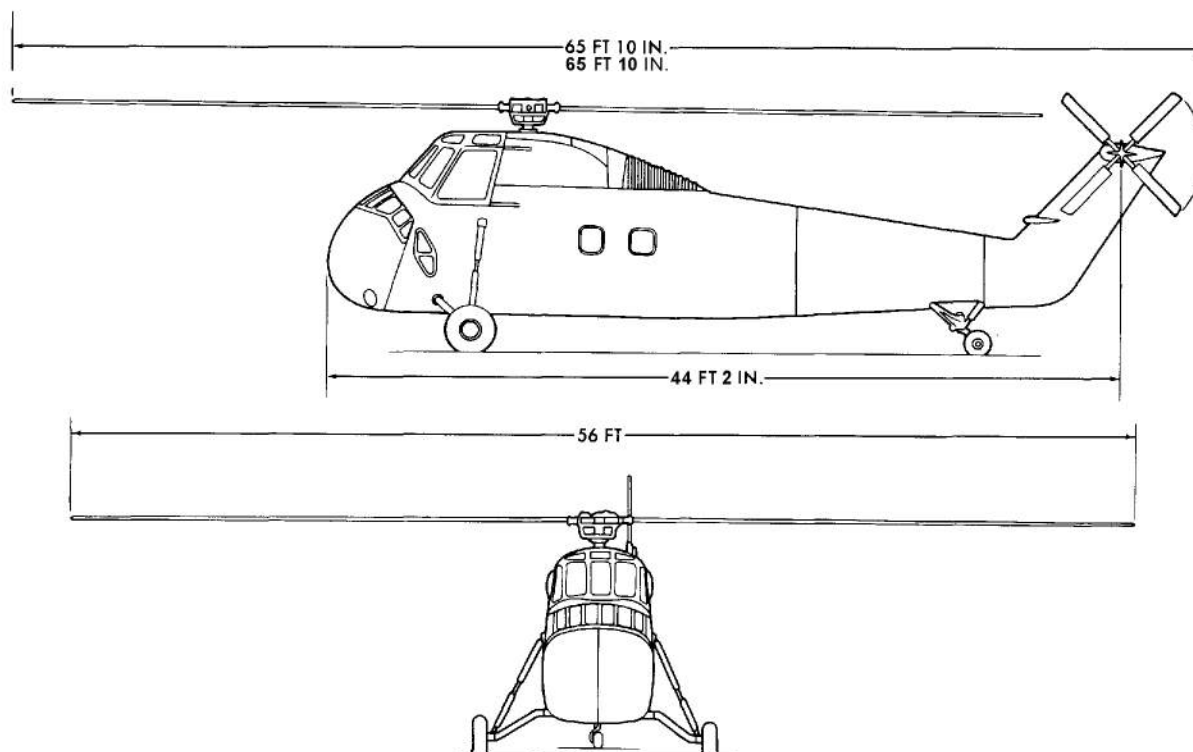
FIGURE 4-115. CH-34 HELICOPTER
