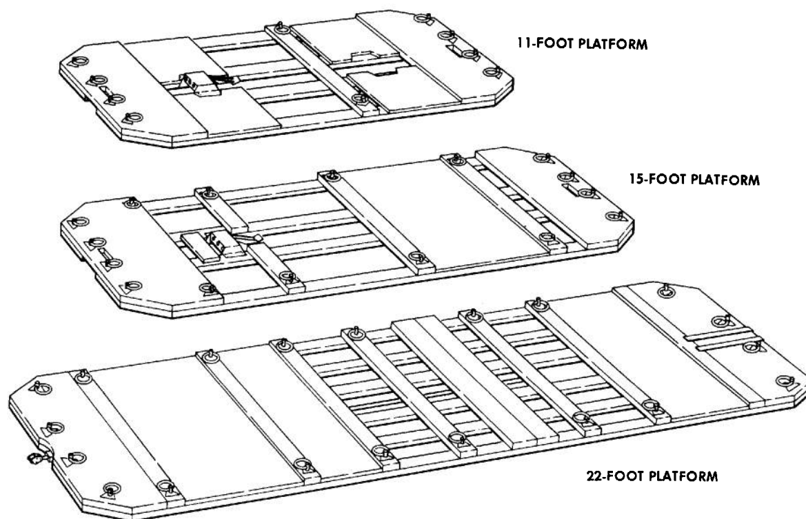
FIGURE 3-60. STANDARD 8 PLATFORMS
