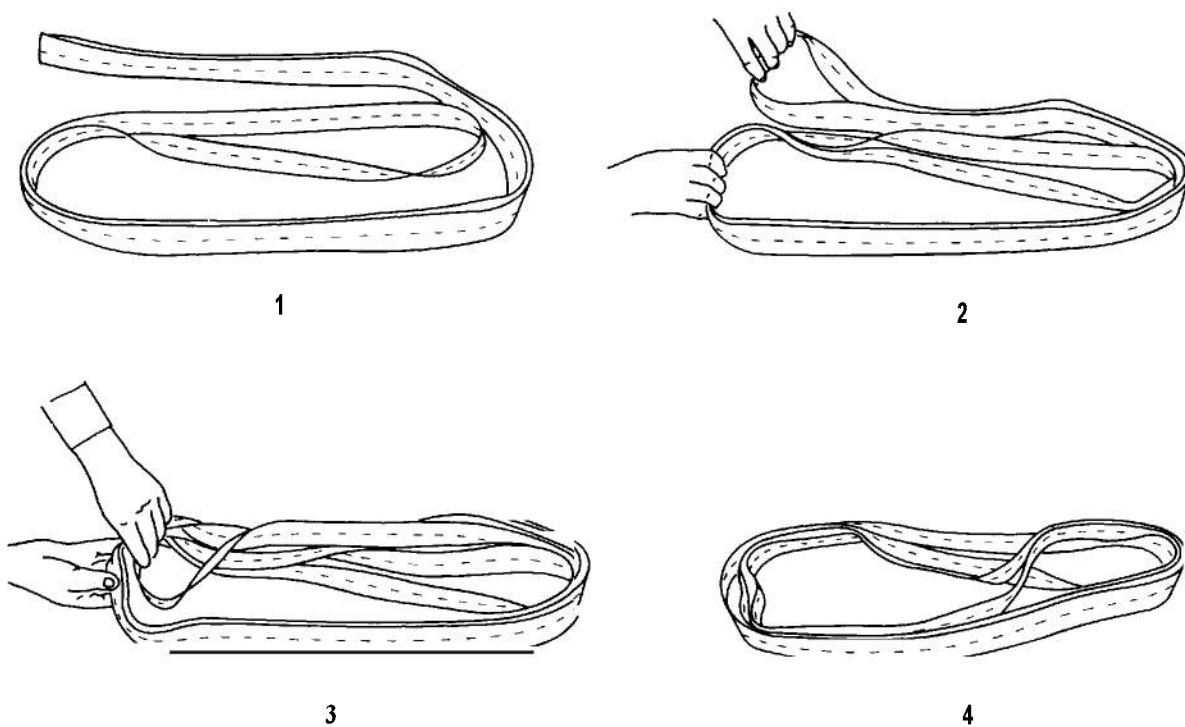
FIGURE 2-37. LAP FOLD
