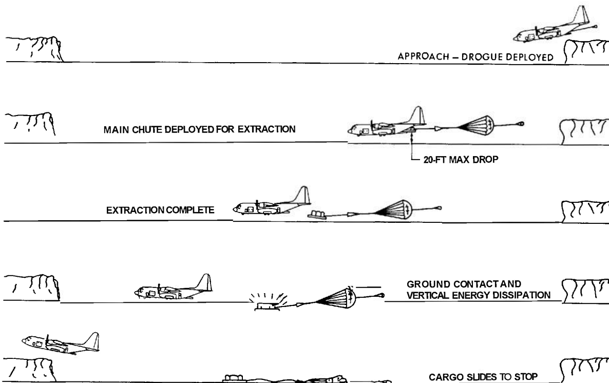
FIGURE 3-10. PARACHUTE DELIVERY SEQUENCE
