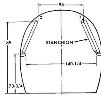
MAXIMUM CLEARANCE OUTLINE AFT OF STATION 340
