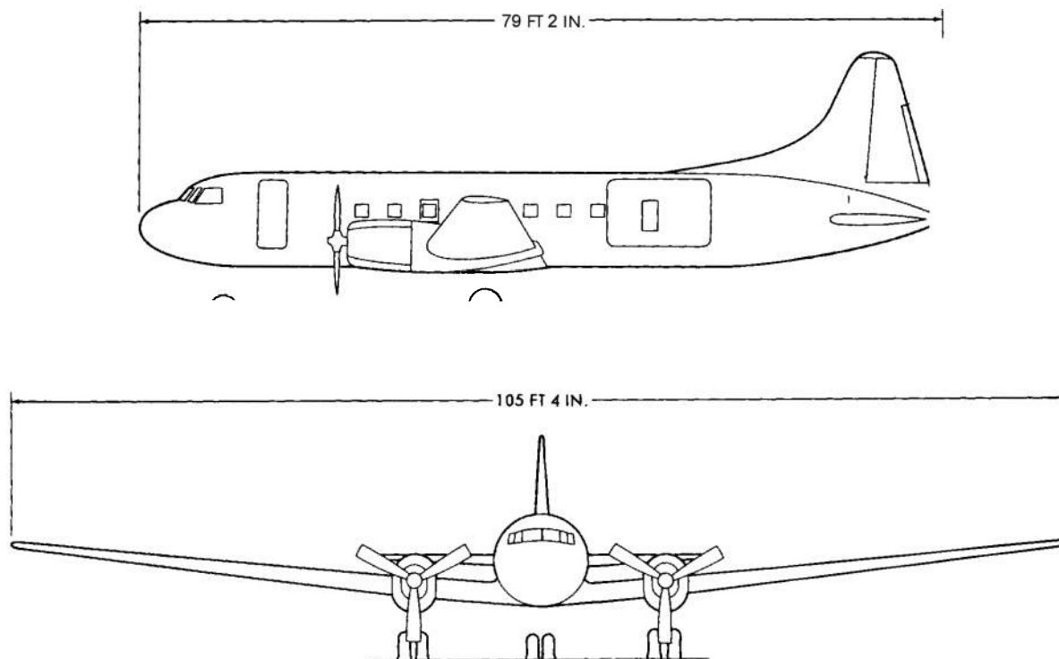
FIGURE 4-66. C-131E AIRCRAFT
