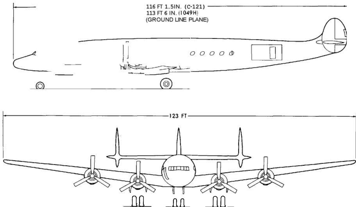
FIGURE 4-38. C-121/1049H AIRCRAFT
