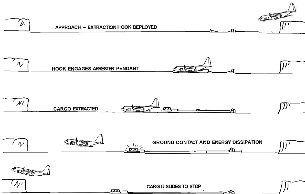
FIGURE 3-9. DELIVERY SEQUENCE WITH GROUND-BASED ENERGY ABSORBER
