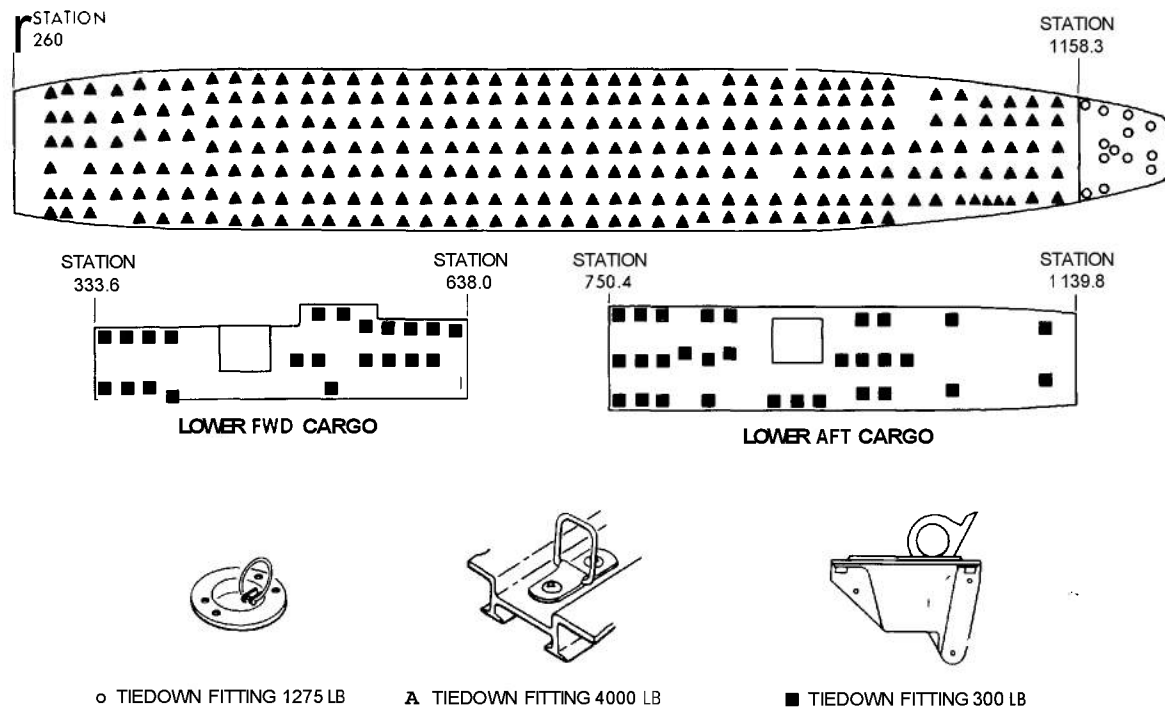
FIGURE 4-41. ANCHORING ARRANGEMENT, C-121/1049H AIRCRAFT
