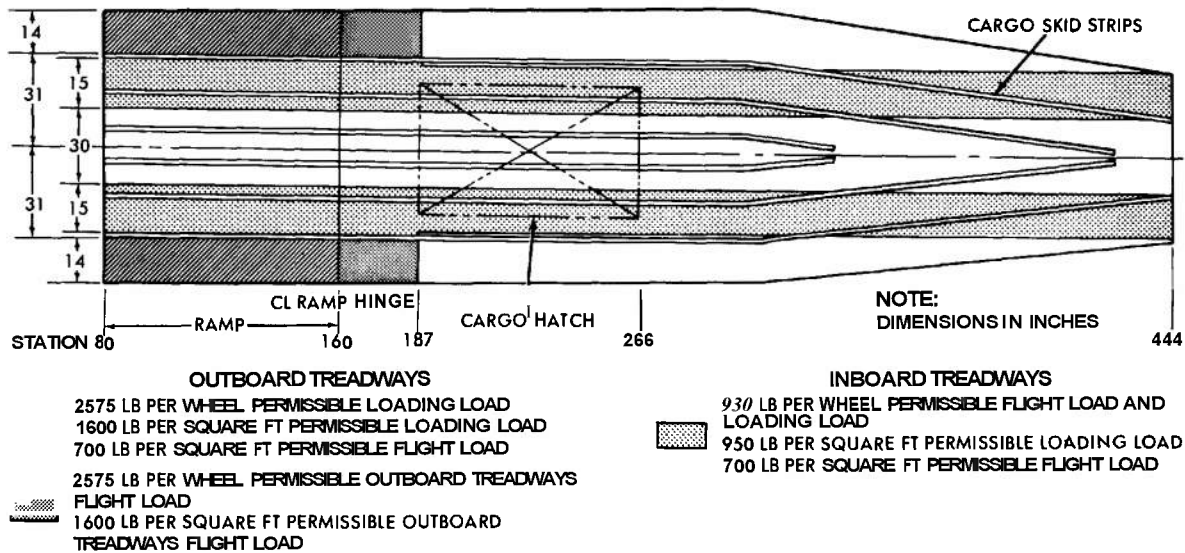
FIGURE 4-121. TREADWAY CAPACITIES, CH-378 HELICOPTER
