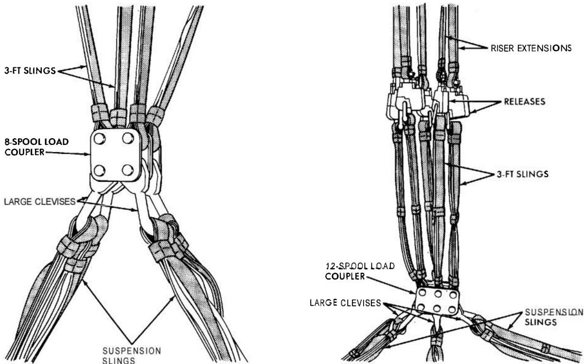
FIGURE 3-43. TYPICAL RELEASE INSTALLATION WITH LOAD COUPLER AND LARGE CLEAVISES
