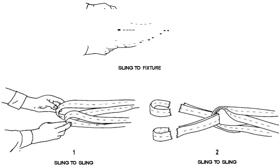
FIGURE 2-34. BASKET HITCH
