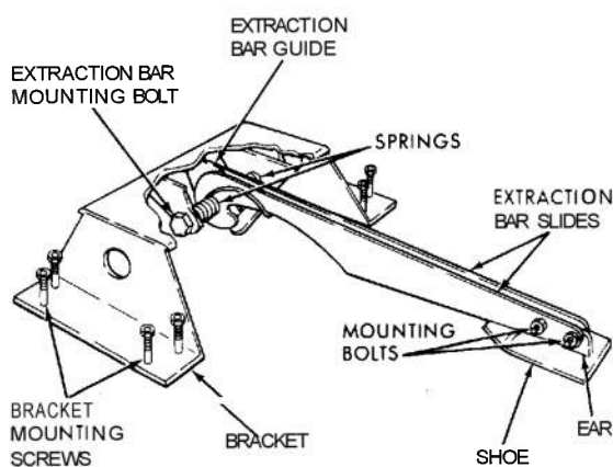
FIGURE 3-46. EXTRACTION BAR ASSEMBLY
