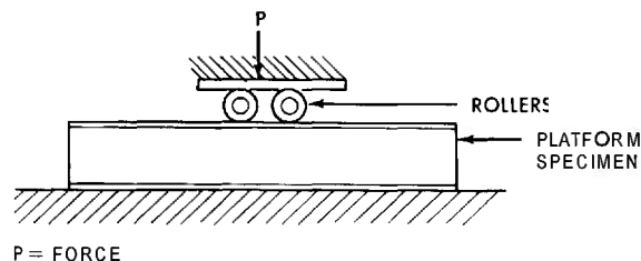
FIGURE 3-64. DESIGN CONDITION FOR GROUND HANDLING
