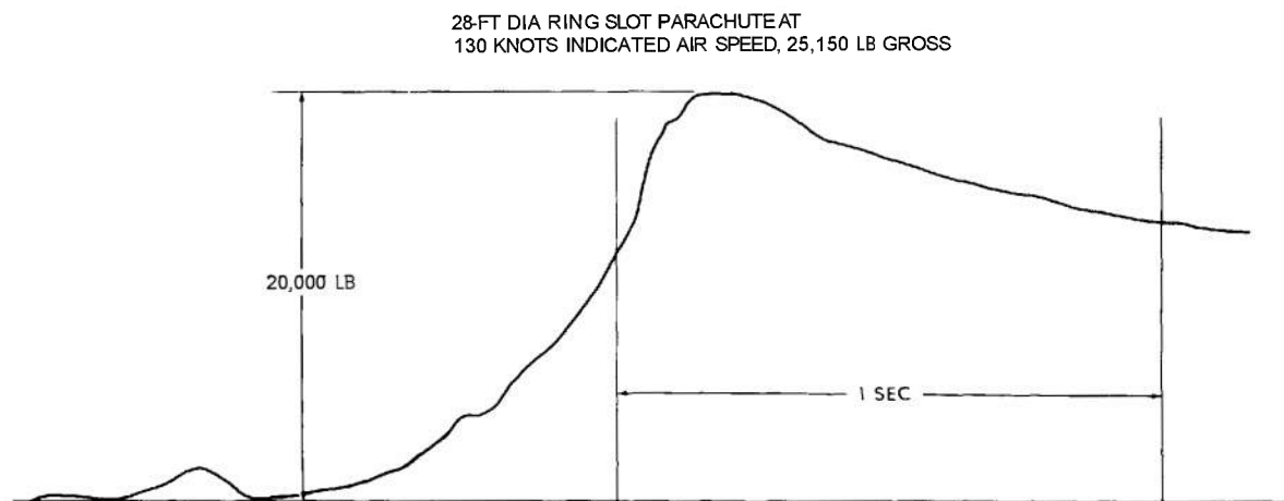
FIGURE 3-65. TYPICAL TRACE OF EXTRACTION FORCE VS TIME
