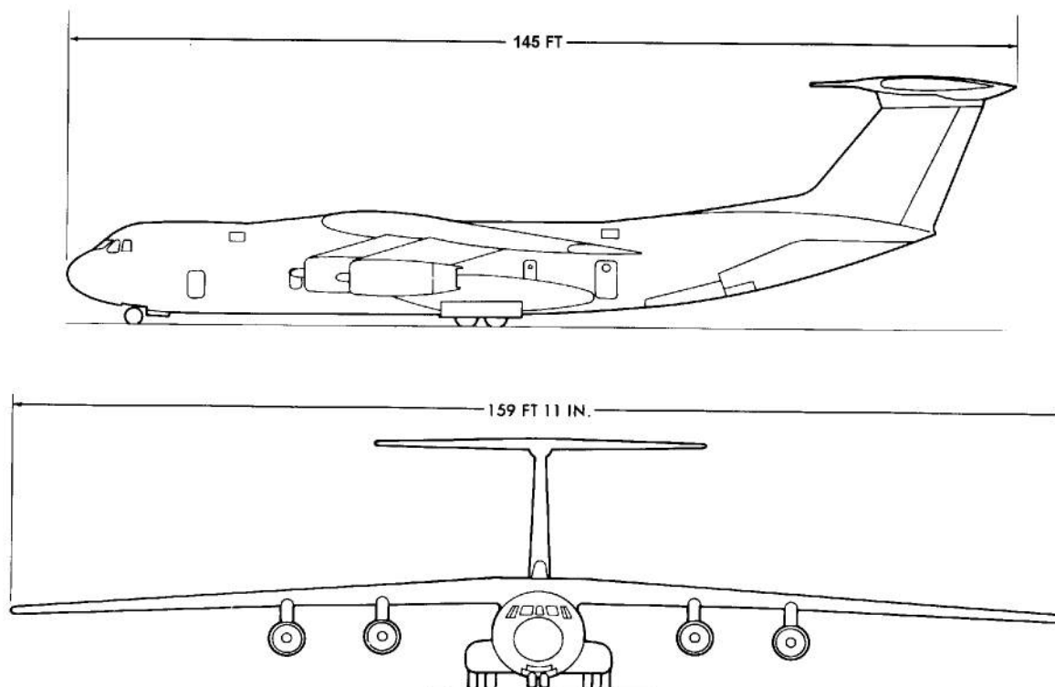
FIGURE 4-84. C-141 AIRCRAFT
