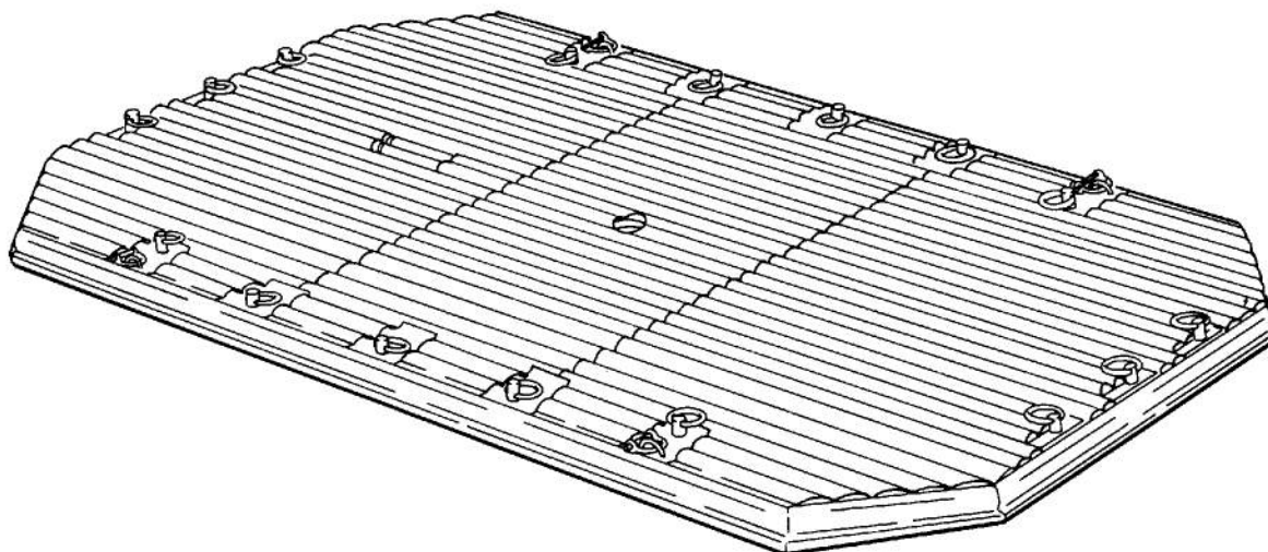
FIGURE 3-59. J-1 PLATFORM
