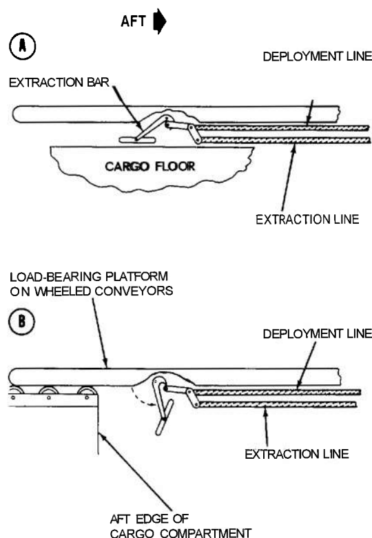
FIGURE 3-47. TYPICAL OPERATION OF EXTRACTION BAR FOR RELEASE AND FORCE TRANSFER
