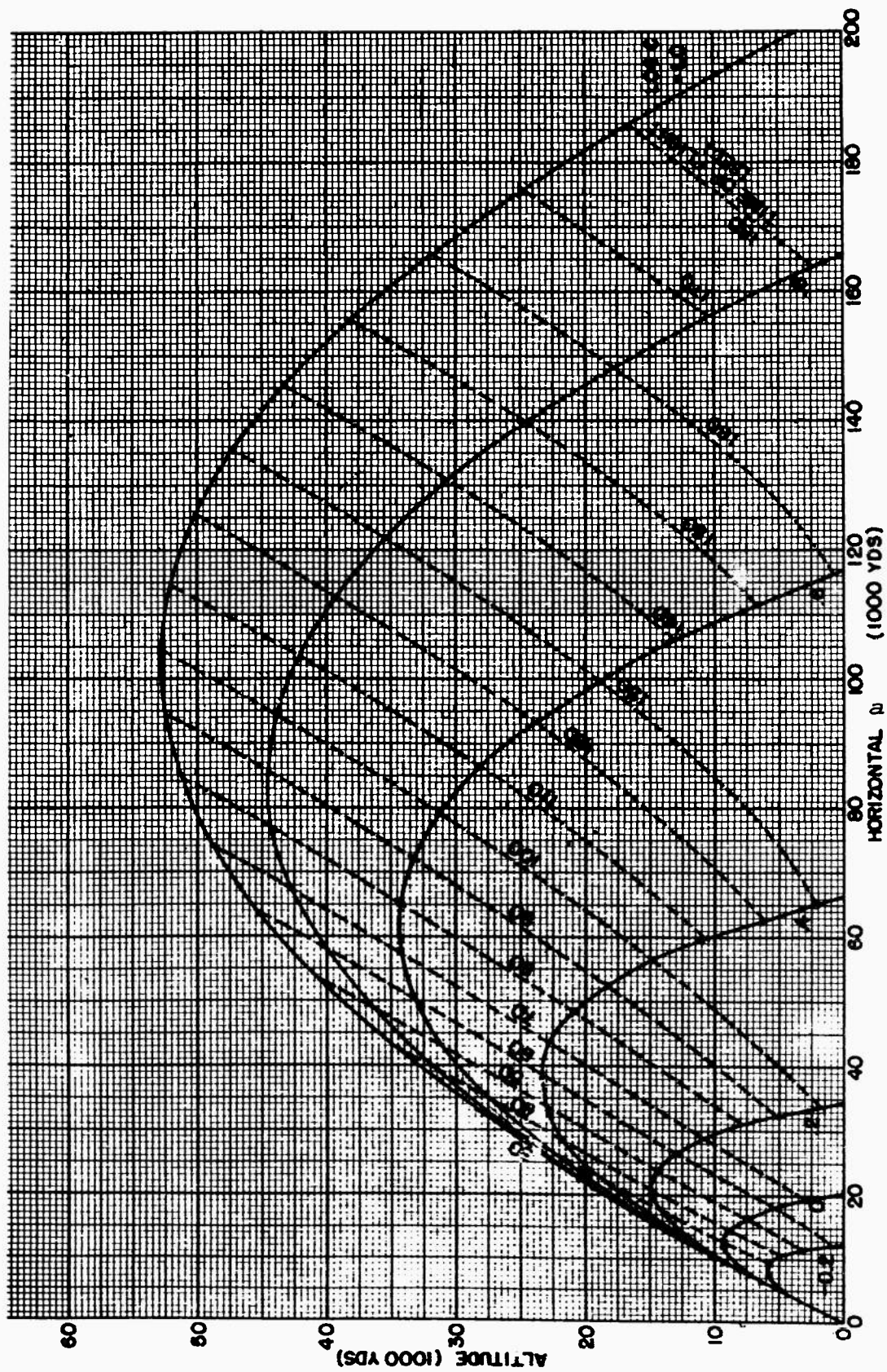
Figure 7 (6 of 12). Trajectories for Projectile Type 8, 45° elevation, 5200 fps muzzle velocity
