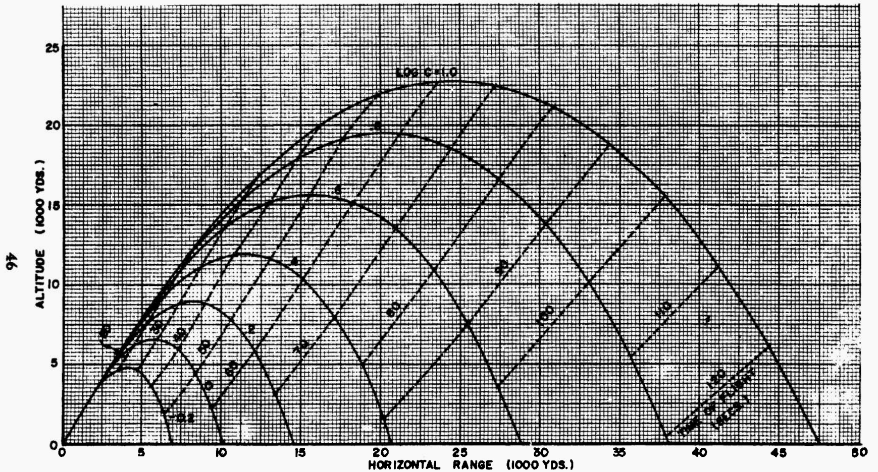
Figure 7 (9 of 12). Trajectories for Projectile Type 8, 60° elevation, 2800 fps muzzle velocity
