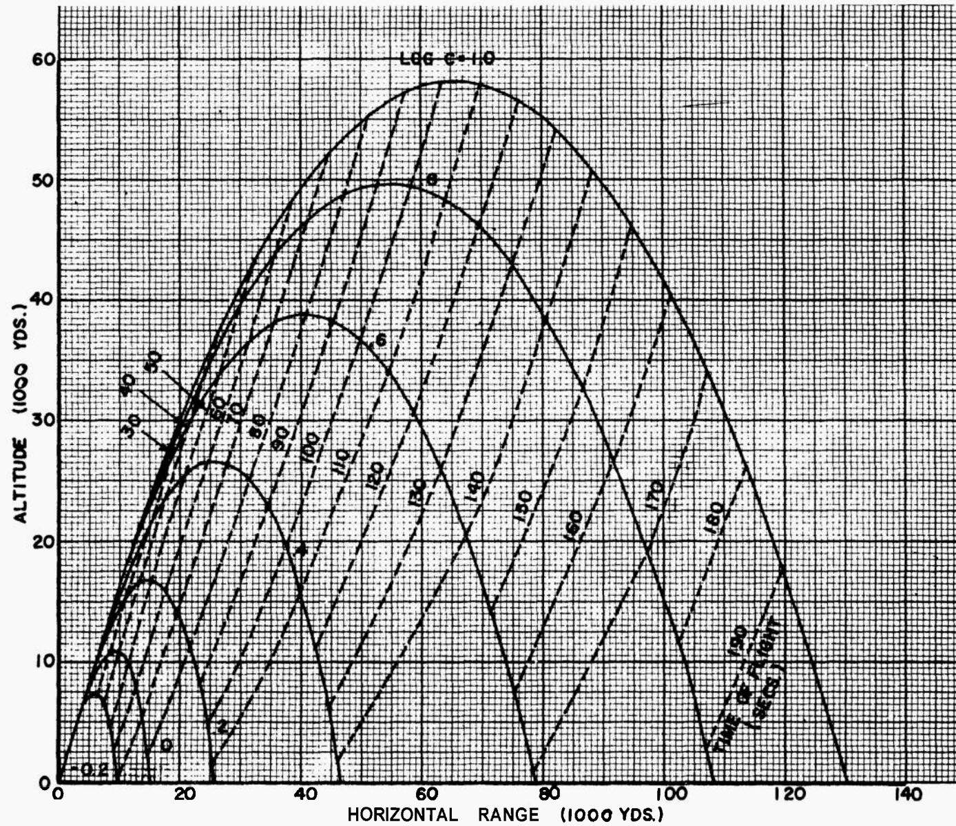
Figure 7 (11 of 12). Trajectories for Projectile Type 8, 60° elevation, 4400 fpe muzzle velocity
