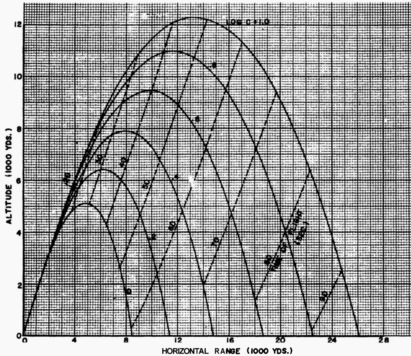
Figure 6 (8 of 12). Trajectories for Projectile Type 2, 60' elevation, 2000 fpe muzzle velocity
