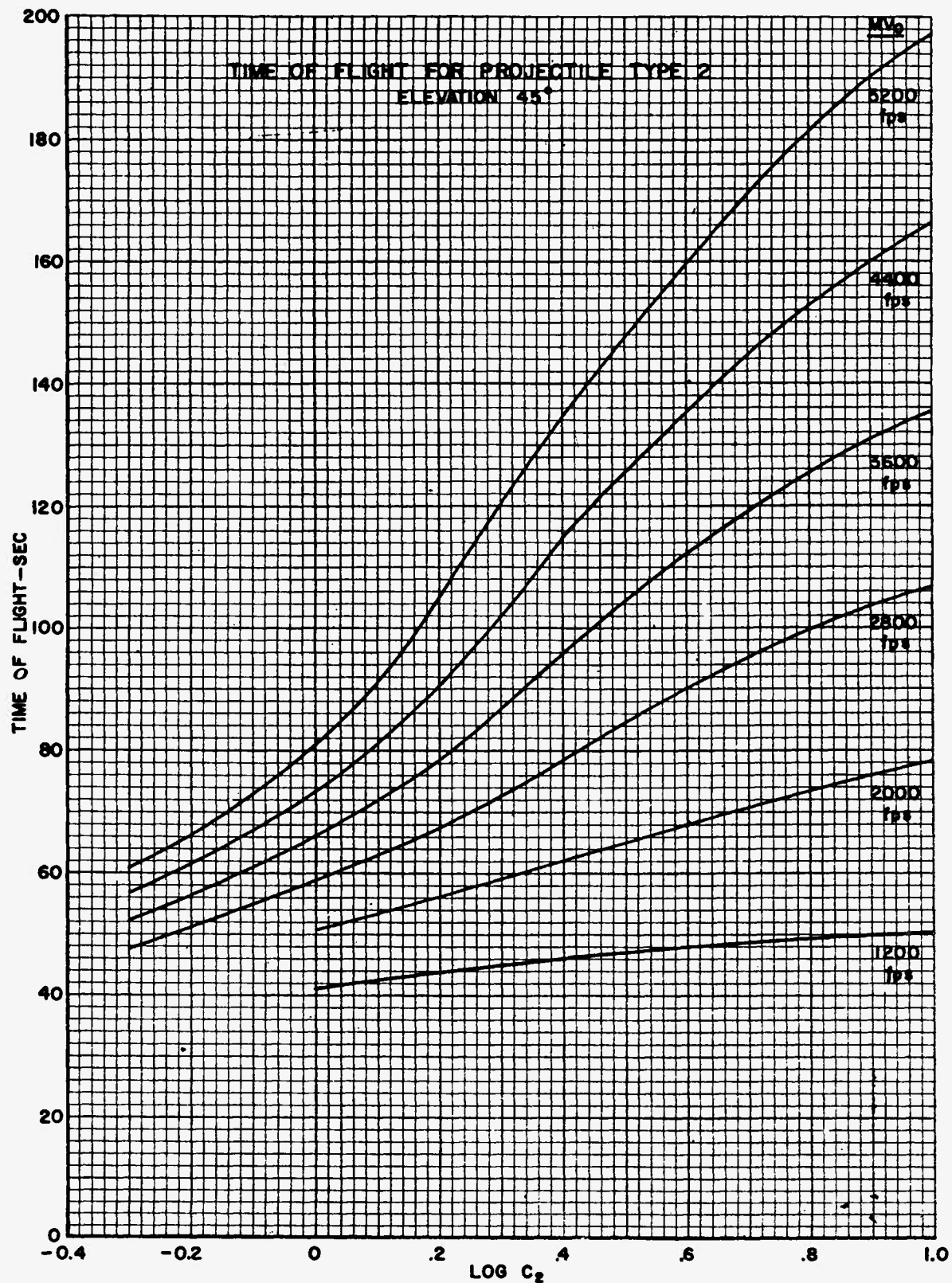
Figure 4. Time of Flight for Projectile Type 2
