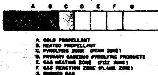
Figure 2. Burning of Solid Monopropellant
