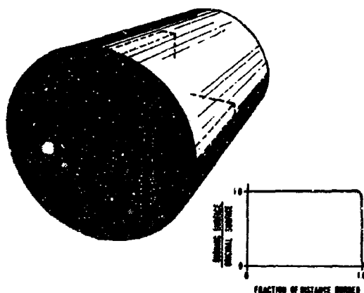
Figure 11. Slotted-Tube Grain
