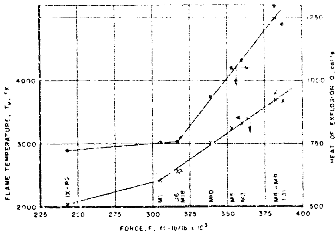
Figure 29. Relationships among T , F , and Q for Gun Propellants
