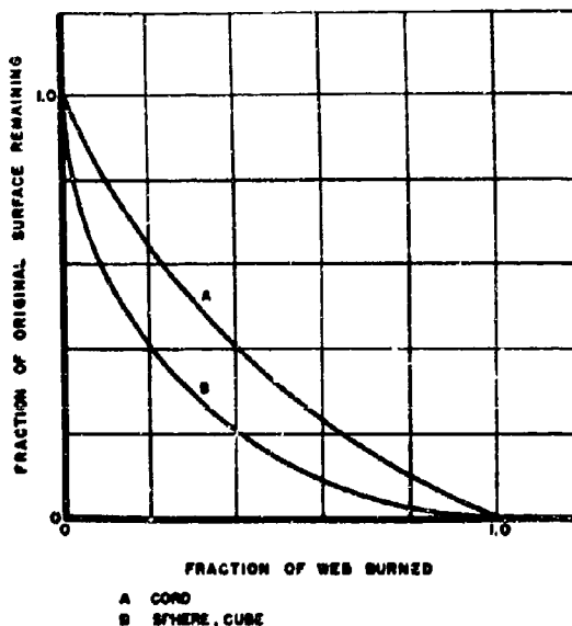
Figure 14. Degressive Geometry
