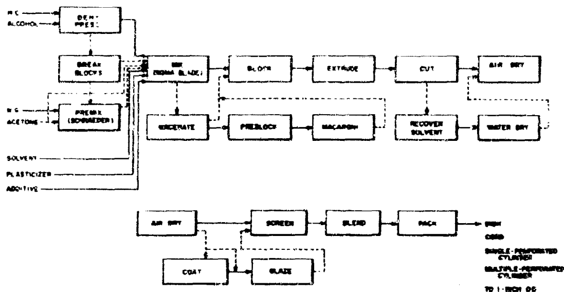
Figure 37. Solvent Extrusion Process
