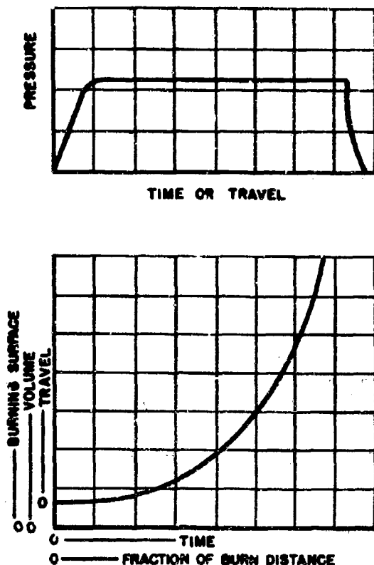
Figure 18. Catapult Cycle
