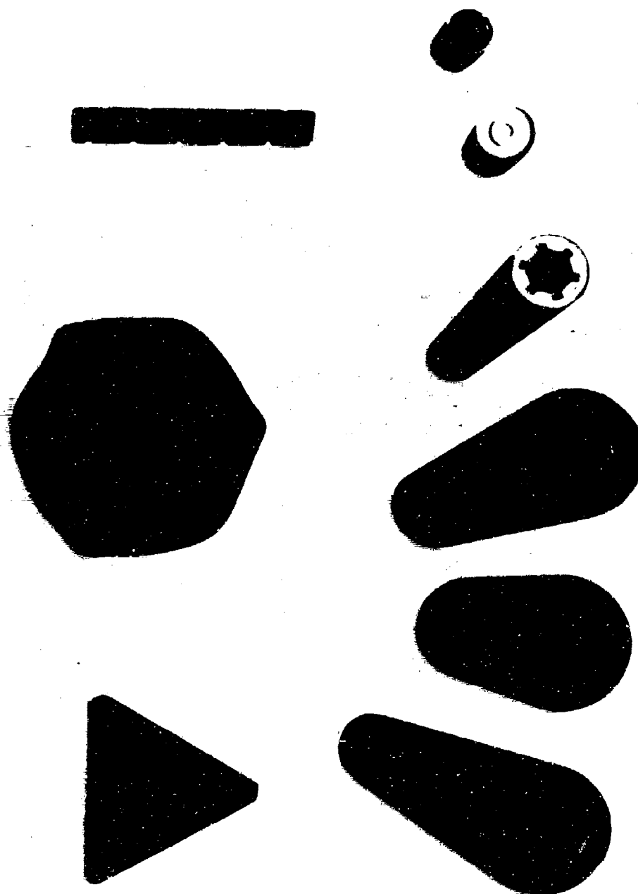
Figure 52. Solvent-extruded Shapes
