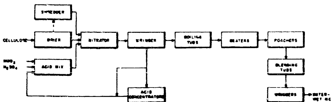
Figure 33. Nitrocellulose Manufacture
