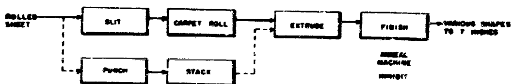
Figure 51. Solventless Extrusion Process
