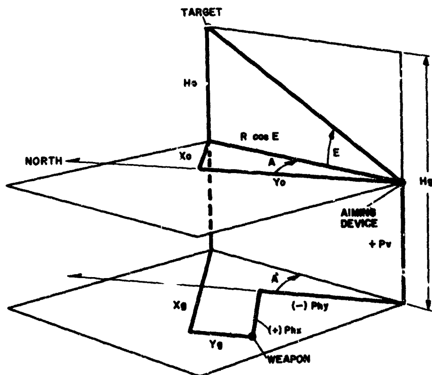
Figure 26. Parallax corrections in rectangular coordinates
