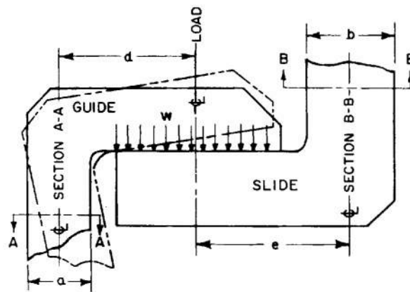
(a) LOADING DIAGRAM
