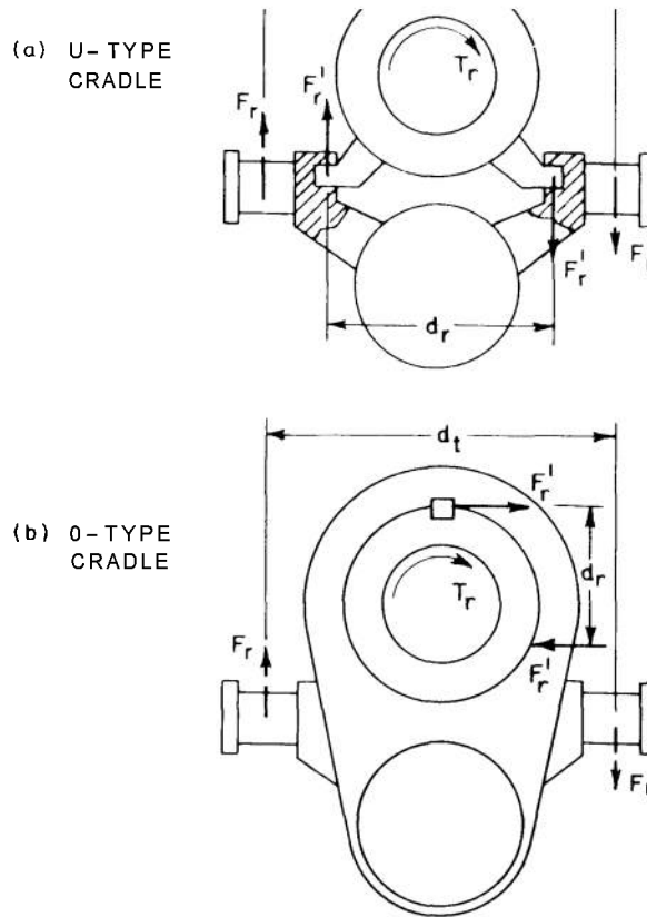
Figure 11. Forces Due to Rifling Torque
