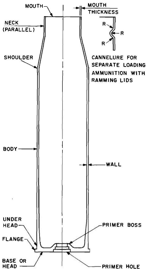
Figure 4-19. Cartridge case
