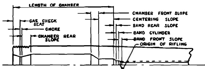
FIGURE B SOME LARGE CALIBER GUNS
