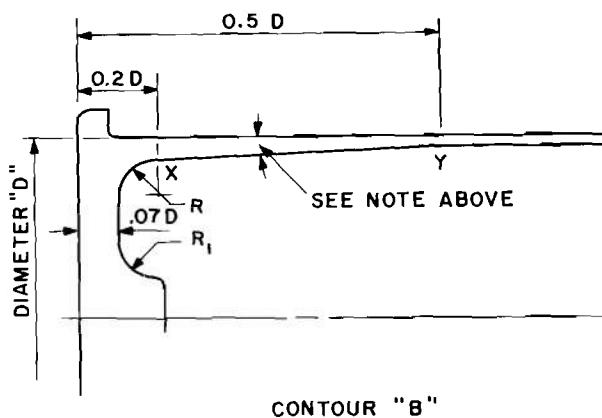
Figure 4-25. Internal contour of cartridge cases
