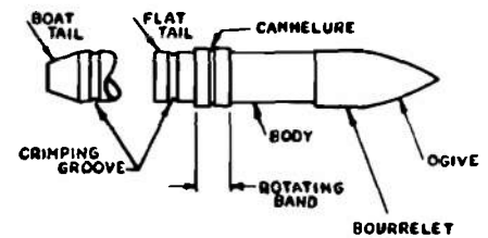
FIGURE I ARTILLERY TYPE PROJECTILE
