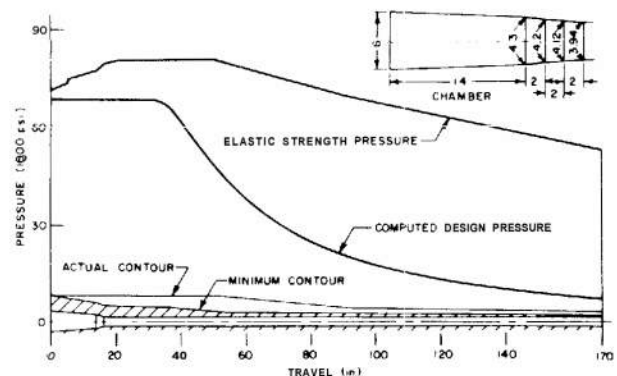
FIGURE 61. Design Data, Monobloc Artillery Tube.
