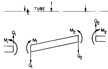
FIGURE 44. Conical Section Loading.
