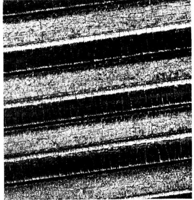
FIGURE 10. Thermal Cracks on Bare Surface.
