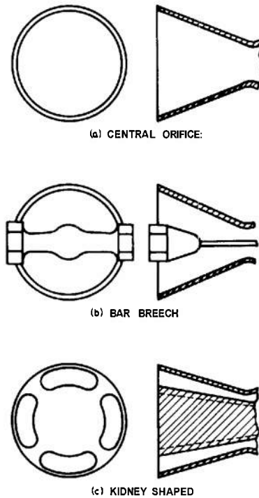
FIGURE 24. Nozzle Shapes-Schematic.
