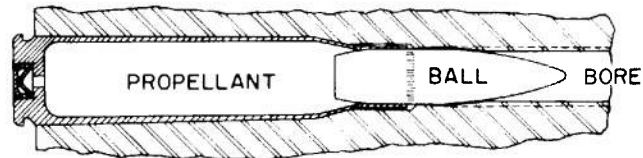
(b) SMALL ARMS CHAMBER CONTAINING FIXED ROUND
