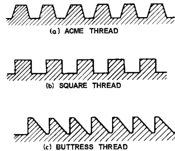
FIGURE 50. Thread Profile Types.
