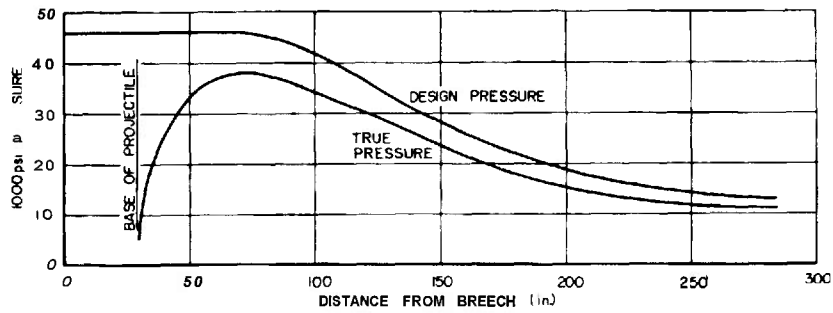
FIGURE 41. Design Pressure-Travel Curve.
