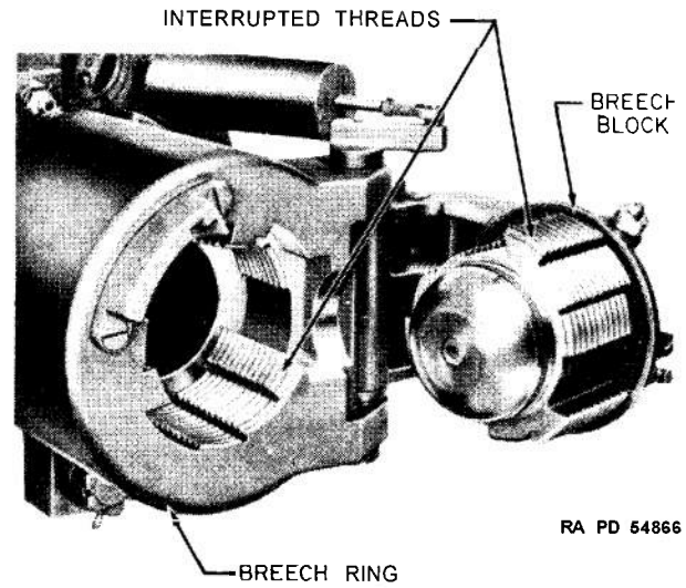
FIGURE 51. Interrupted Threads.
