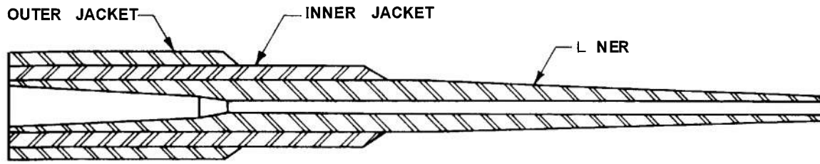
FIGURE 3. Jacketed Tube.
