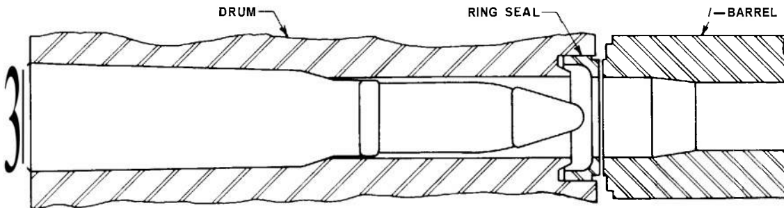
FIGURE 5. Revolver Type Tube Showing Separate Chamber With Round.
