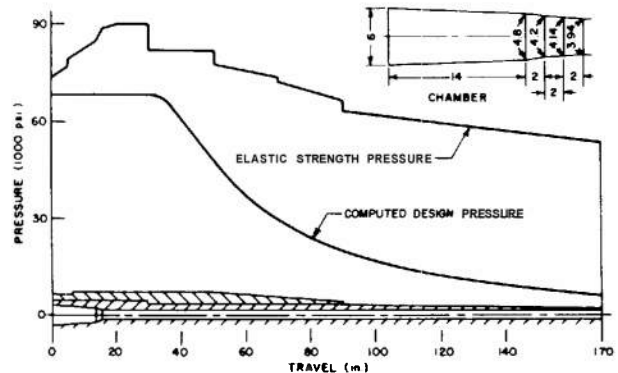
FIGURE 62. Design Data, Jacketed Artillery Tube.
