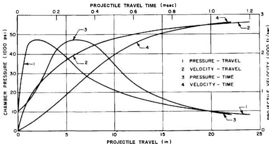
FIGURE 16. Interior Ballistics of Caliber .30 Gun.
